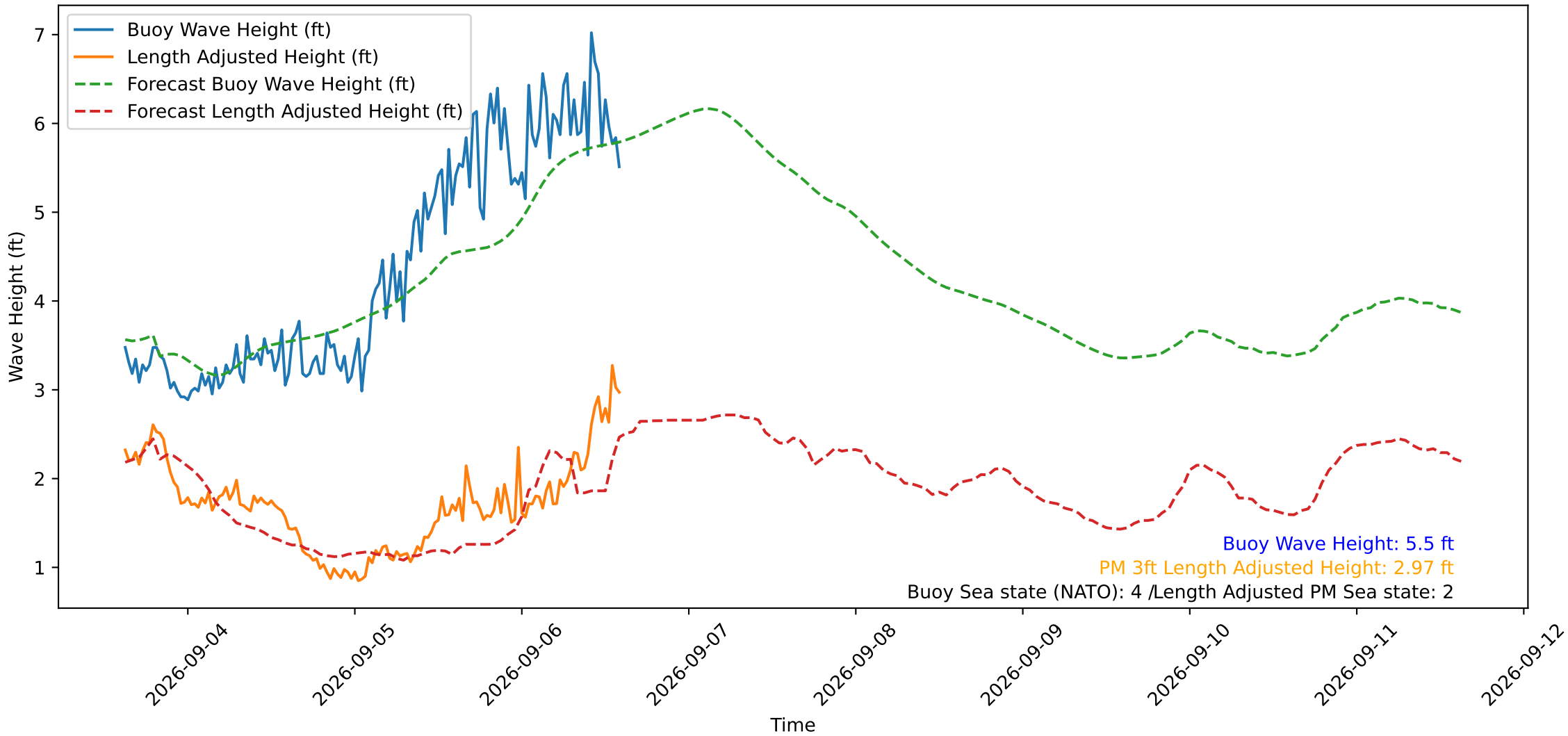
Wave Heights over Time for Oceanside Harbor at 2026-09-06 15:00:30
