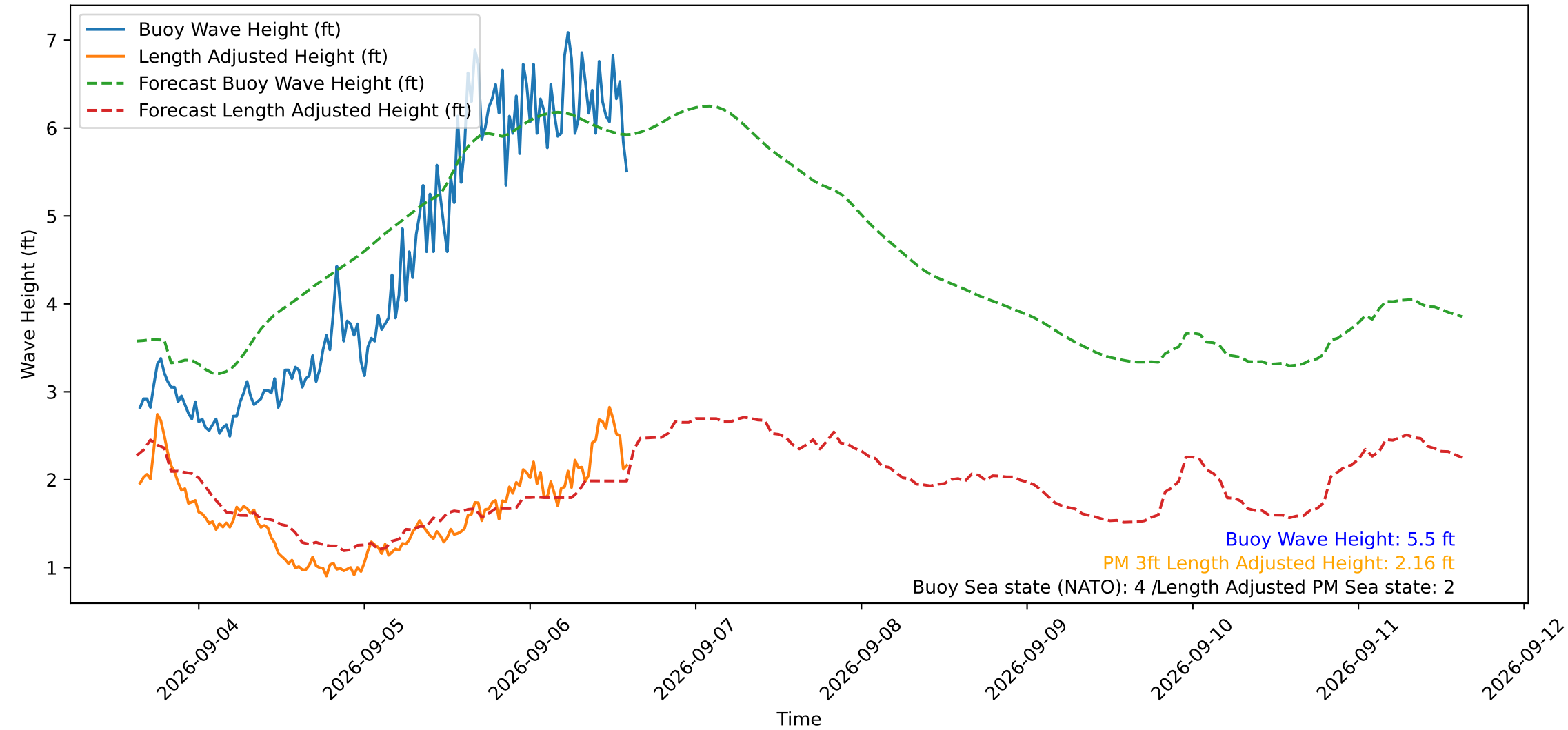
Wave Heights over Time for Green Beach at 2026-09-06 15:01:12
