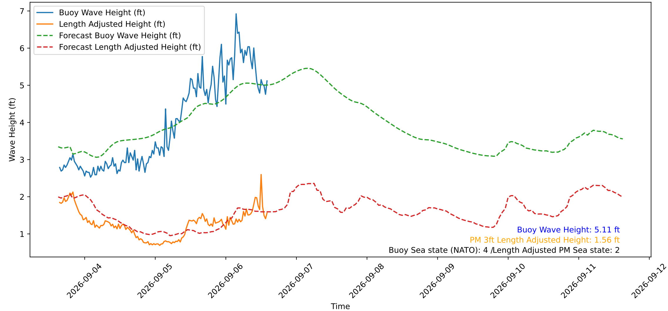
Wave Heights over Time for Red Beach at 2026-09-06 15:00:50
