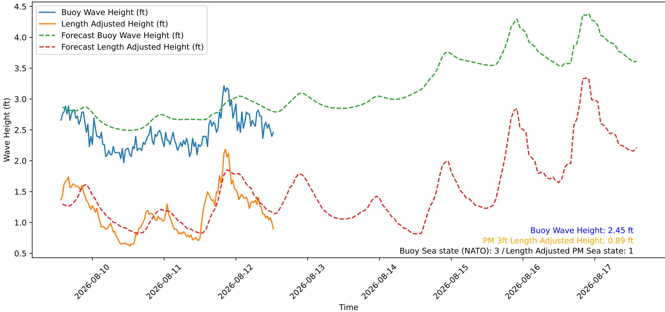
Wave Heights over Time for Green Beach at 2026-08-12 13:31:09
