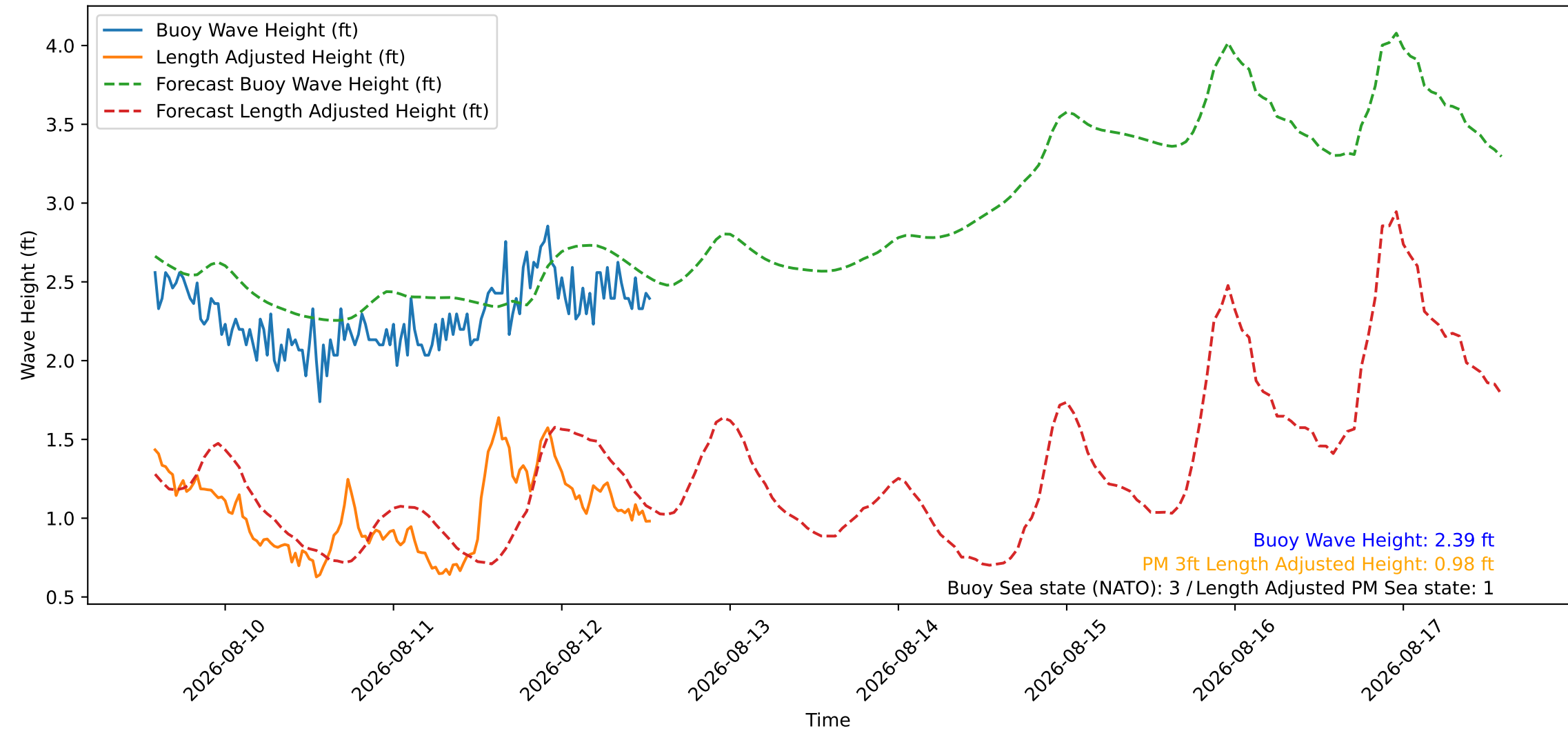
Wave Heights over Time for Red Beach at 2026-08-12 13:30:46
