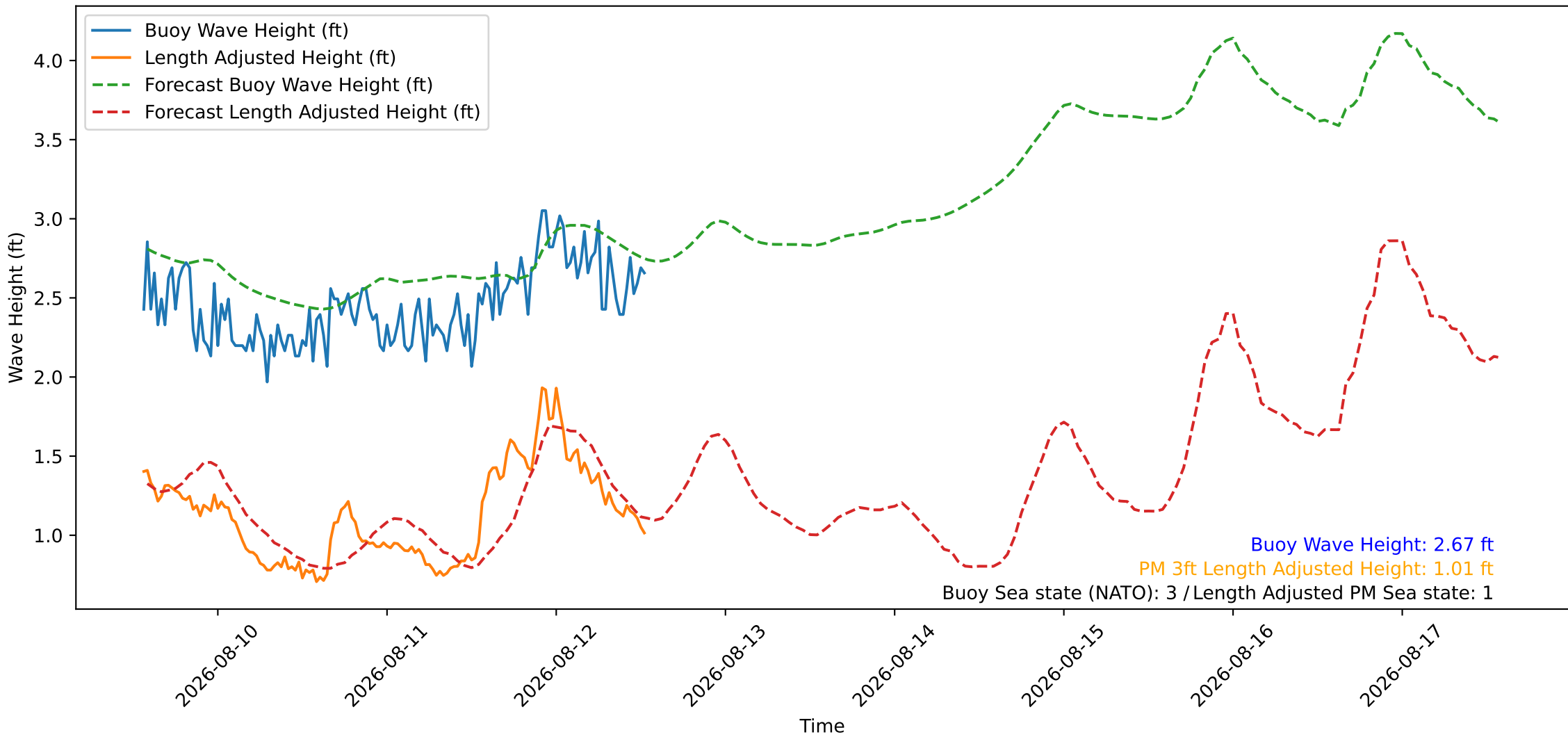
Wave Heights over Time for Oceanside Harbor at 2026-08-12 13:30:27
