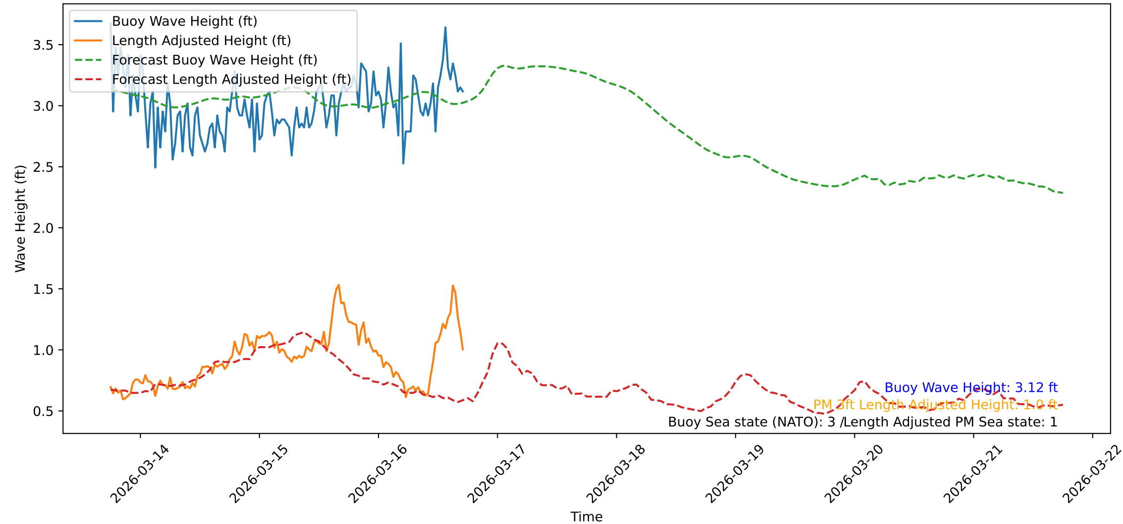
Wave Heights over Time for Red Beach at 2026-03-16 17:51:03
