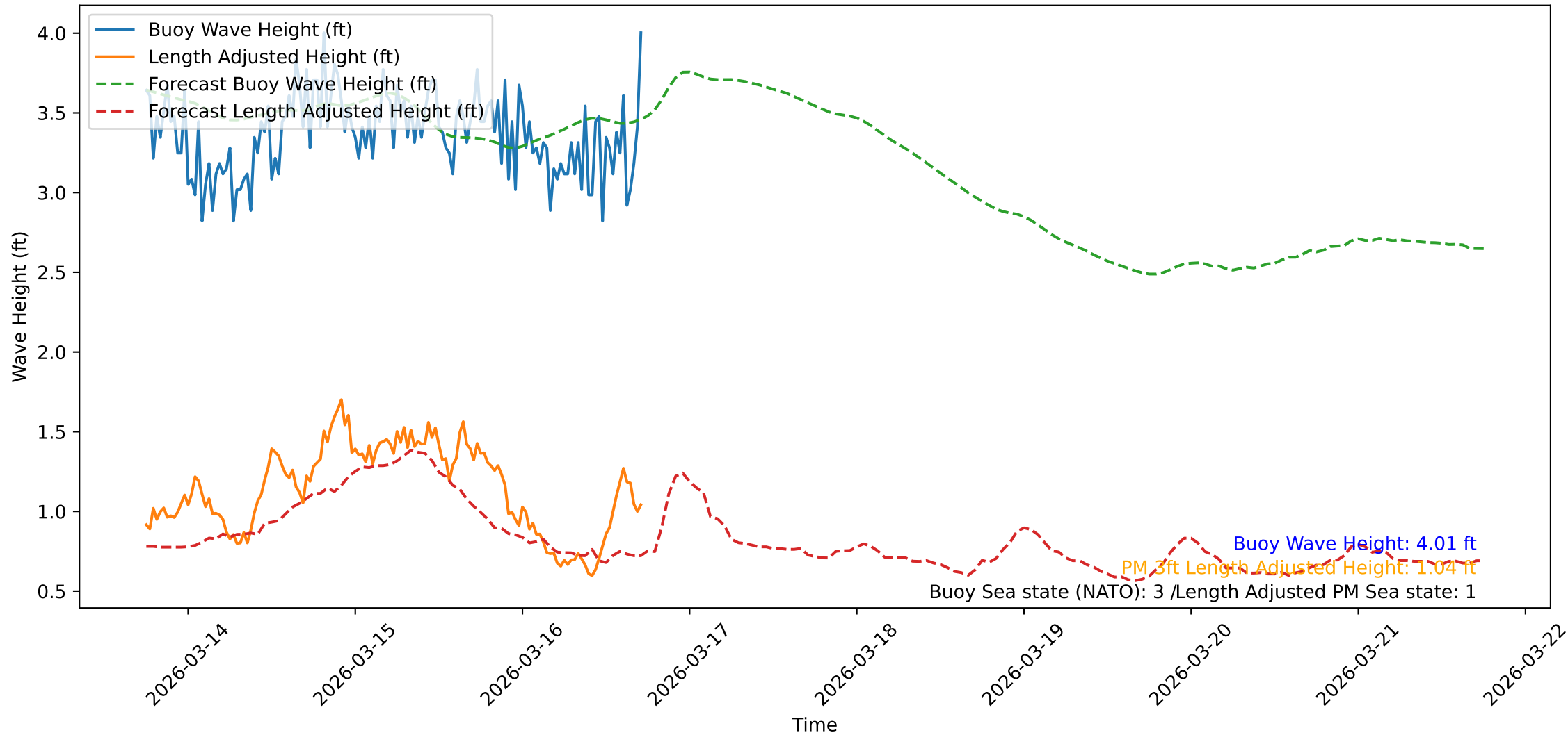
Wave Heights over Time for Green Beach at 2026-03-16 17:51:37
