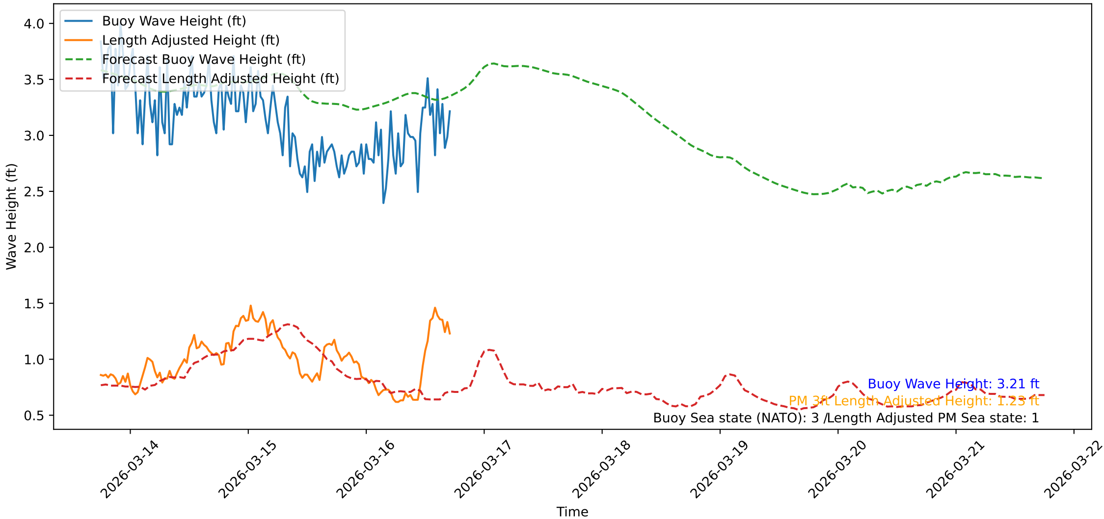
Wave Heights over Time for Oceanside Harbor at 2026-03-16 17:50:41
