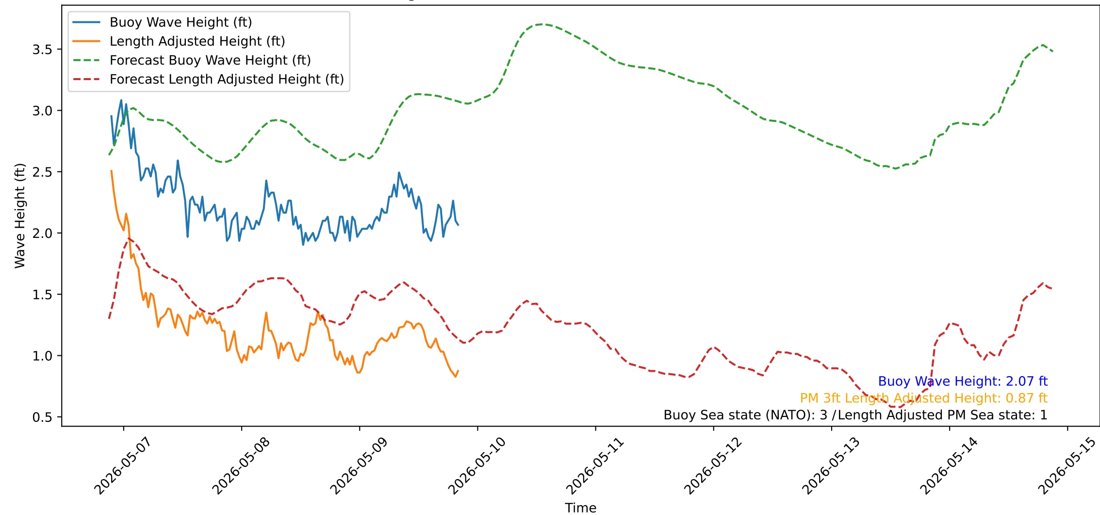
Wave Heights over Time for Red Beach at 2026-05-09 21:10:50
