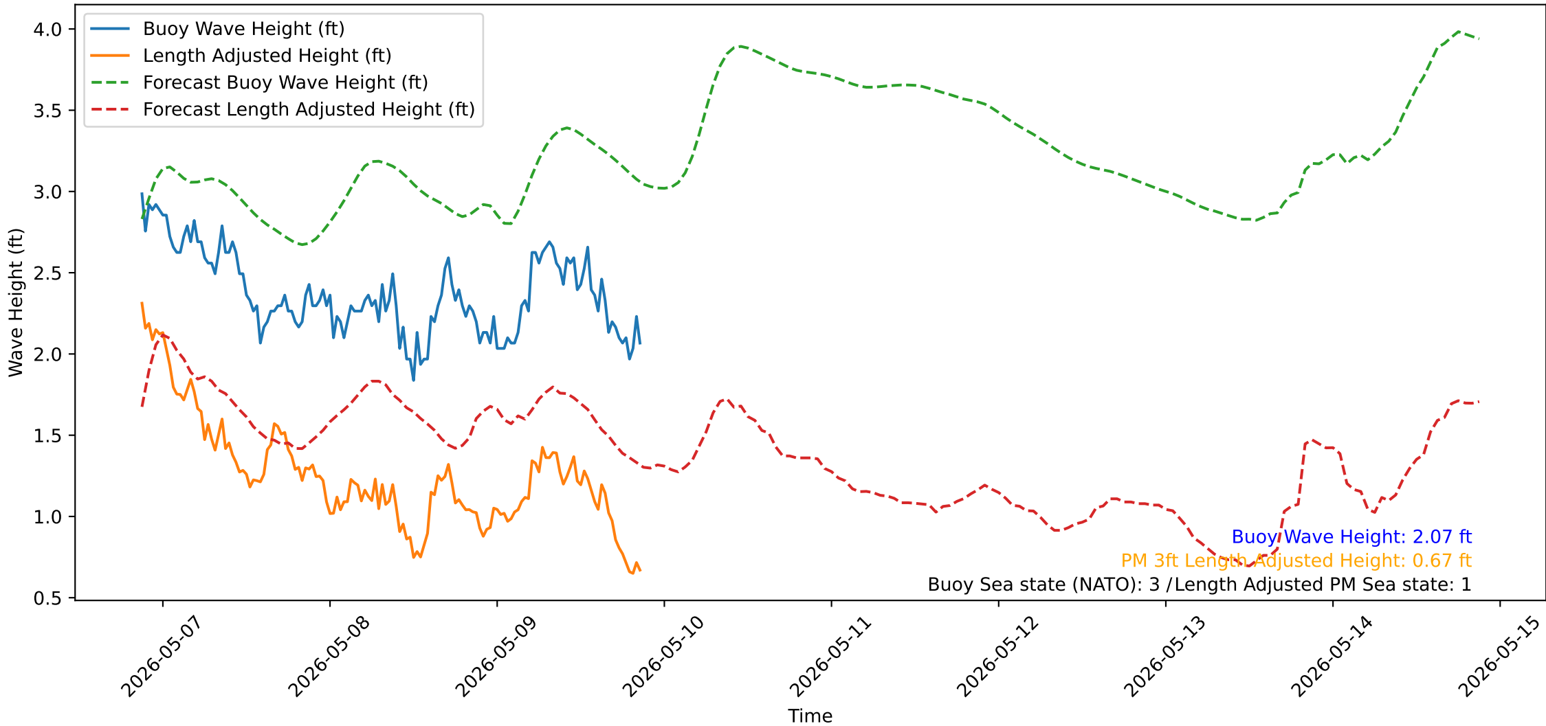
Wave Heights over Time for Green Beach at 2026-05-09 21:11:13
