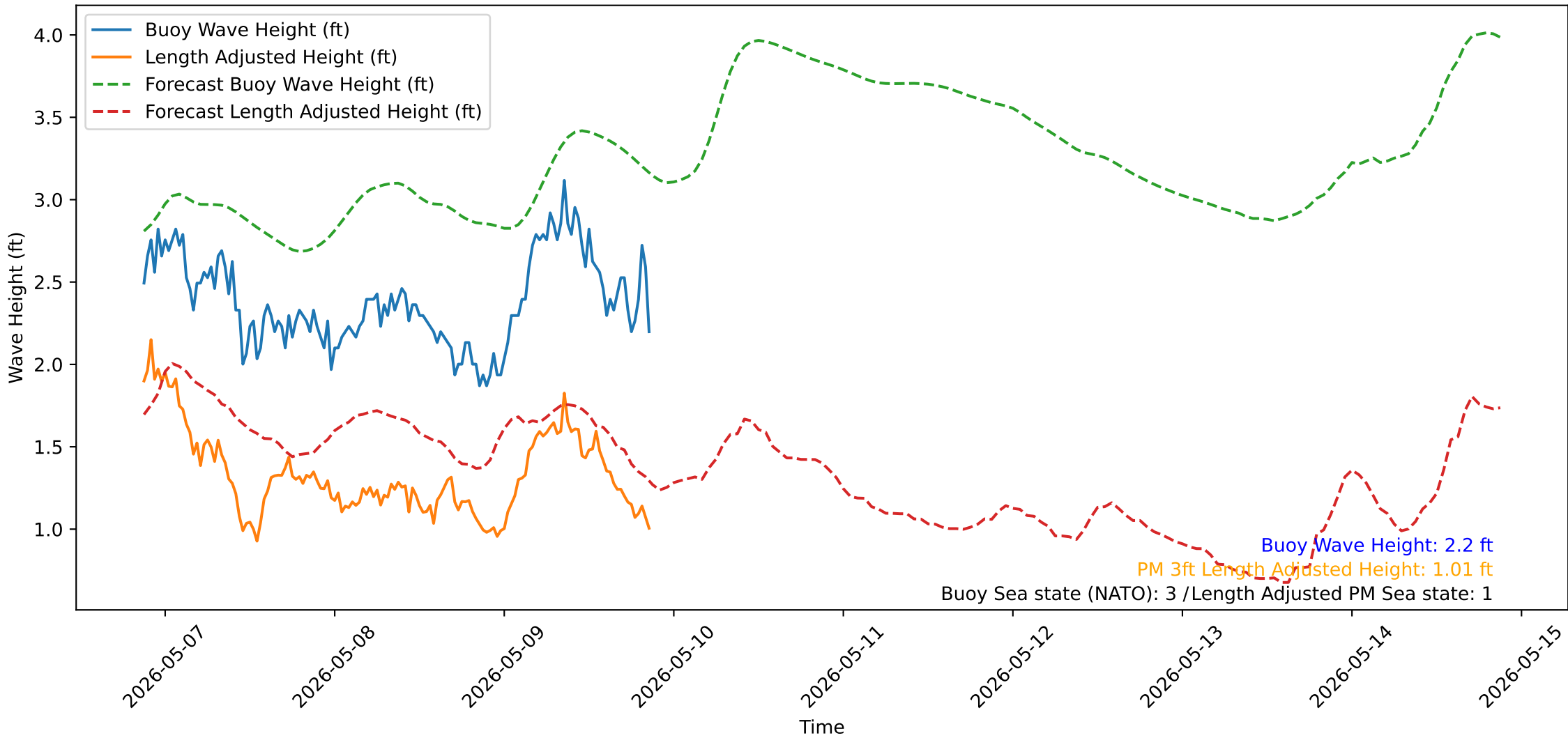
Wave Heights over Time for Oceanside Harbor at 2026-05-09 21:10:31
