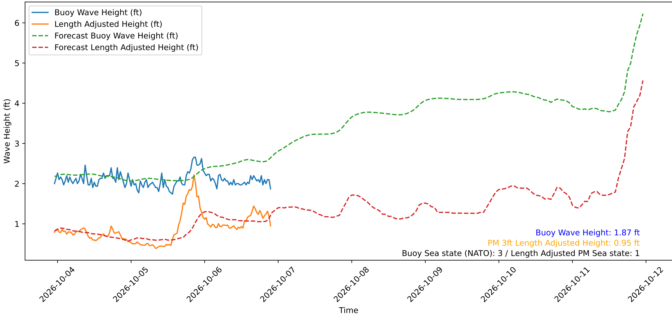
Wave Heights over Time for Red Beach at 2026-10-06 22:30:50
