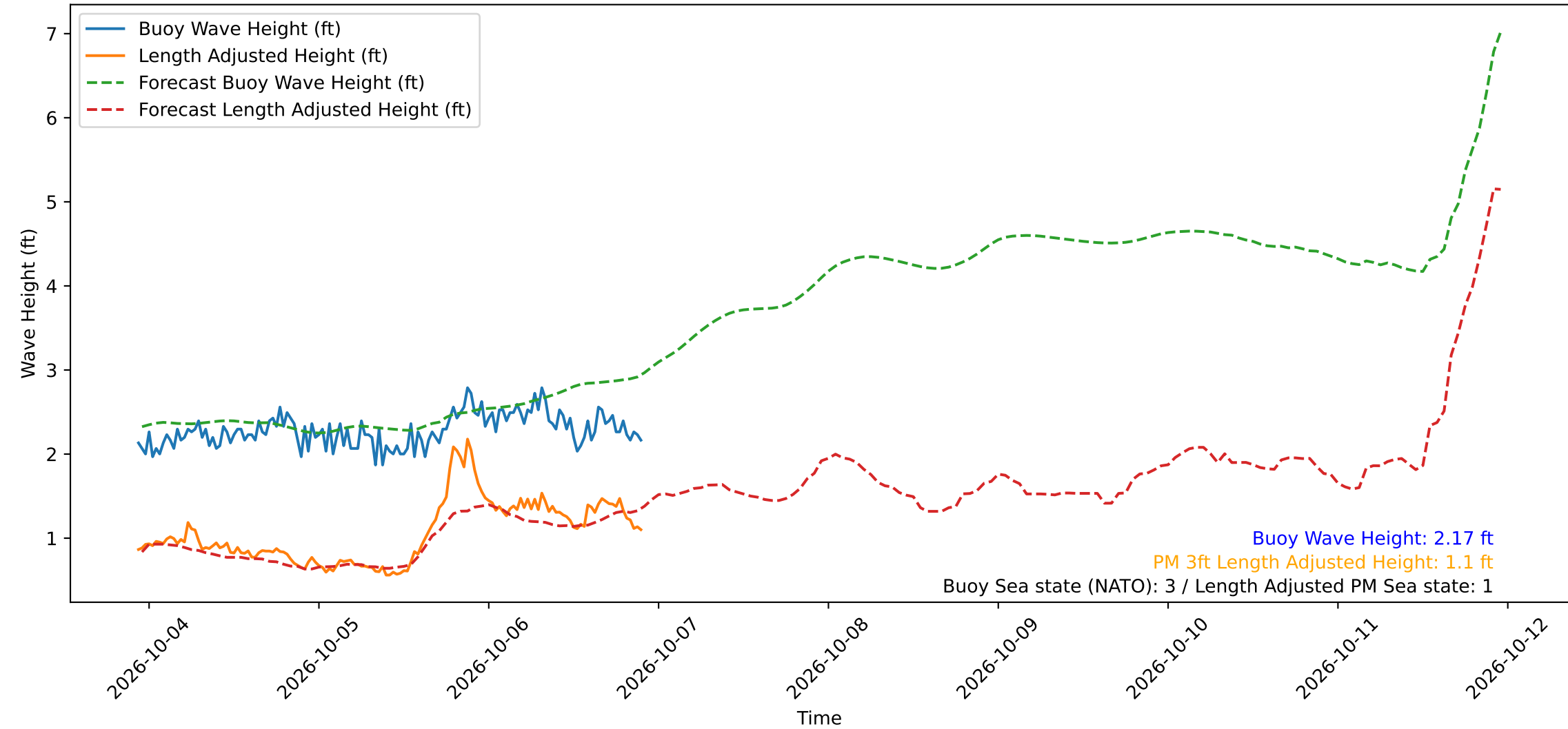
Wave Heights over Time for Oceanside Harbor at 2026-10-06 22:30:30
