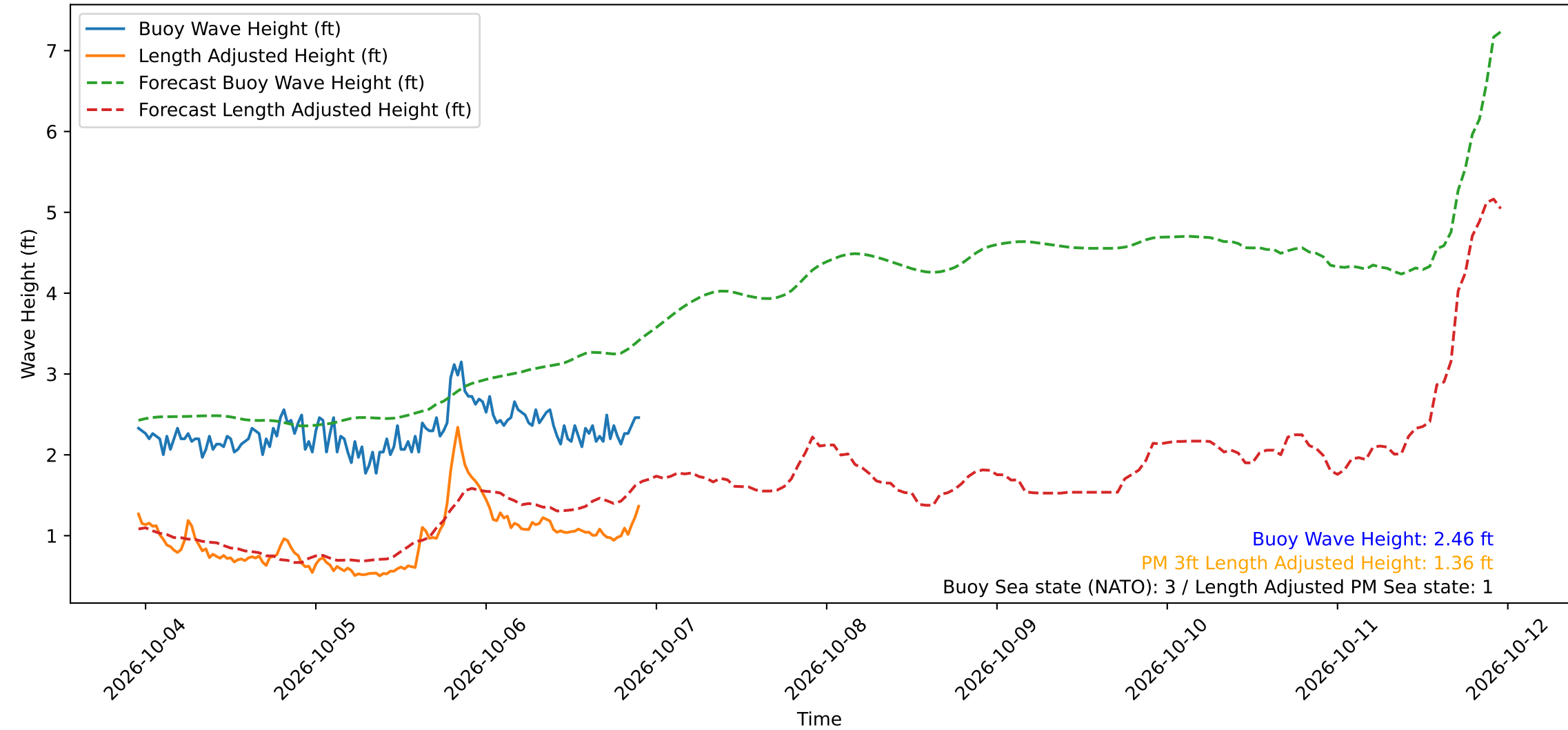
Wave Heights over Time for Green Beach at 2026-10-06 22:31:13
