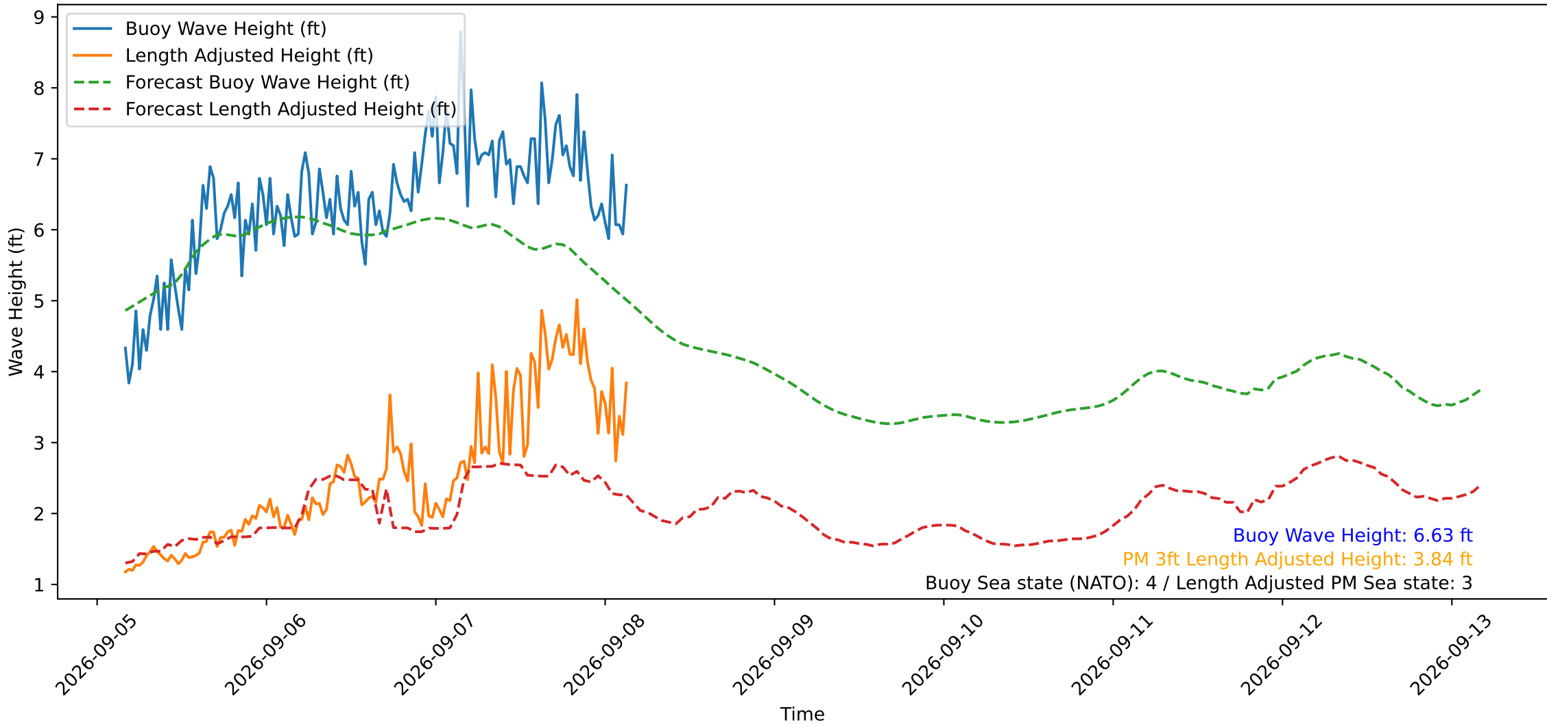
Wave Heights over Time for Green Beach at 2026-09-08 03:41:12
