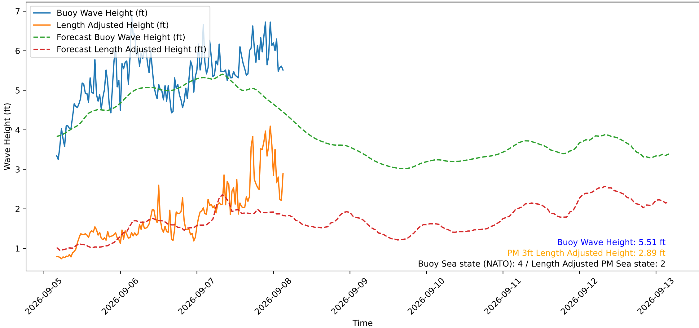
Wave Heights over Time for Red Beach at 2026-09-08 03:40:50
