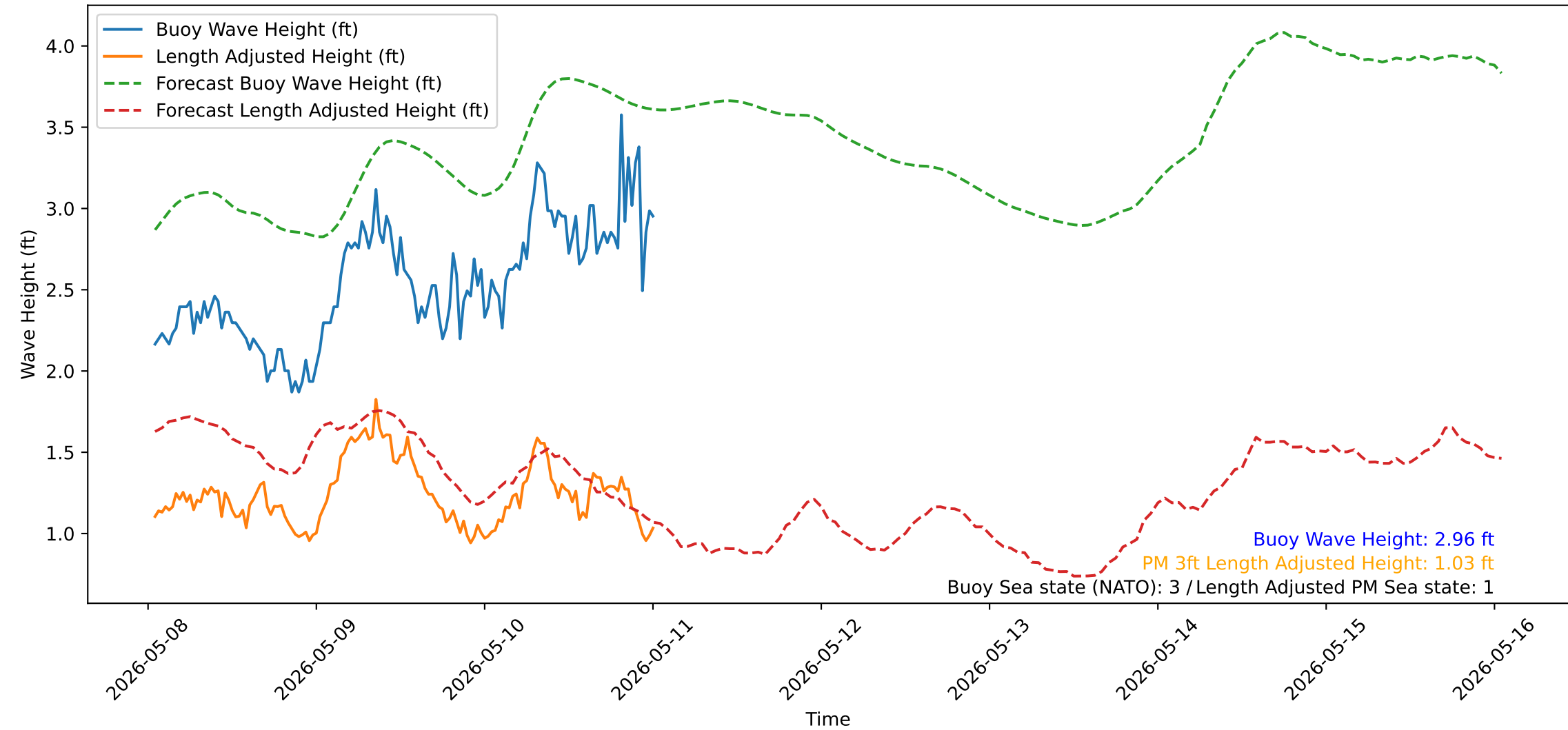
Wave Heights over Time for Oceanside Harbor at 2026-05-11 00:50:31
