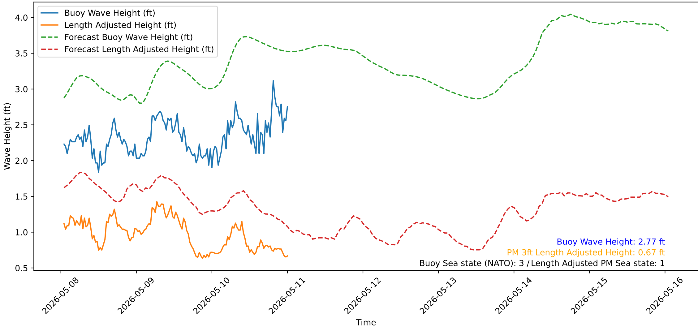
Wave Heights over Time for Green Beach at 2026-05-11 00:51:13
