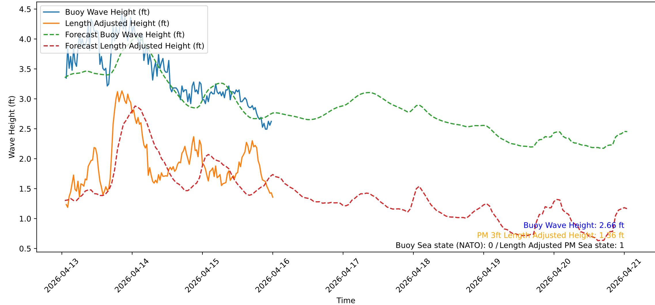
Wave Heights over Time for Red Beach at 2026-04-16 01:00:51
