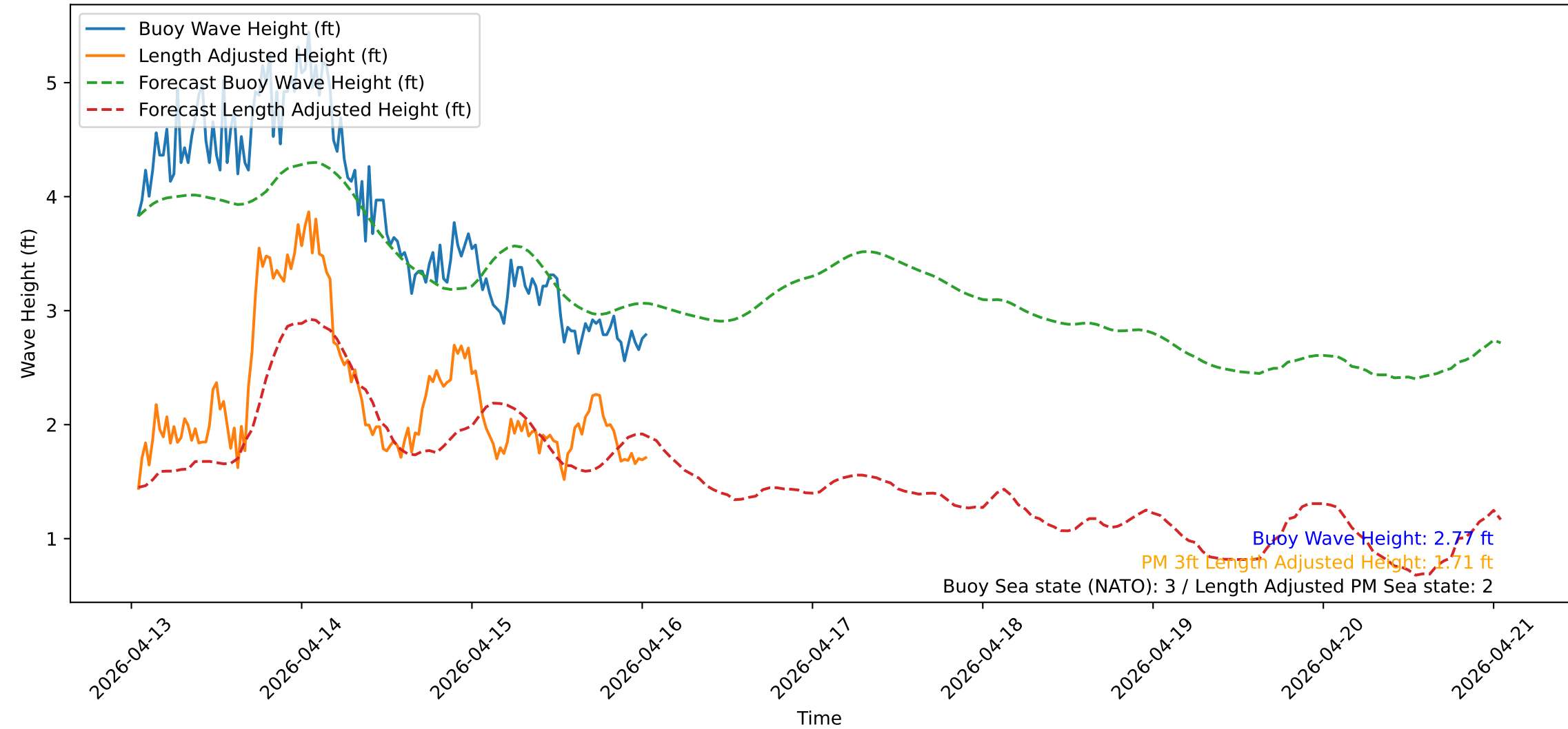
Wave Heights over Time for Oceanside Harbor at 2026-04-16 01:00:32
