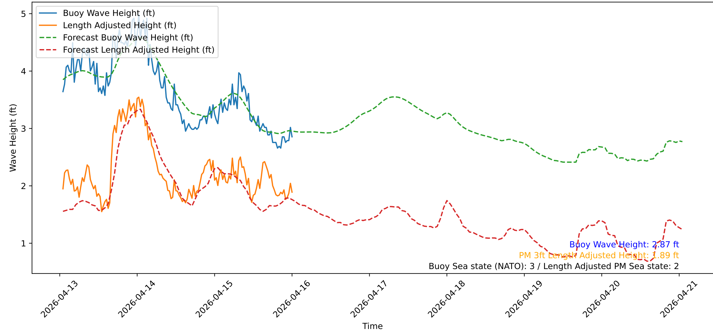
Wave Heights over Time for Green Beach at 2026-04-16 01:01:13
