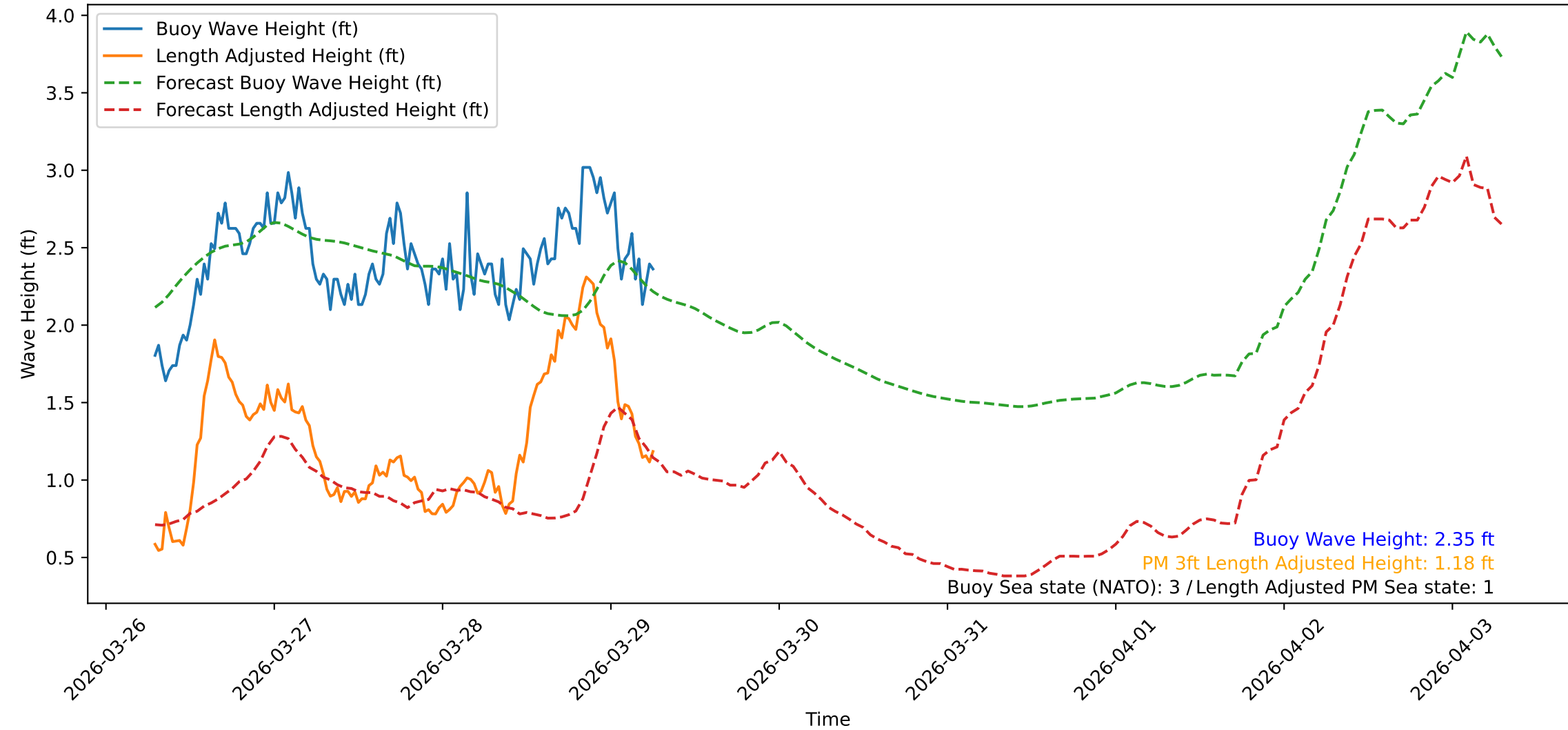
Wave Heights over Time for Red Beach at 2026-03-29 06:50:47
