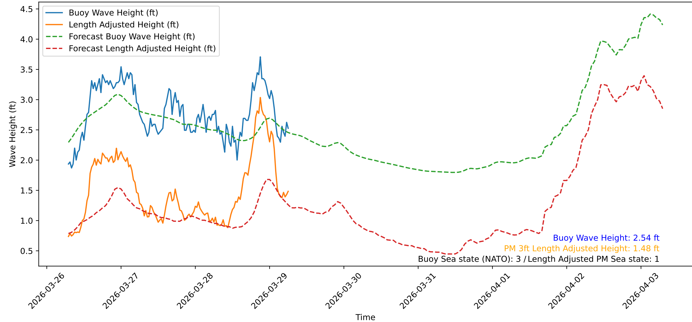
Wave Heights over Time for Green Beach at 2026-03-29 06:51:09
