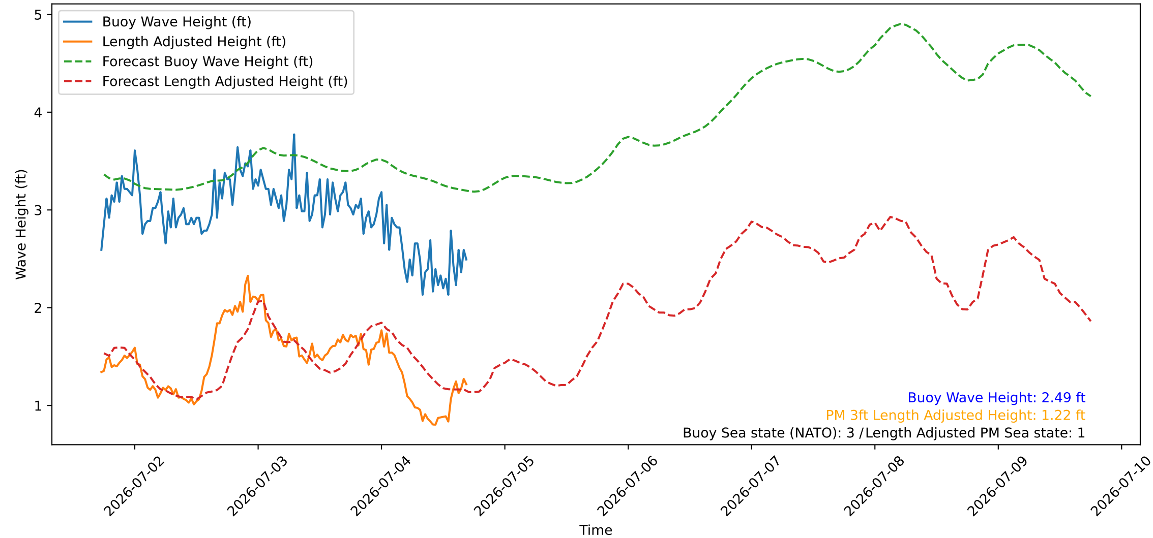
Wave Heights over Time for Oceanside Harbor at 2026-07-04 17:30:26
