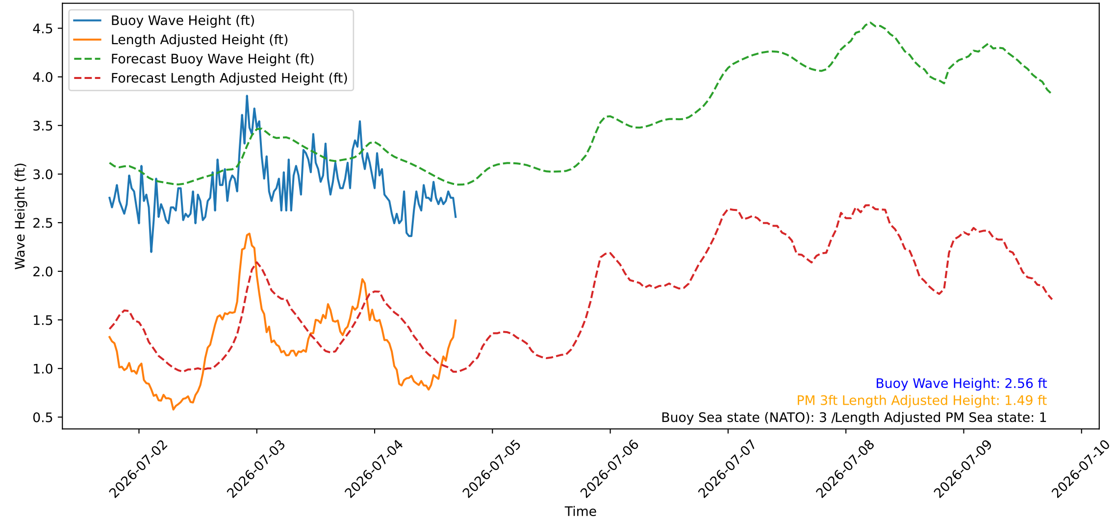
Wave Heights over Time for Red Beach at 2026-07-04 17:30:46
