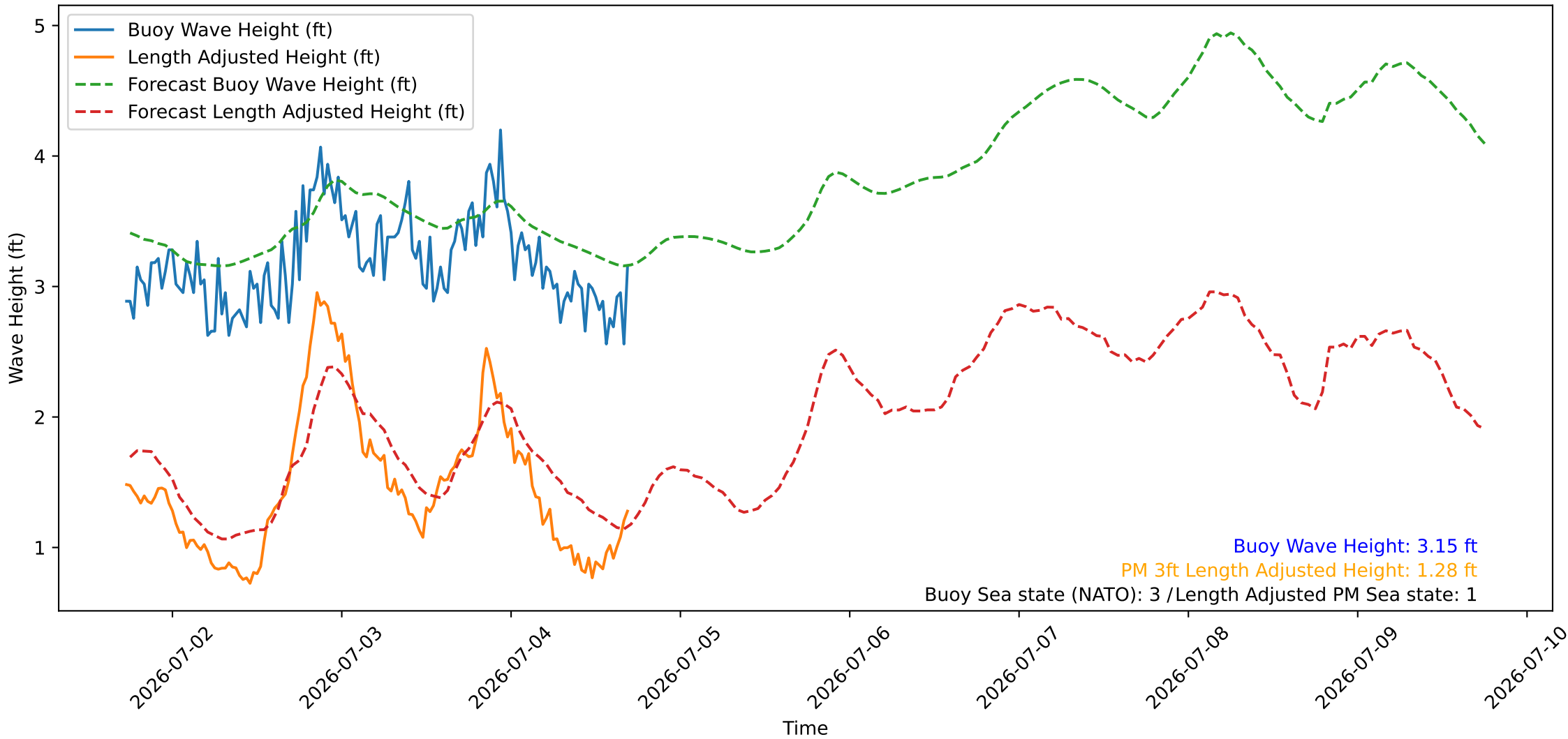
Wave Heights over Time for Green Beach at 2026-07-04 17:31:08
