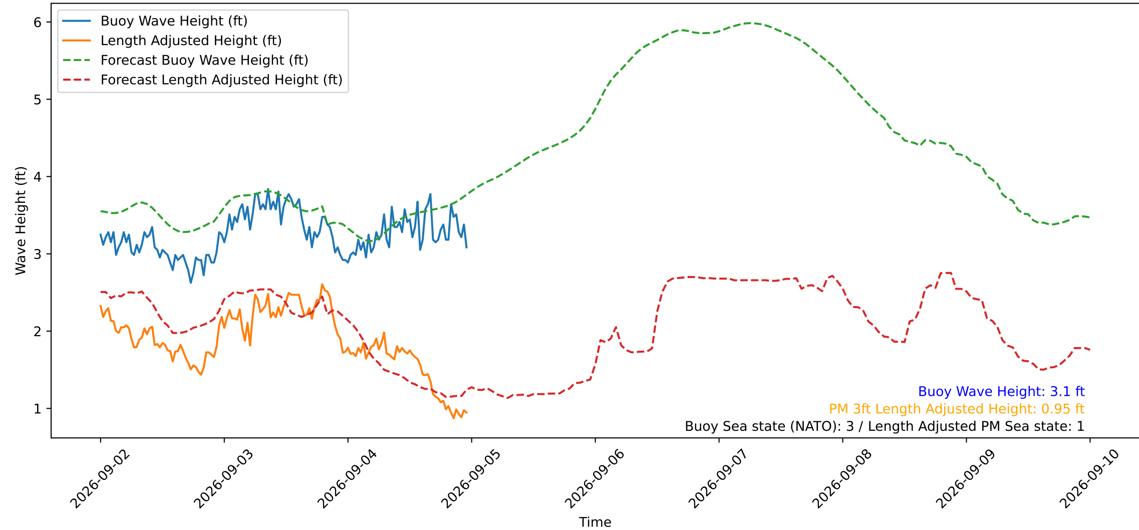
Wave Heights over Time for Oceanside Harbor at 2026-09-04 23:50:29
