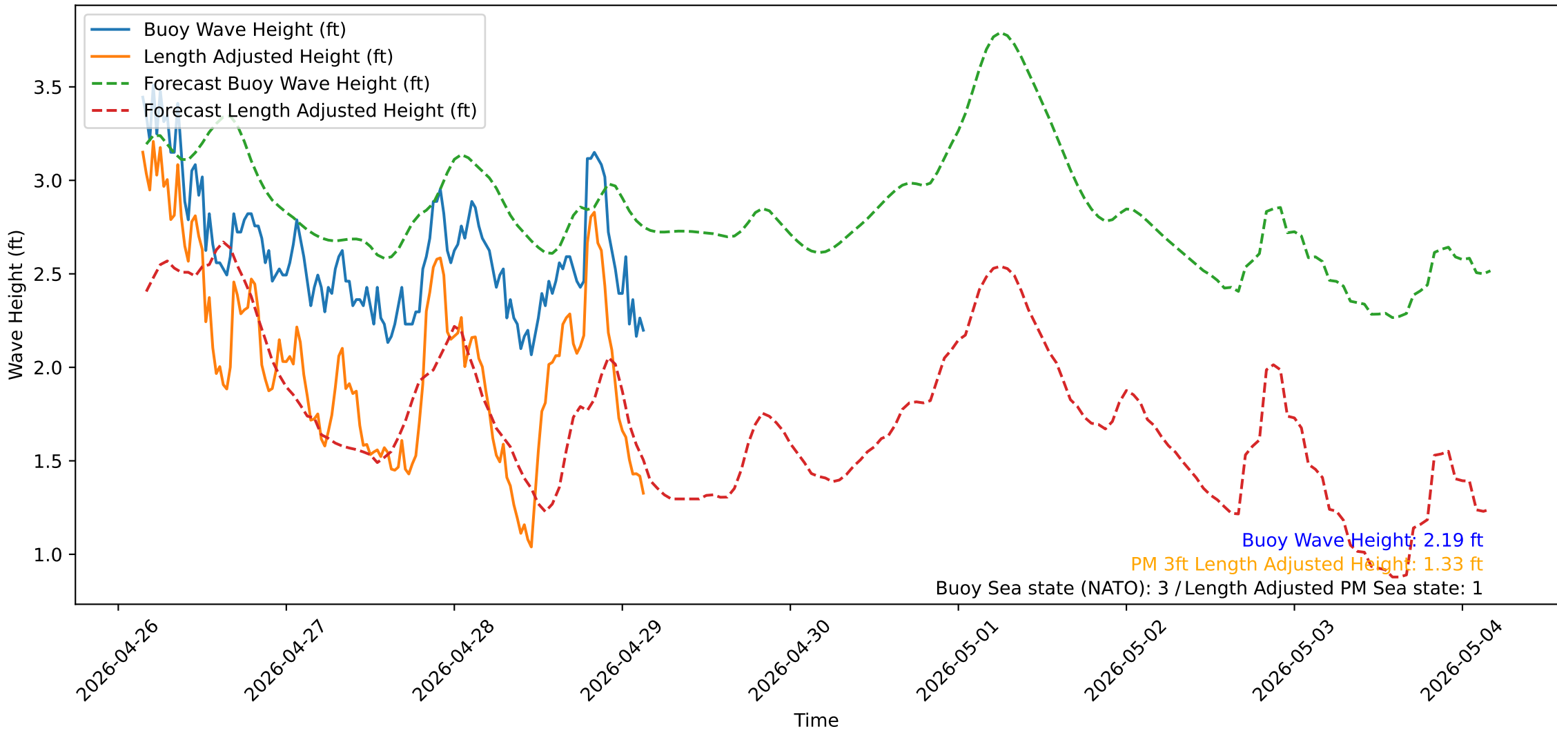
Wave Heights over Time for Green Beach at 2026-04-29 03:41:13
