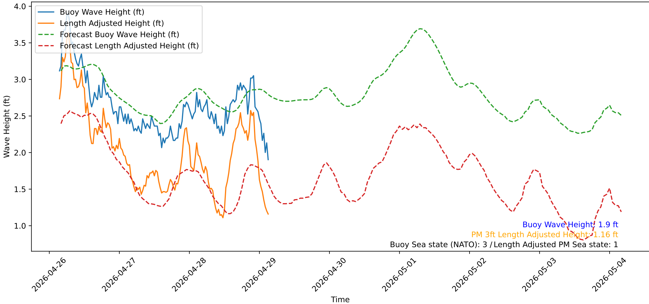
Wave Heights over Time for Oceanside Harbor at 2026-04-29 03:40:31
