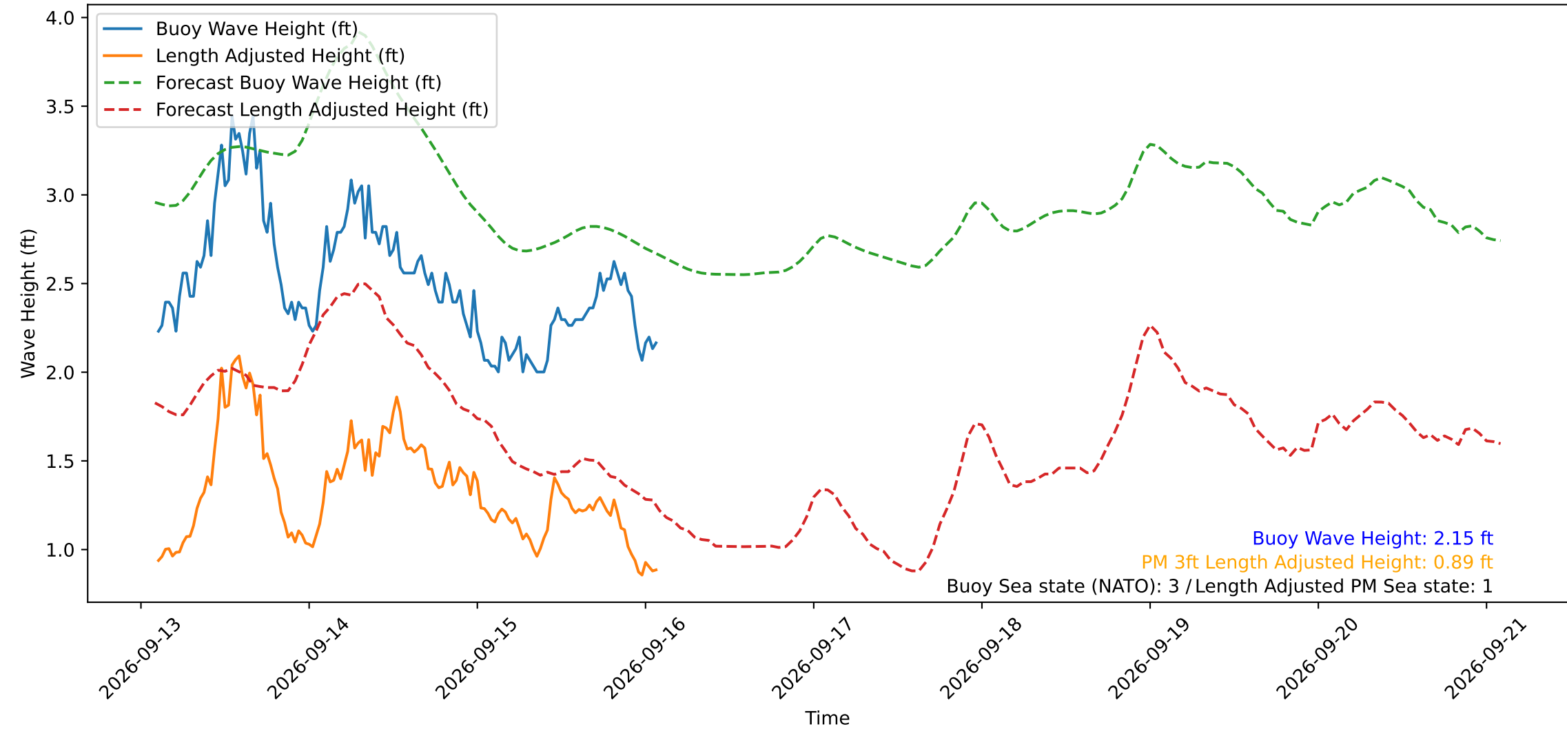
Wave Heights over Time for Red Beach at 2026-09-16 02:10:50
