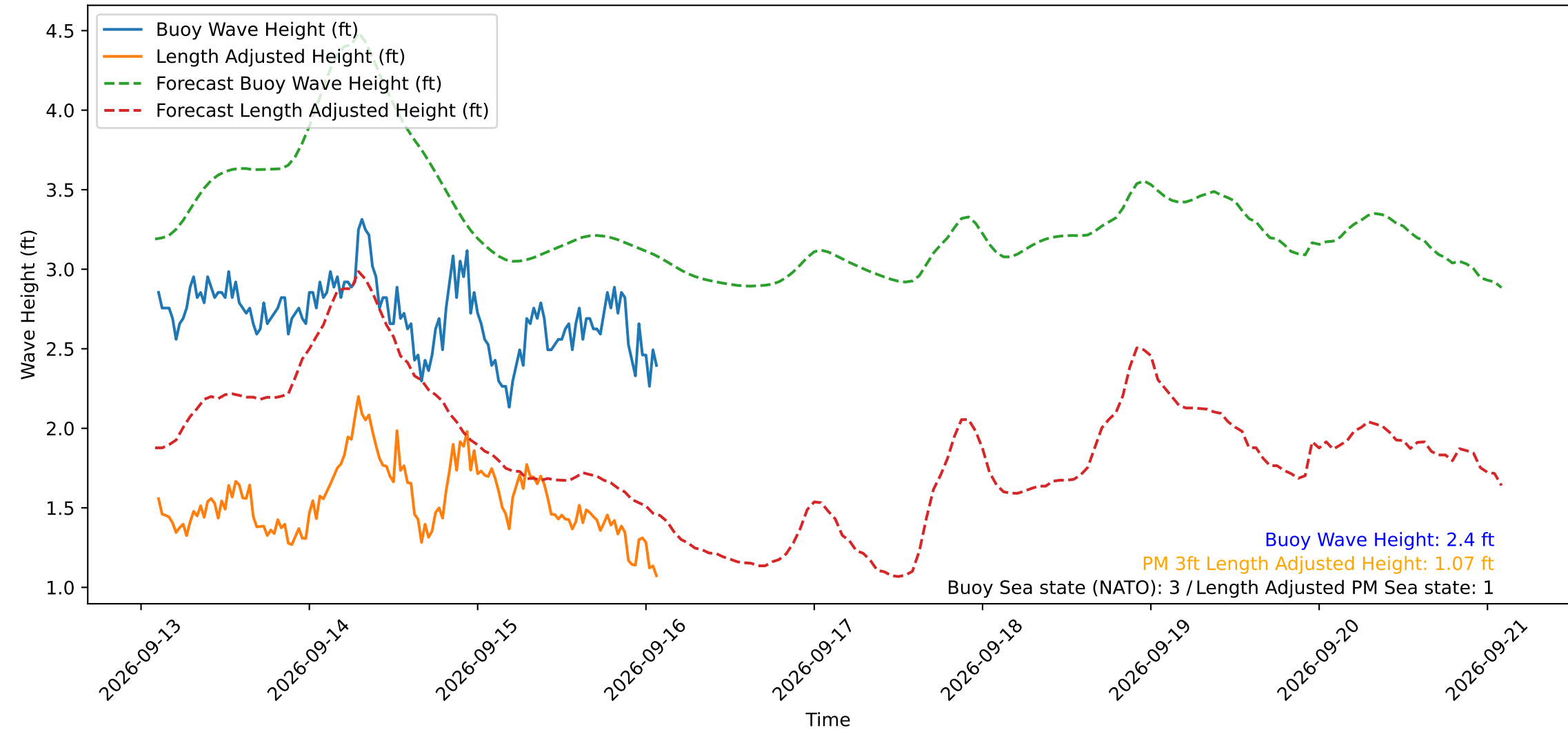
Wave Heights over Time for Green Beach at 2026-09-16 02:11:12
