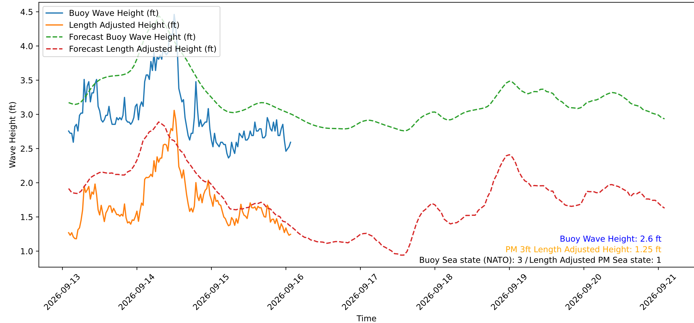
Wave Heights over Time for Oceanside Harbor at 2026-09-16 02:10:29
