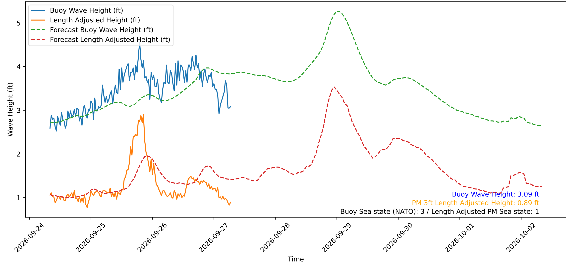
Wave Heights over Time for Green Beach at 2026-09-27 07:31:13
