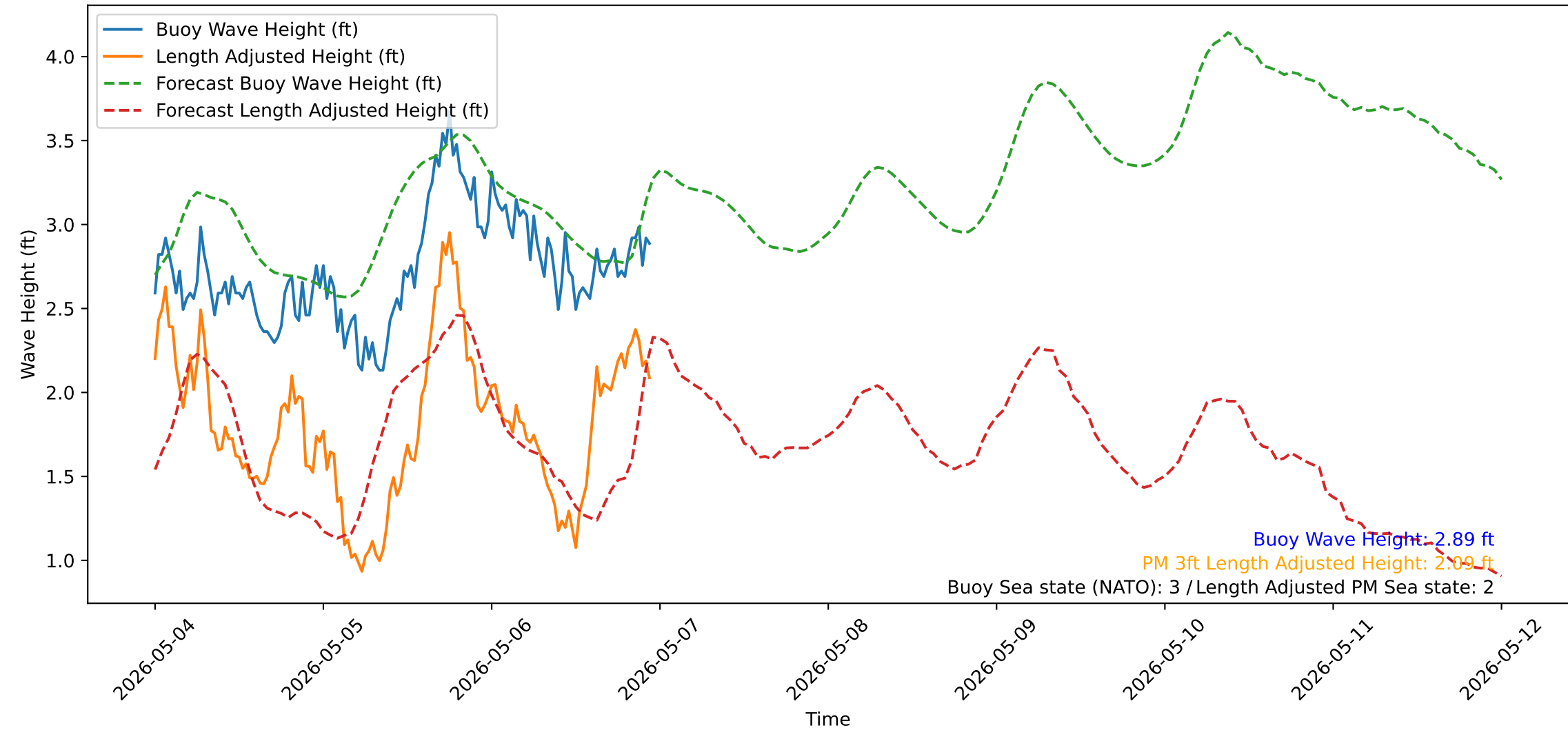
Wave Heights over Time for Green Beach at 2026-05-07 00:01:12
