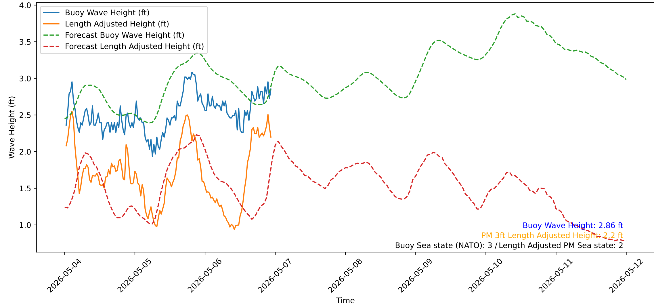
Wave Heights over Time for Red Beach at 2026-05-07 00:00:50
