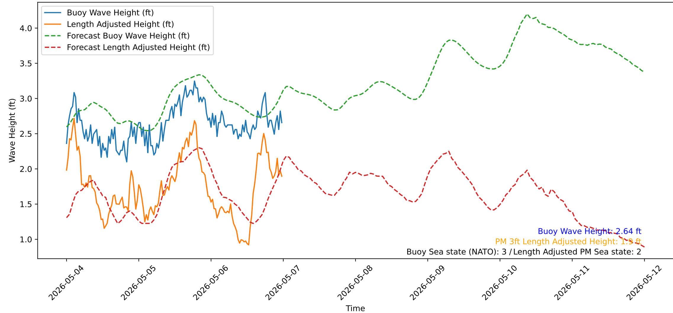
Wave Heights over Time for Oceanside Harbor at 2026-05-07 00:00:31
