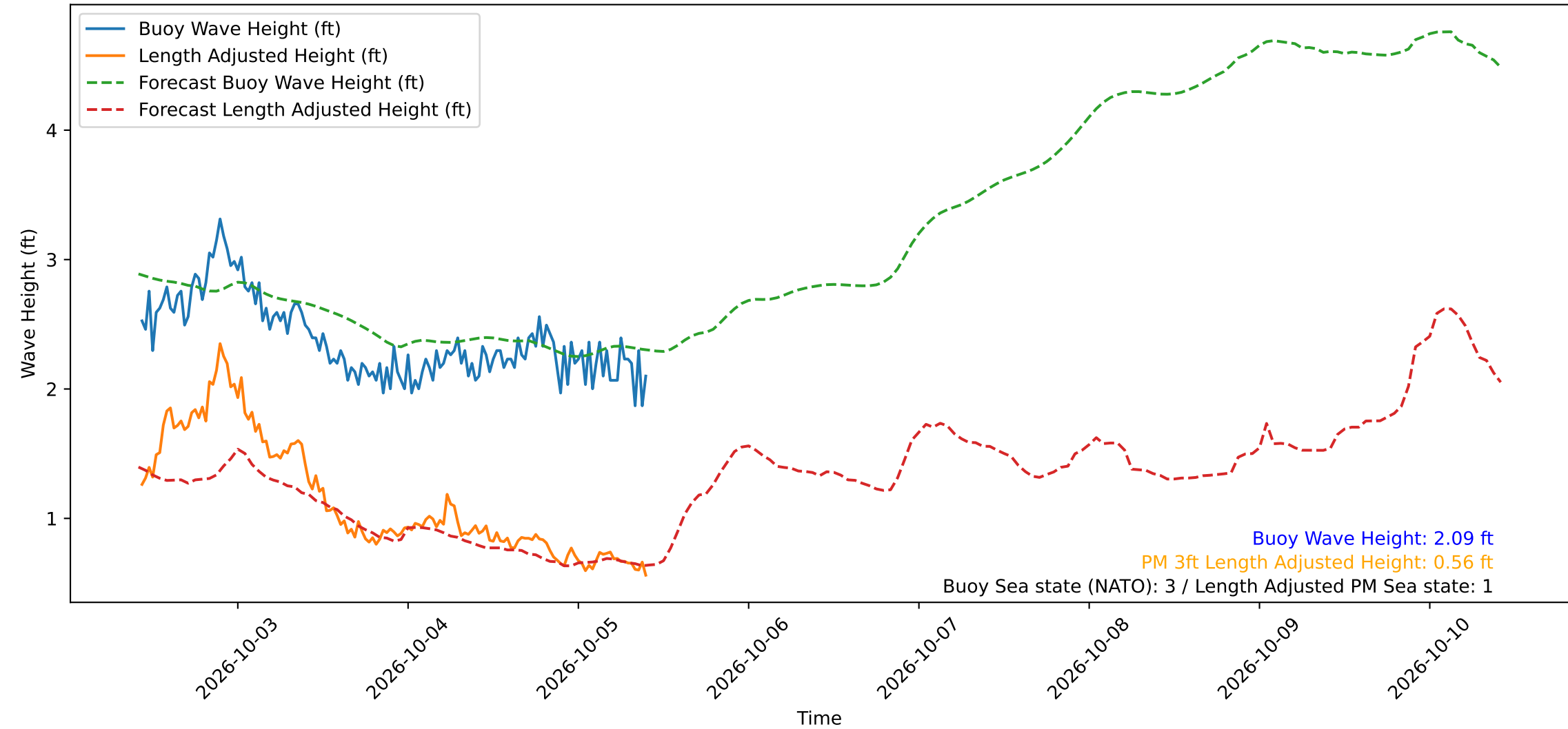
Wave Heights over Time for Oceanside Harbor at 2026-10-05 10:20:30
