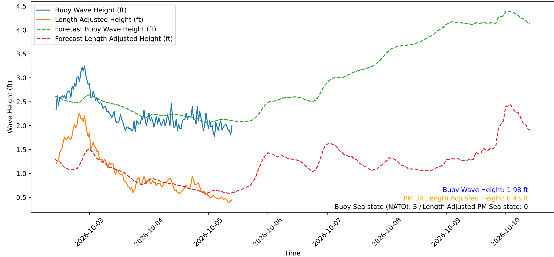
Wave Heights over Time for Red Beach at 2026-10-05 10:20:50
