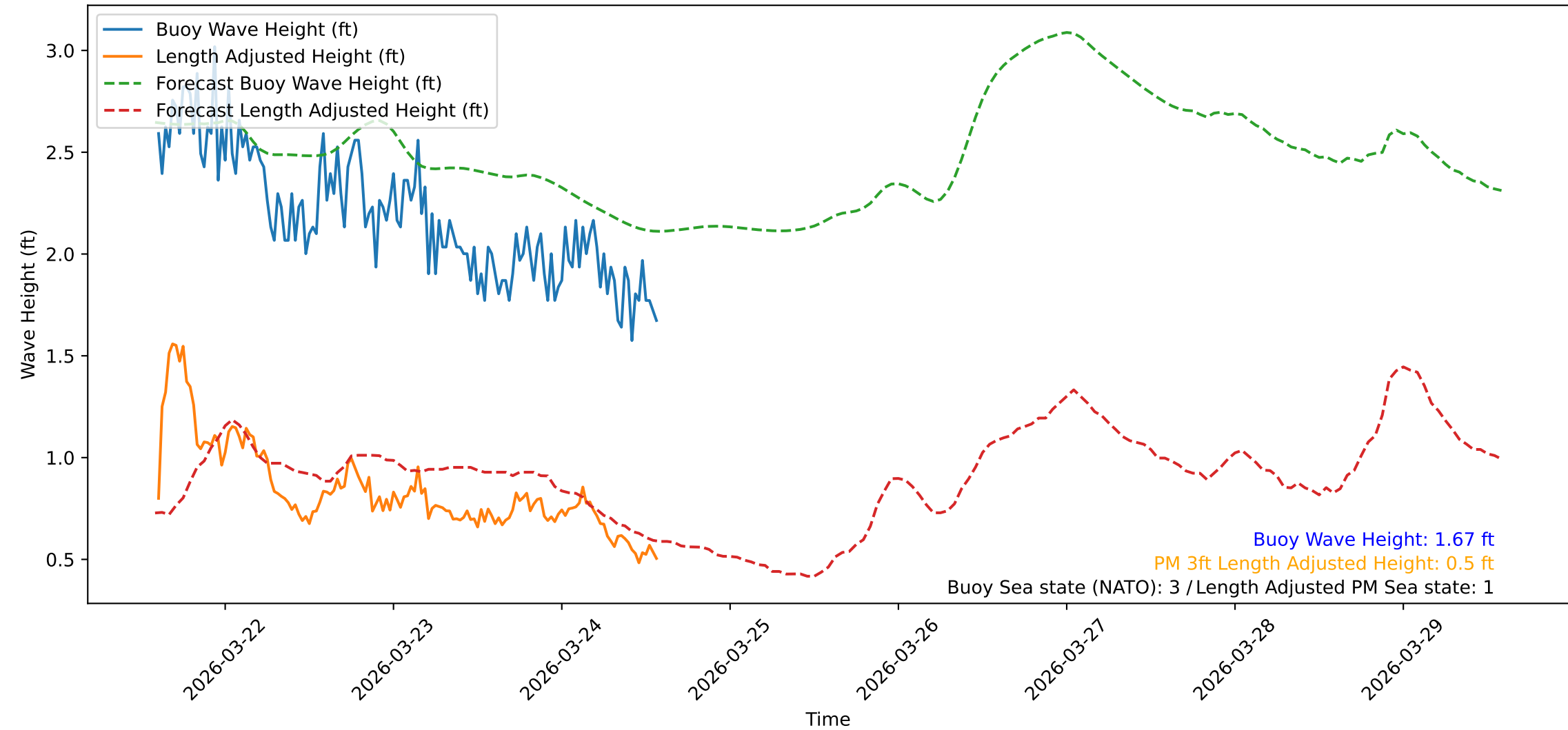
Wave Heights over Time for Oceanside Harbor at 2026-03-24 14:20:31
