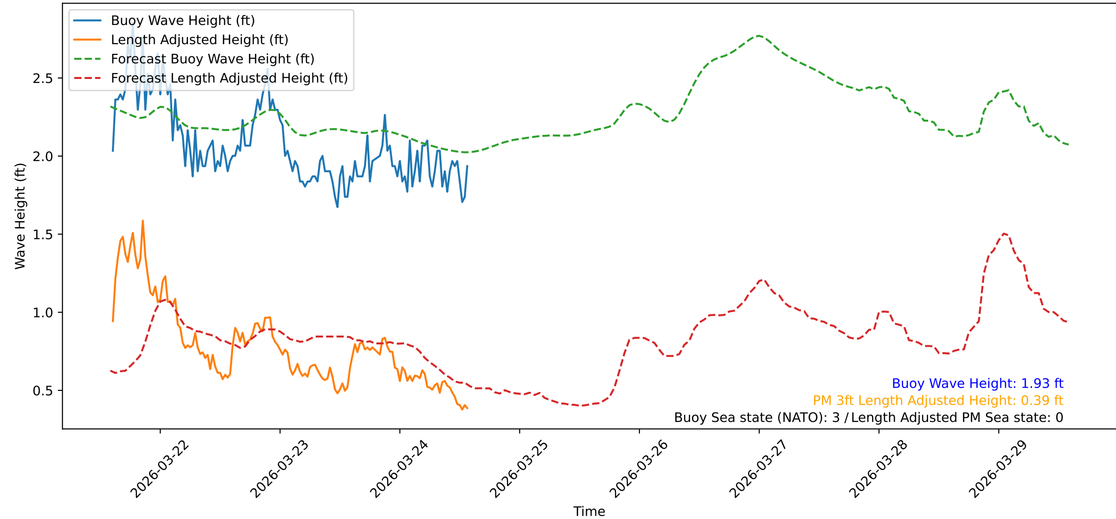
Wave Heights over Time for Red Beach at 2026-03-24 14:20:47
