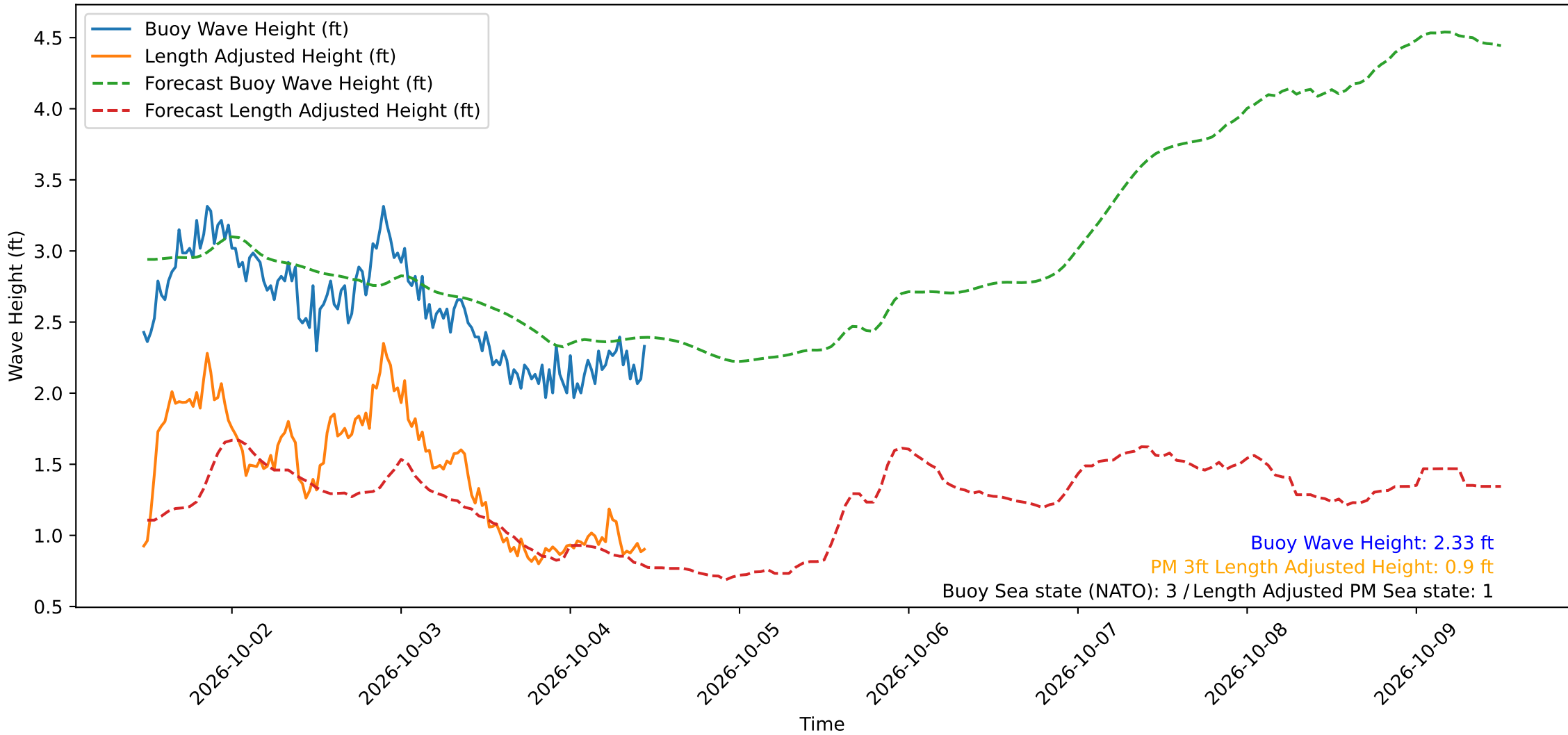
Wave Heights over Time for Oceanside Harbor at 2026-10-04 11:30:30
