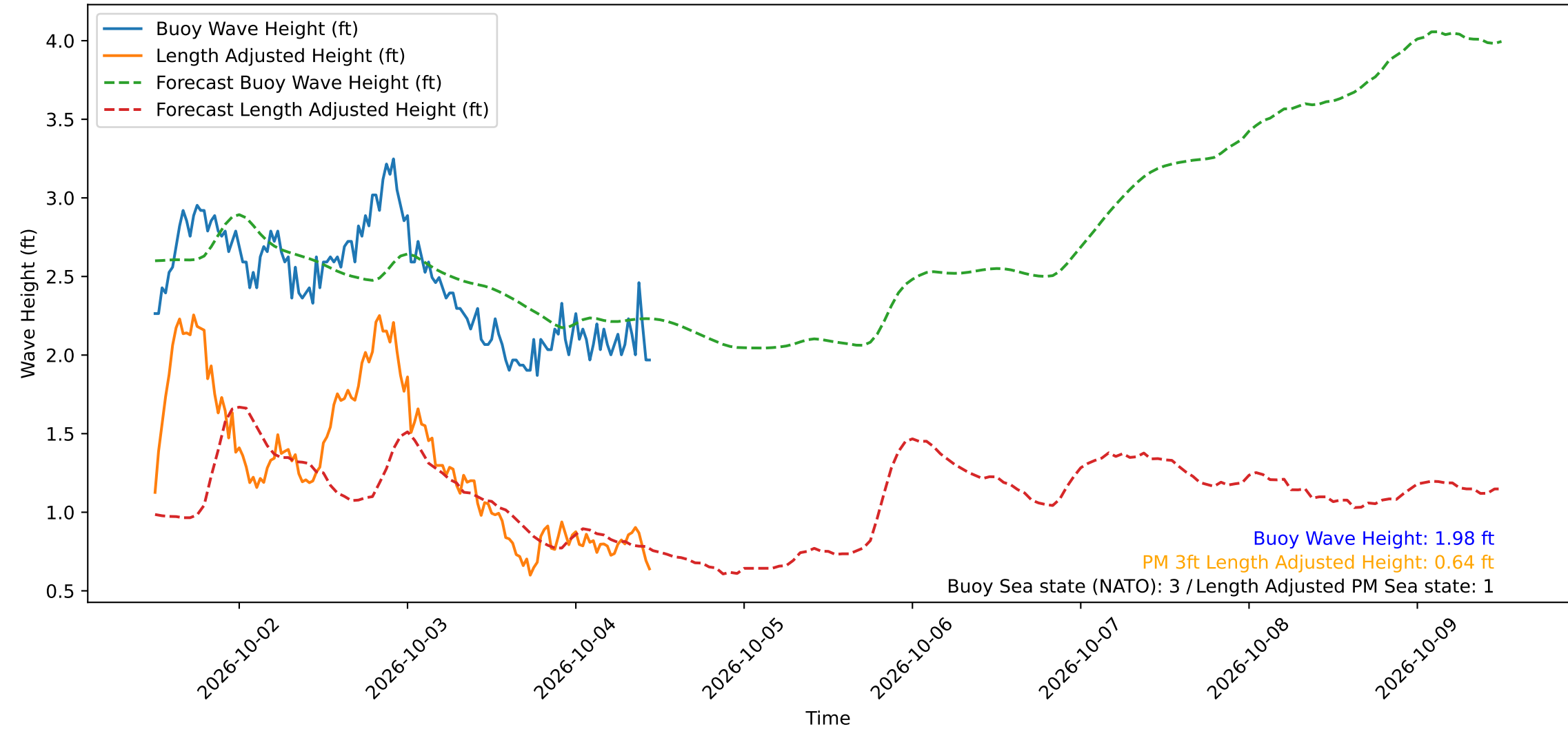
Wave Heights over Time for Red Beach at 2026-10-04 11:30:49
