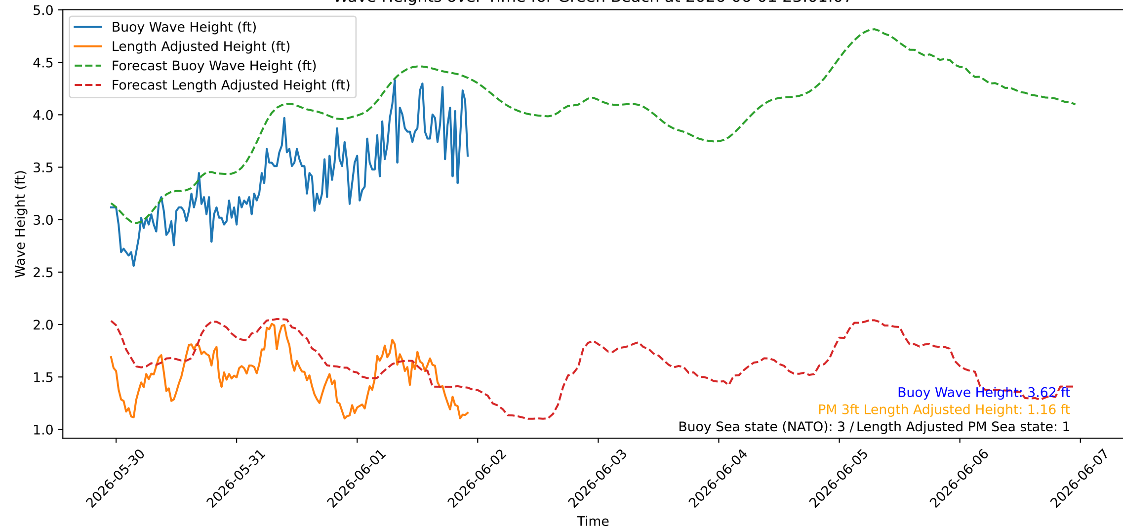
Wave Heights over Time for Green Beach at 2026-06-01 23:01:07
