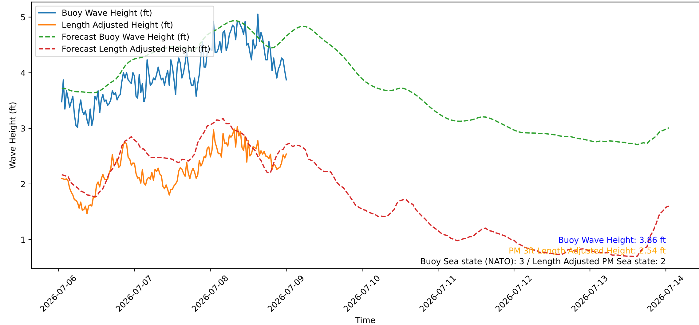
Wave Heights over Time for Oceanside Harbor at 2026-07-09 01:00:26
