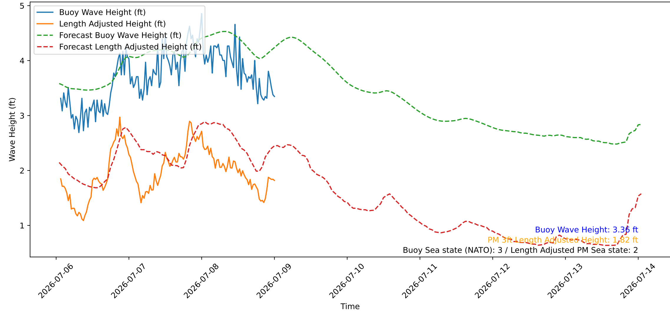
Wave Heights over Time for Red Beach at 2026-07-09 01:00:45
