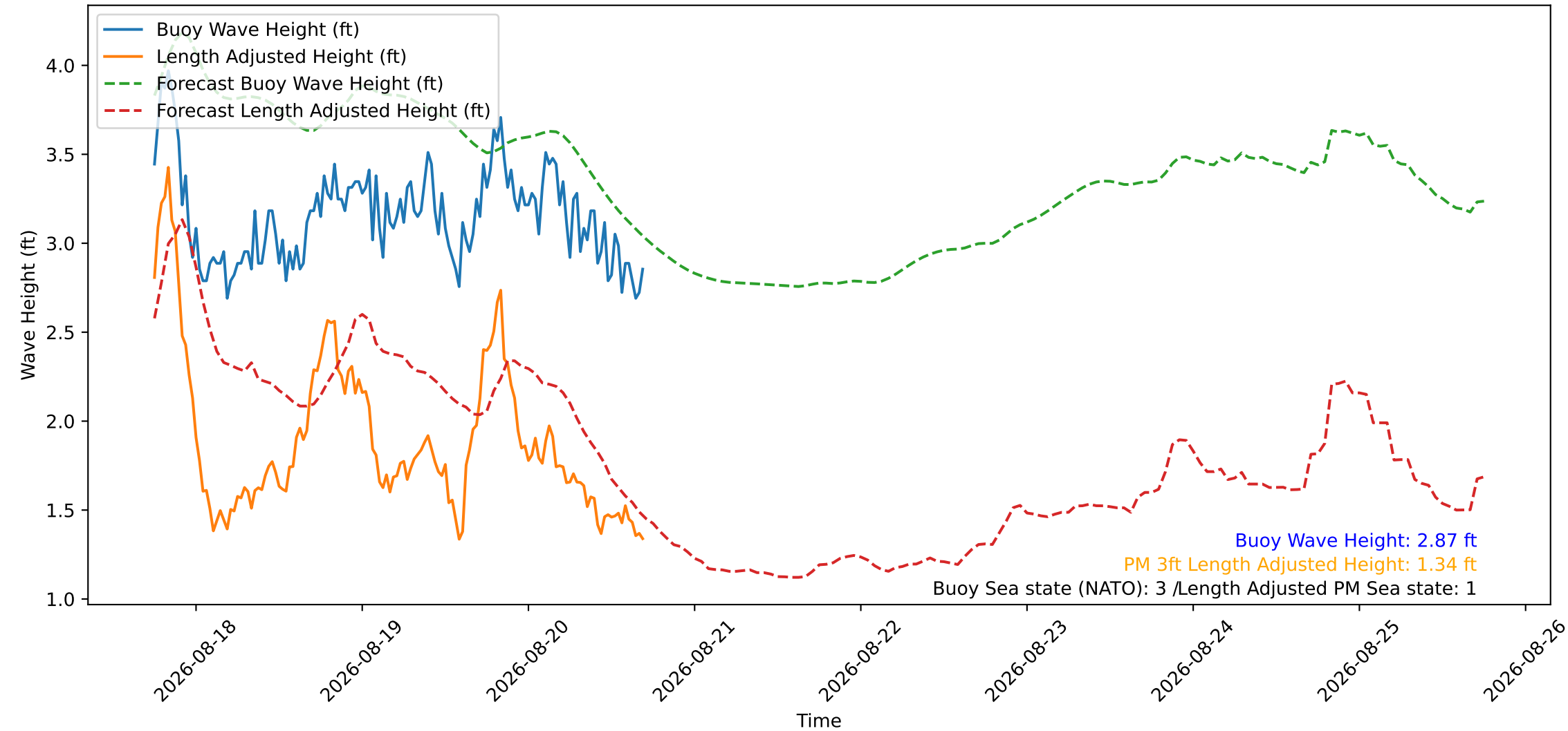
Wave Heights over Time for Green Beach at 2026-08-20 17:31:09
