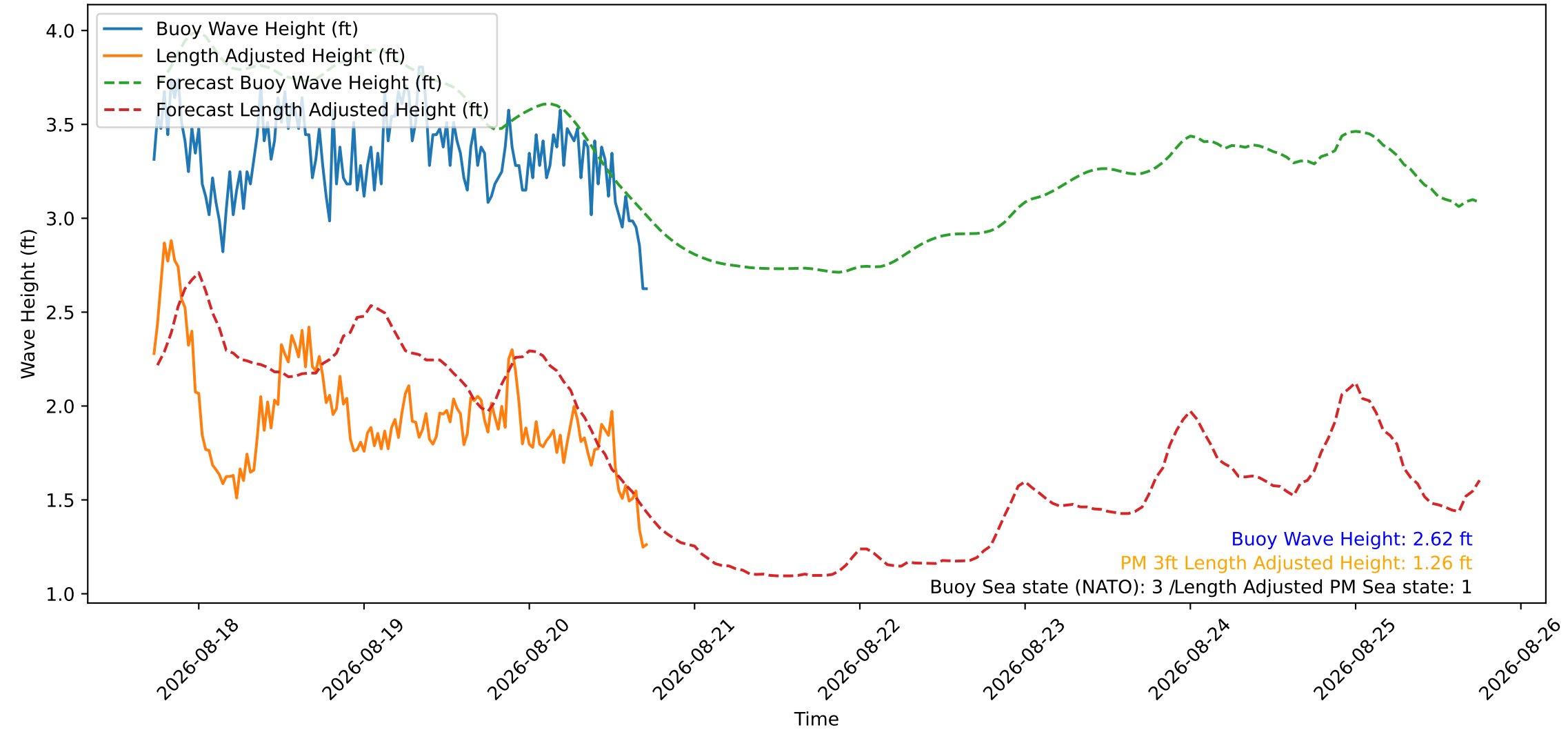
Wave Heights over Time for Oceanside Harbor at 2026-08-20 17:30:27
