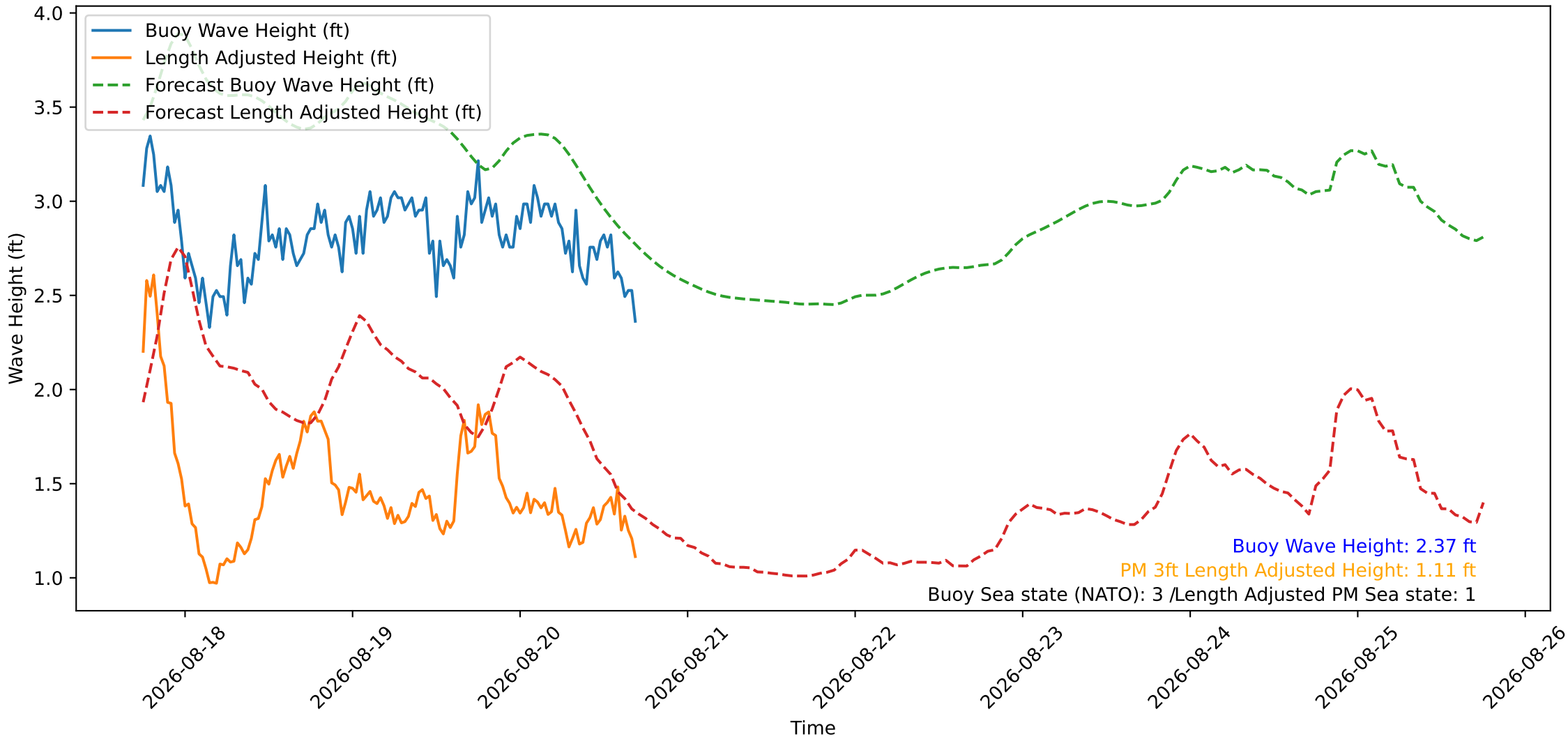
Wave Heights over Time for Red Beach at 2026-08-20 17:30:46
