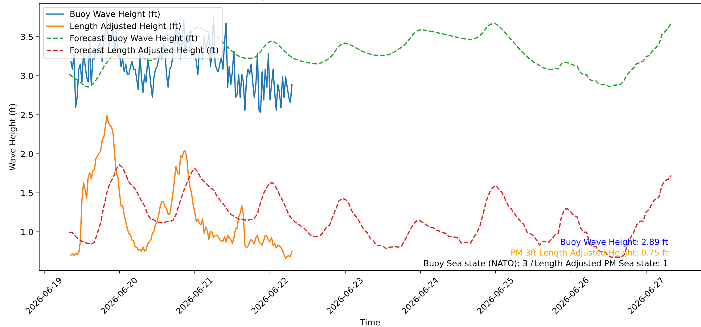
Wave Heights over Time for Red Beach at 2026-06-22 08:10:45
