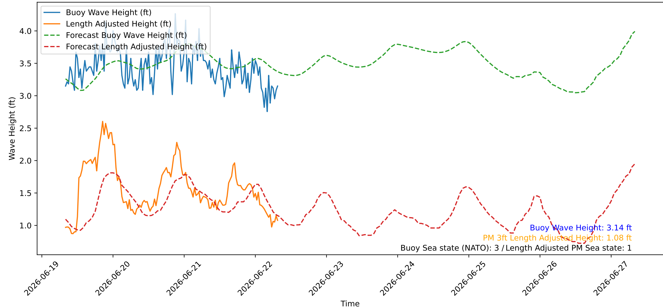
Wave Heights over Time for Oceanside Harbor at 2026-06-22 08:10:26
