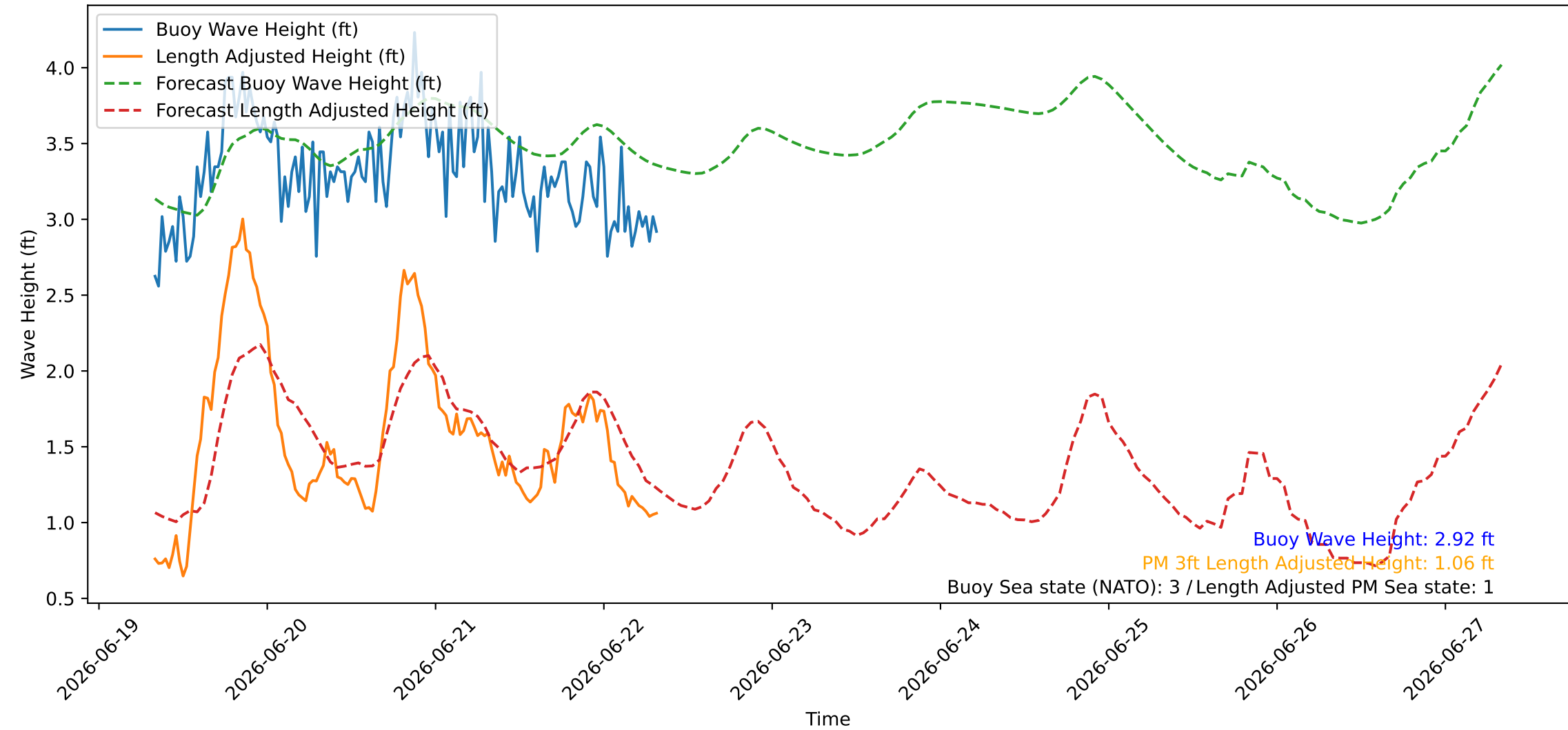
Wave Heights over Time for Green Beach at 2026-06-22 08:11:08
