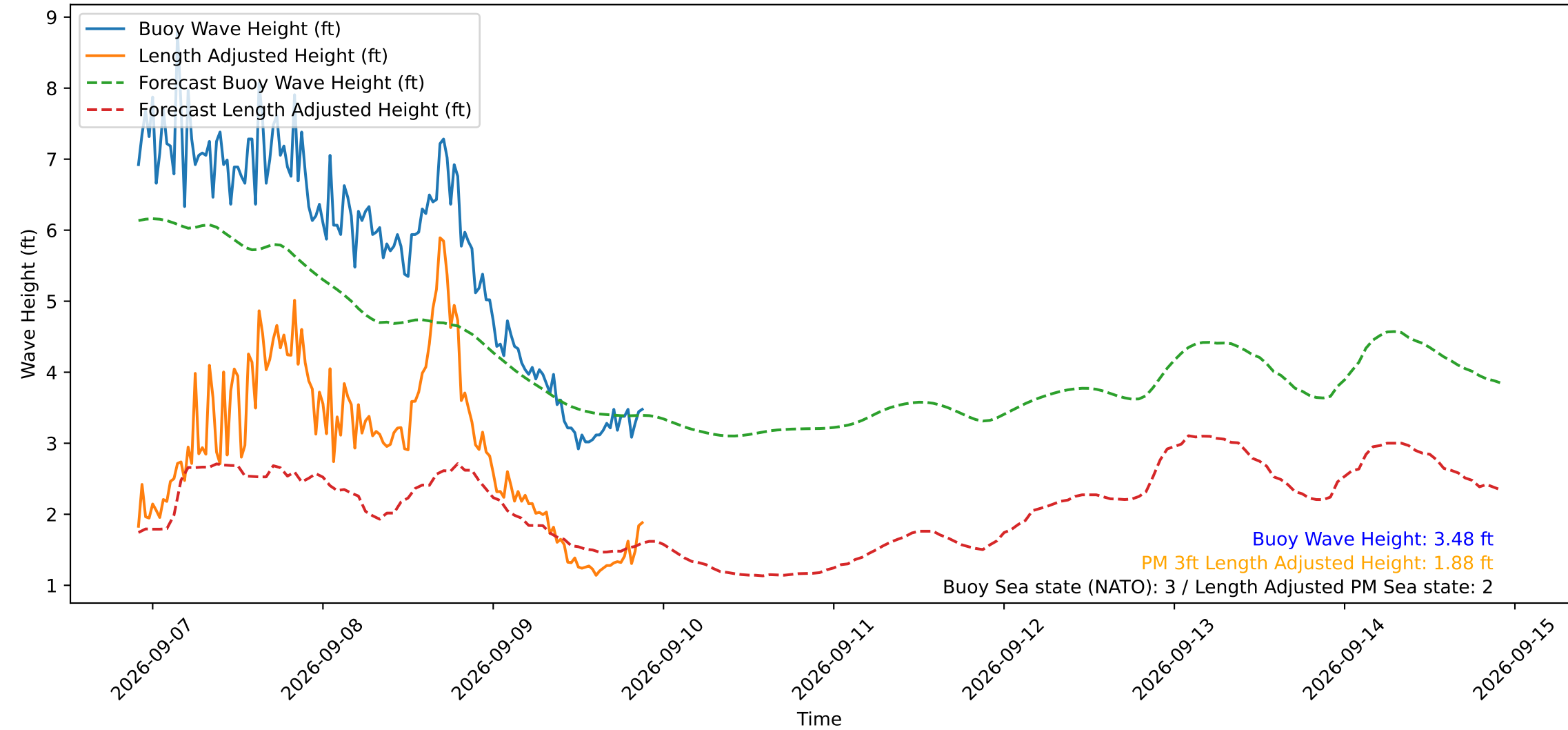
Wave Heights over Time for Green Beach at 2026-09-09 21:41:11
