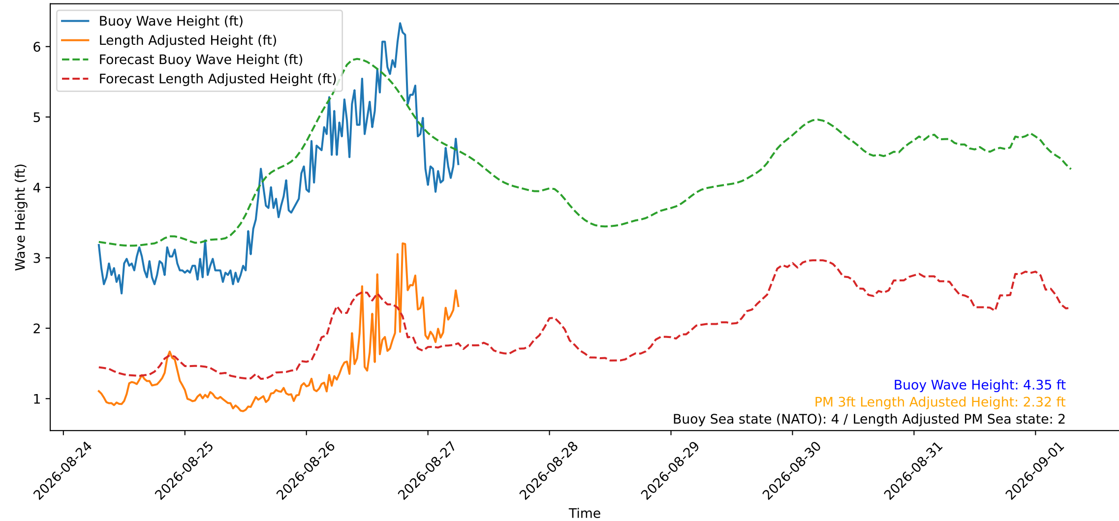
Wave Heights over Time for Green Beach at 2026-08-27 06:51:14
