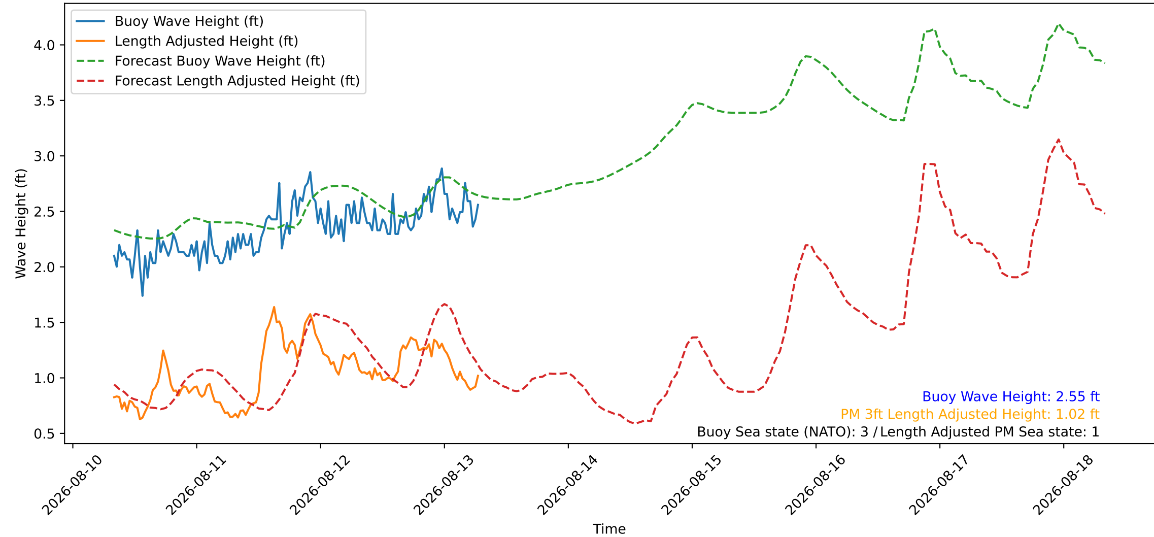
Wave Heights over Time for Red Beach at 2026-08-13 07:30:46
