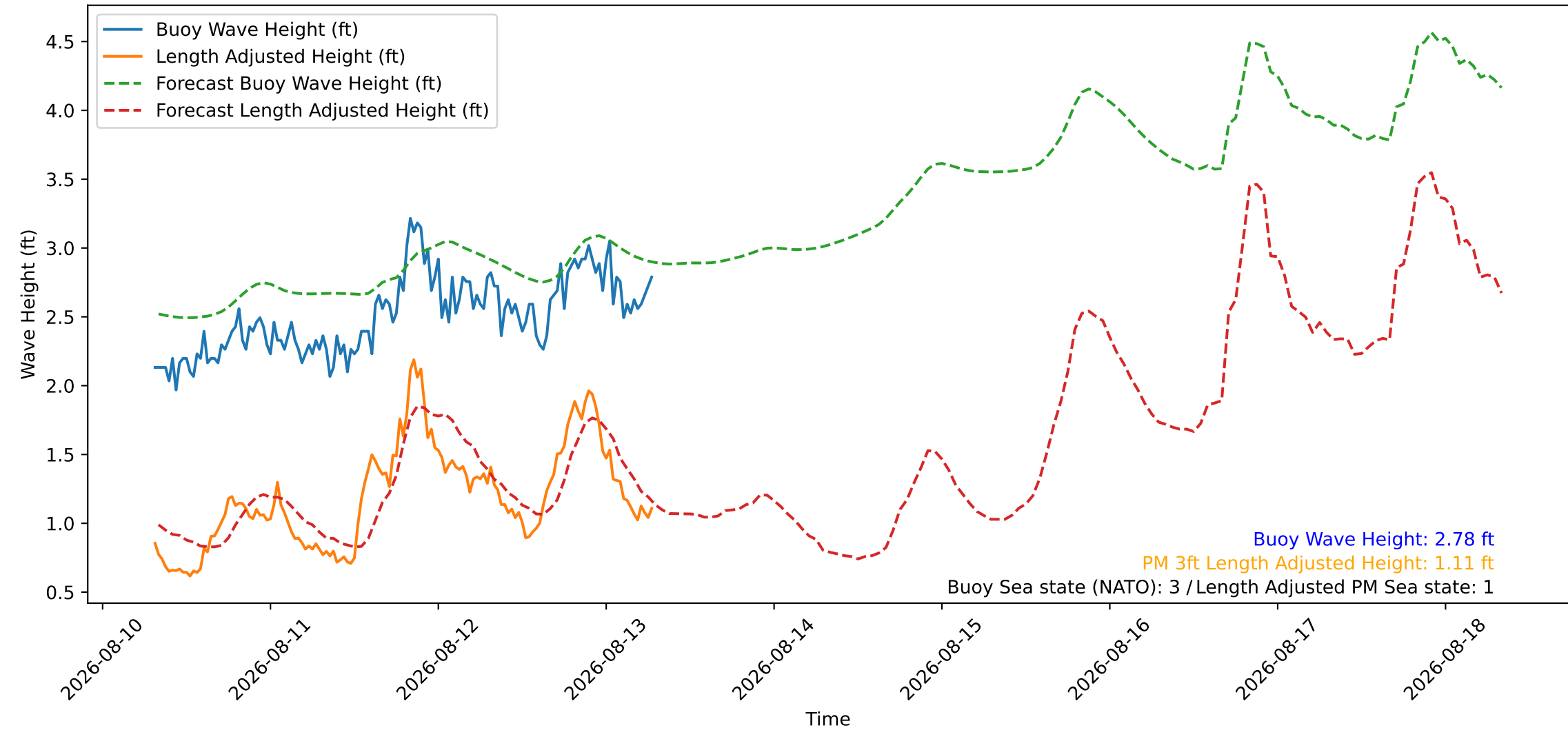
Wave Heights over Time for Green Beach at 2026-08-13 07:31:08
