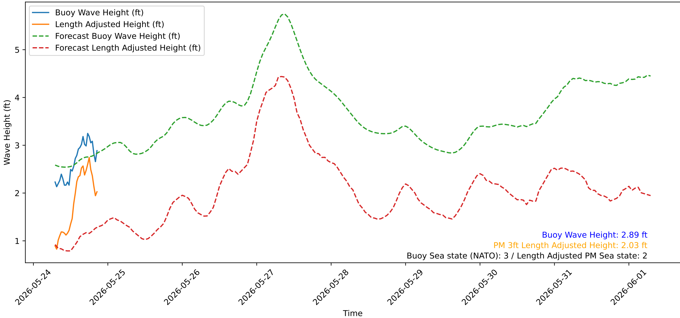
Wave Heights over Time for Oceanside Harbor at 2026-05-27 07:10:26
