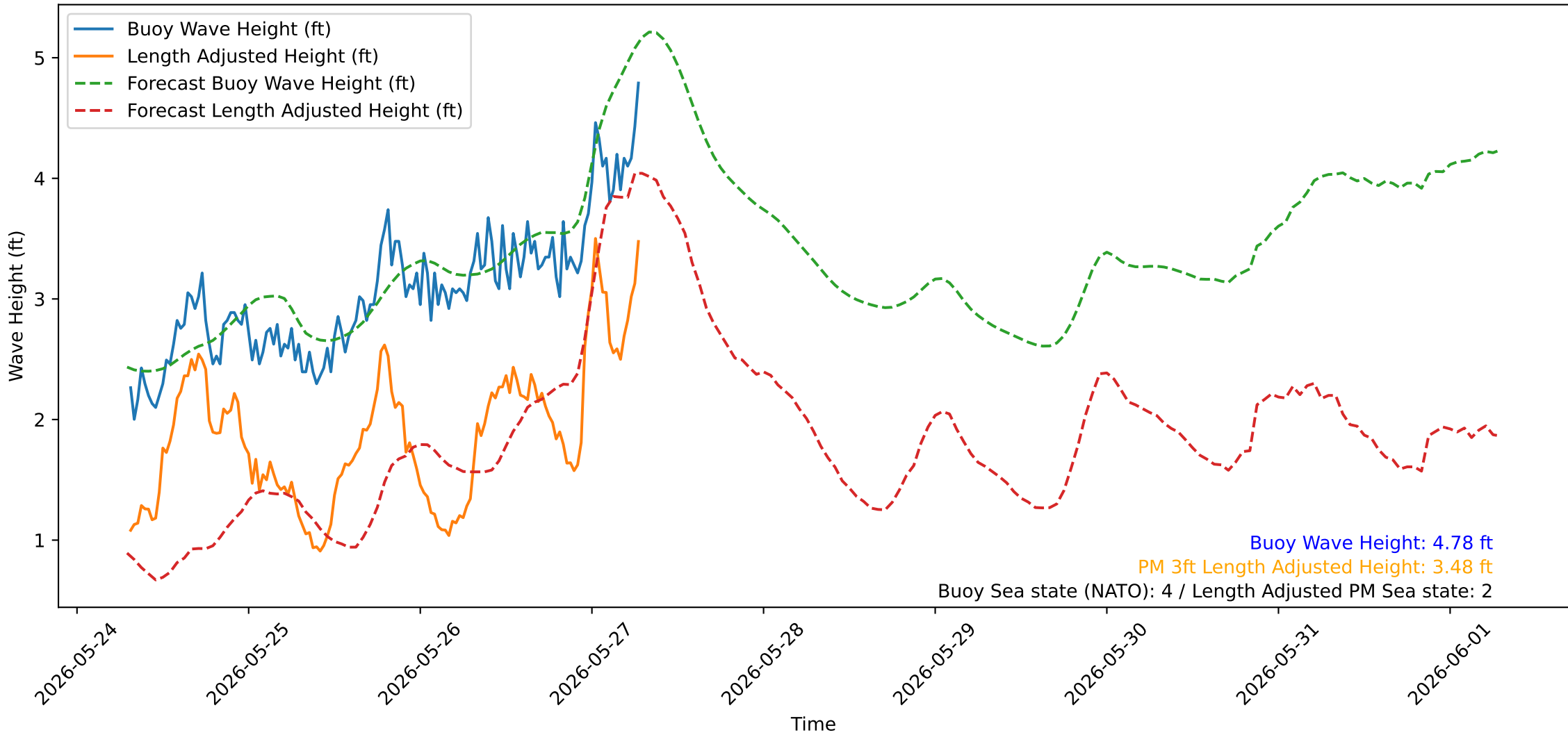
Wave Heights over Time for Red Beach at 2026-05-27 07:10:45
