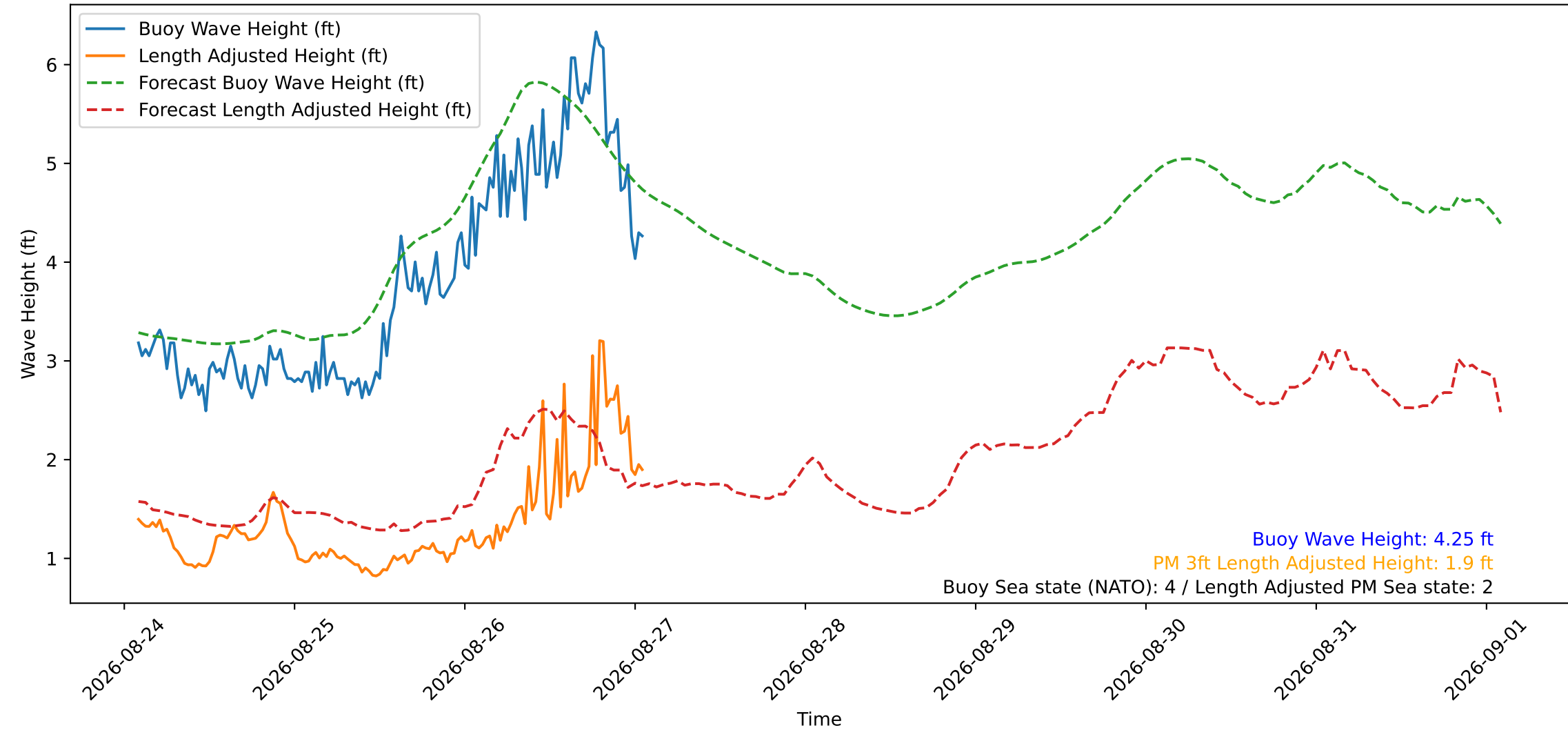
Wave Heights over Time for Green Beach at 2026-08-27 01:41:13
