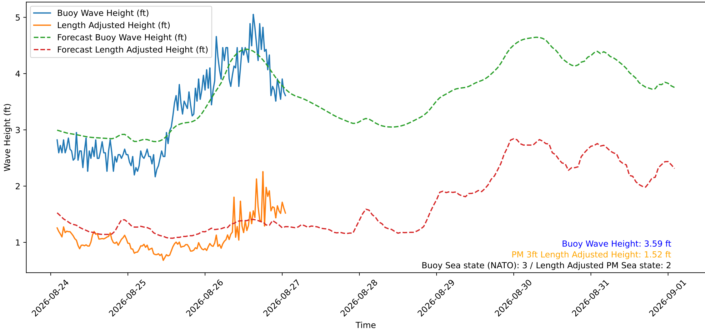
Wave Heights over Time for Red Beach at 2026-08-27 01:40:50
