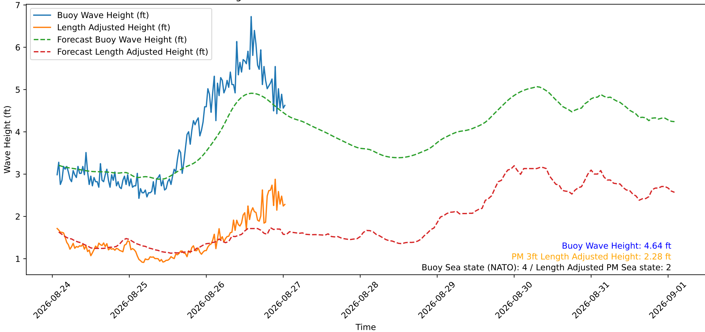
Wave Heights over Time for Oceanside Harbor at 2026-08-27 01:40:30
