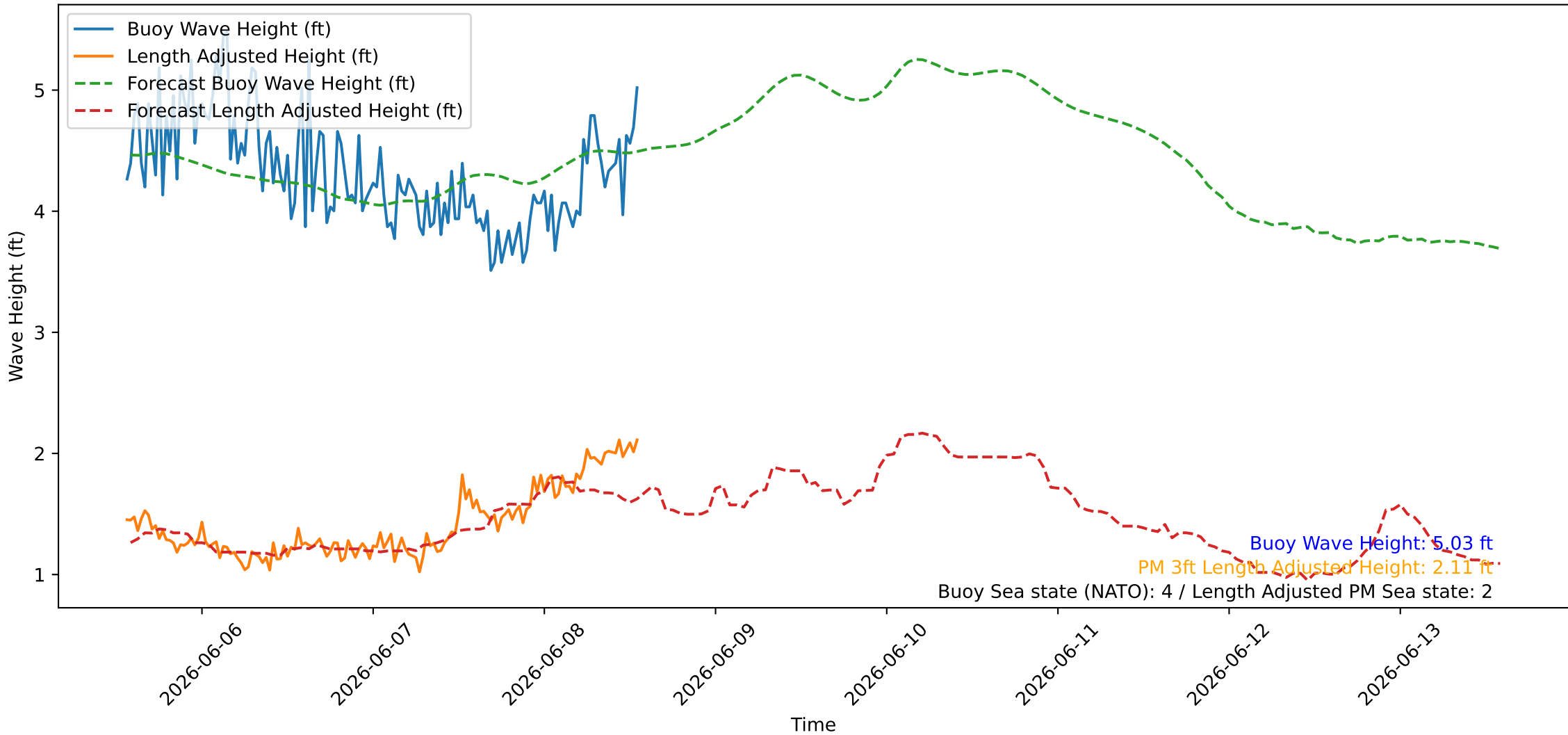
Wave Heights over Time for Oceanside Harbor at 2026-06-08 13:40:25
