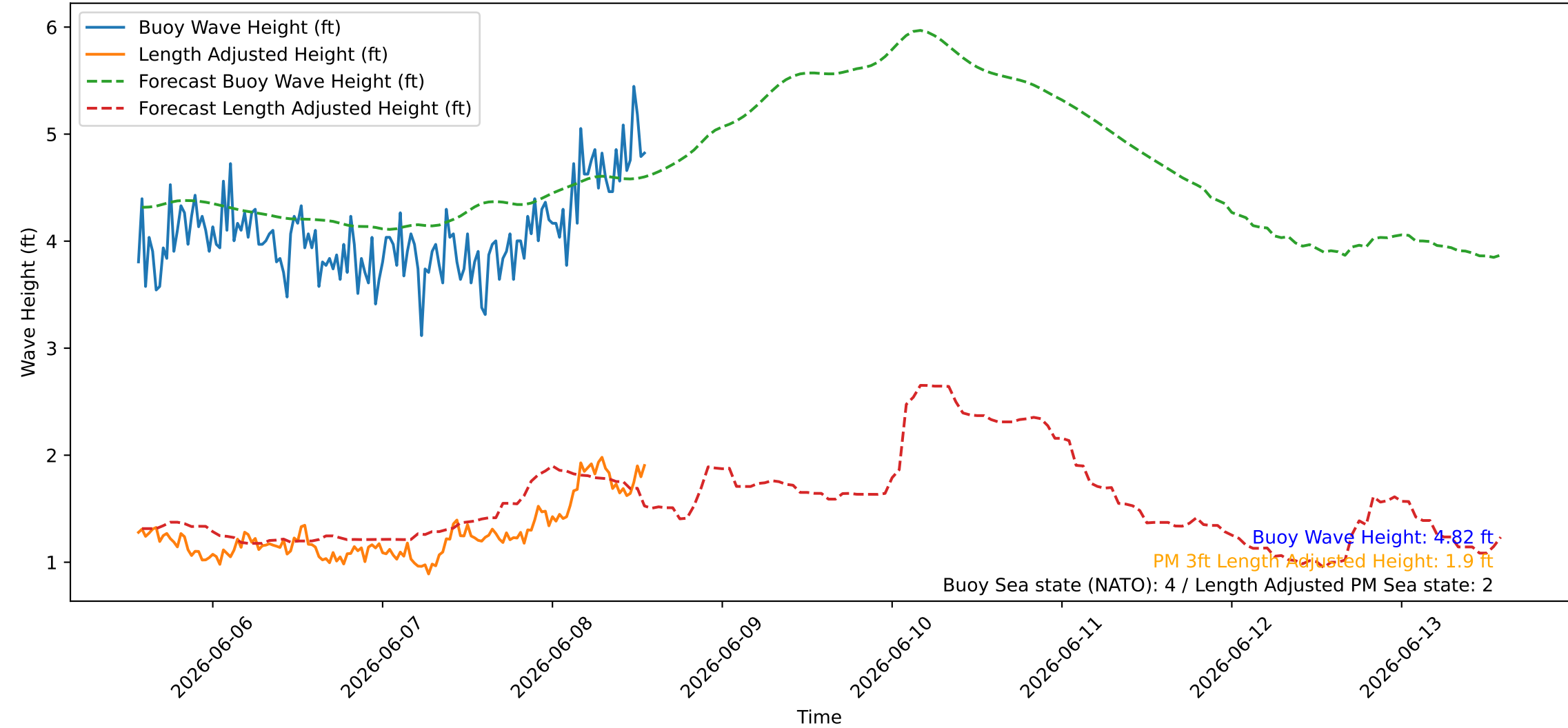
Wave Heights over Time for Green Beach at 2026-06-08 13:41:08
