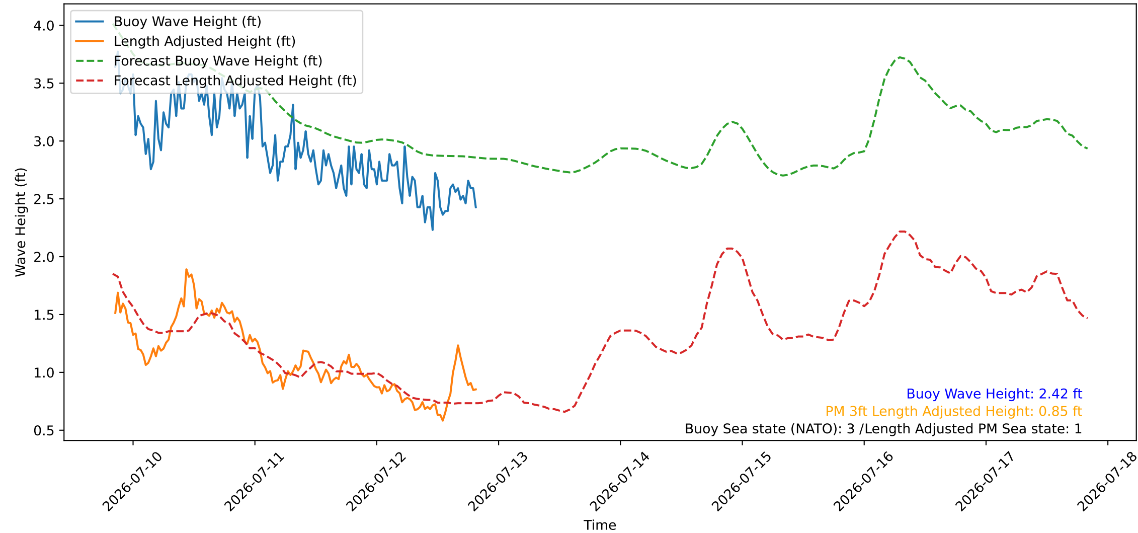
Wave Heights over Time for Green Beach at 2026-07-12 20:21:08
