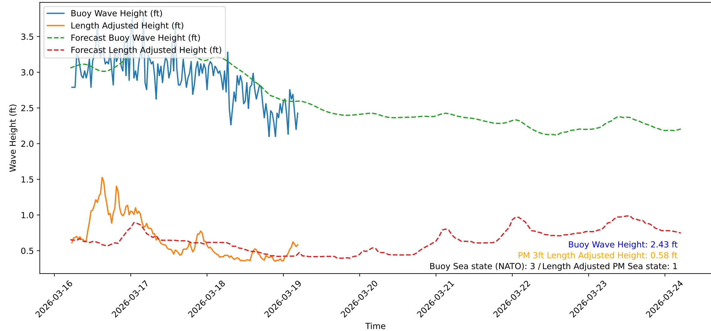
Wave Heights over Time for Red Beach at 2026-03-19 05:10:48
