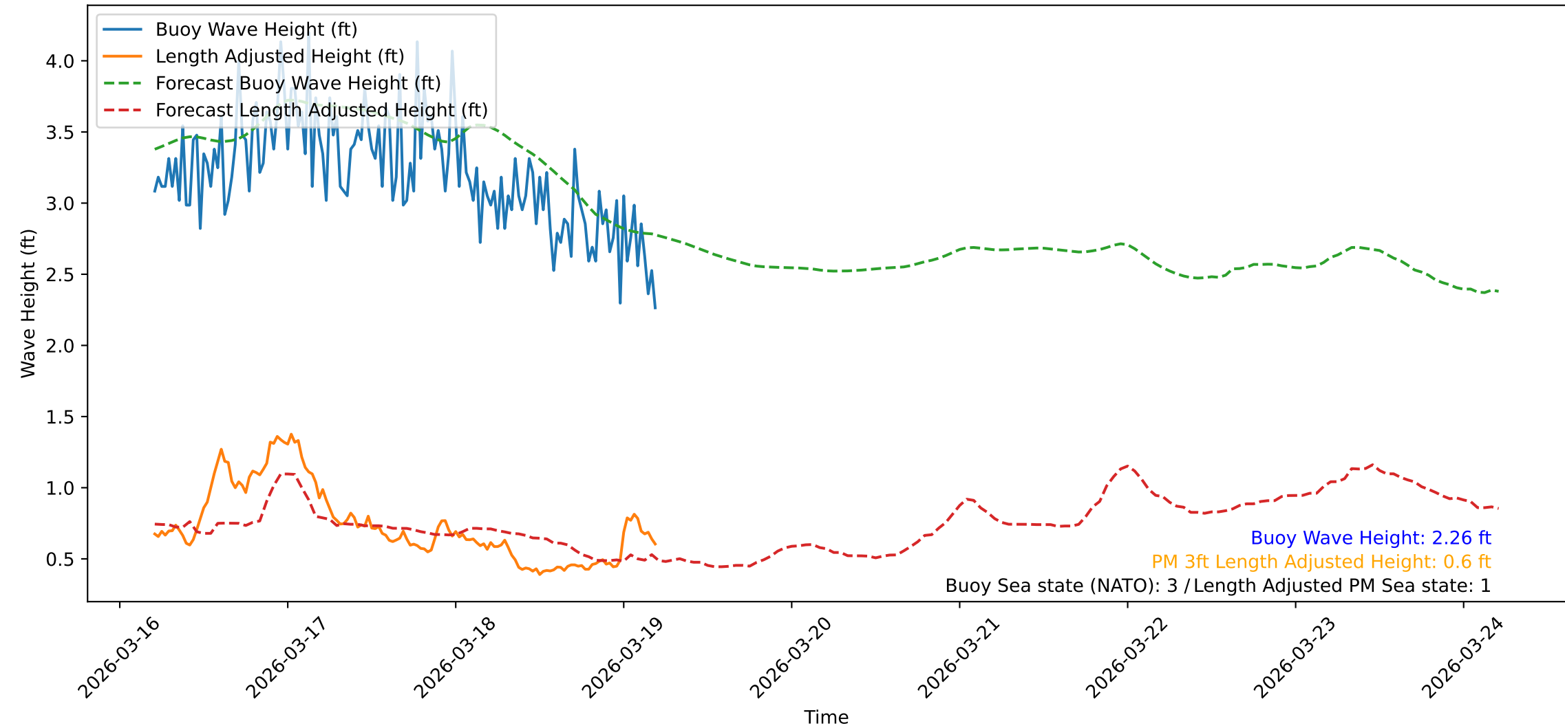
Wave Heights over Time for Green Beach at 2026-03-19 05:11:10
