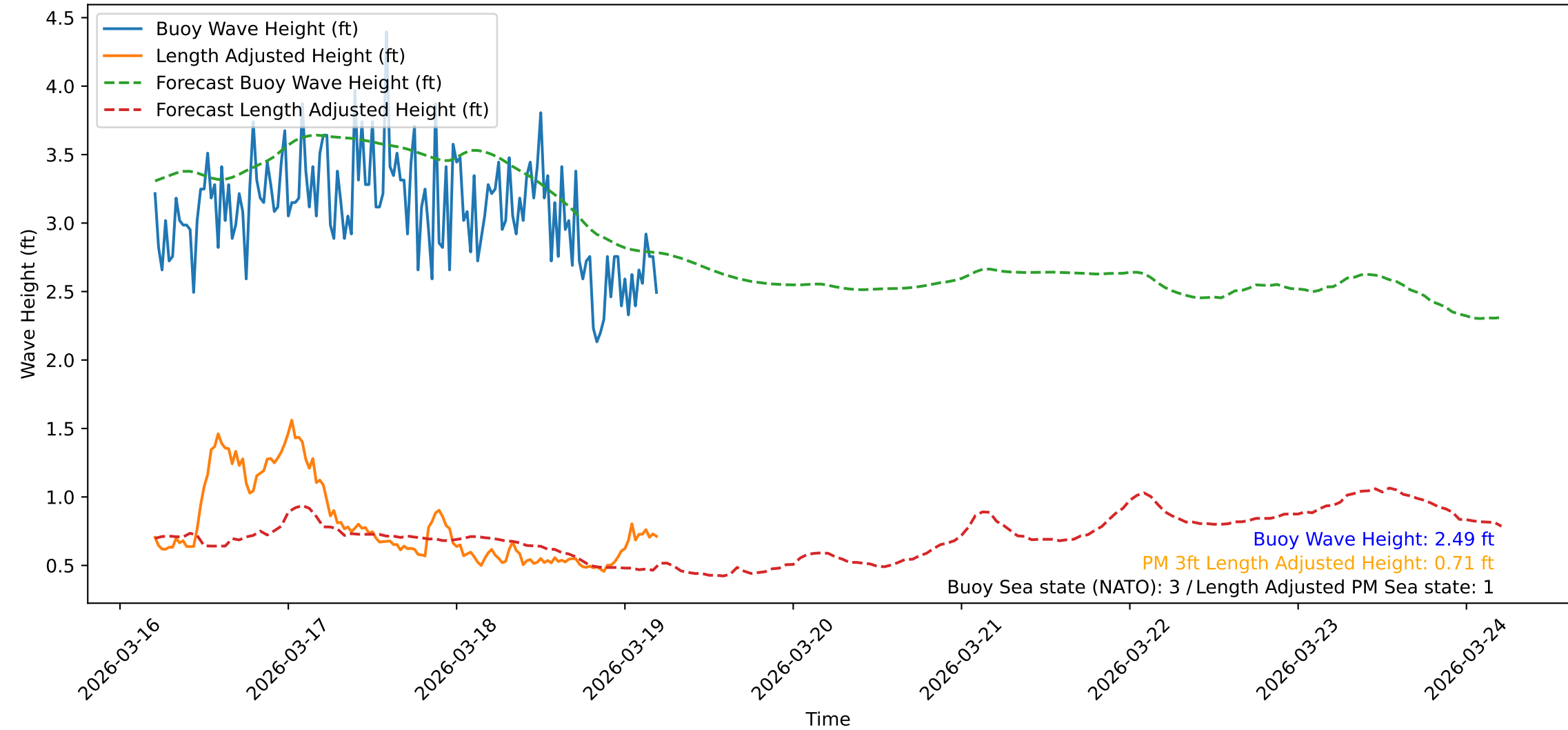
Wave Heights over Time for Oceanside Harbor at 2026-03-19 05:10:32
