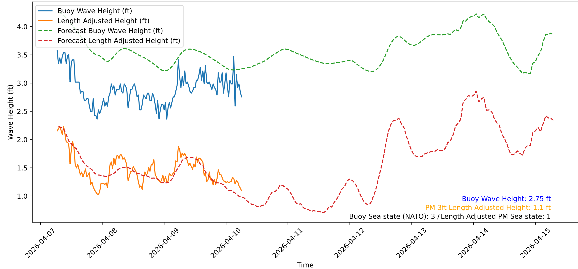
Wave Heights over Time for Green Beach at 2026-04-10 06:41:14
