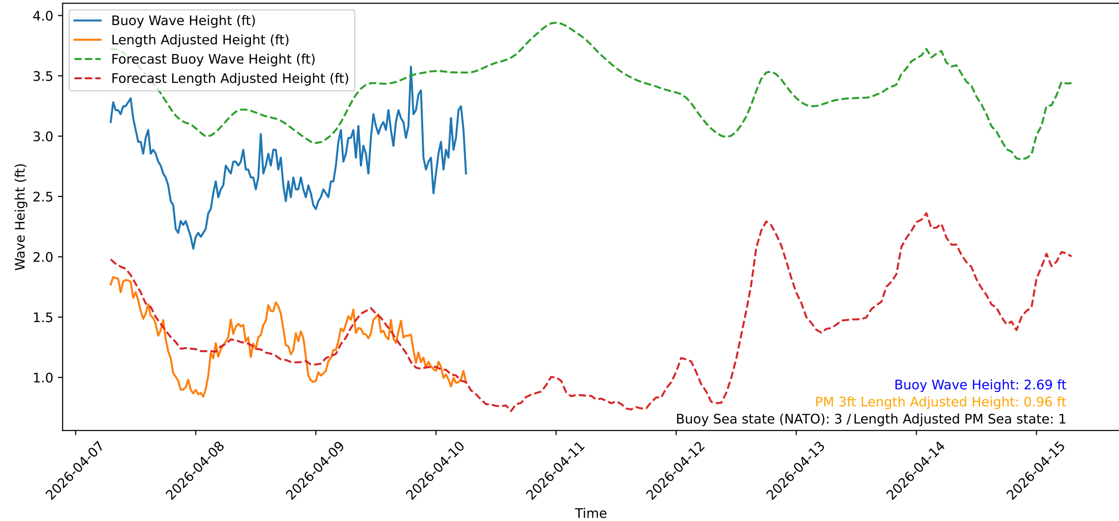
Wave Heights over Time for Red Beach at 2026-04-10 06:40:51
