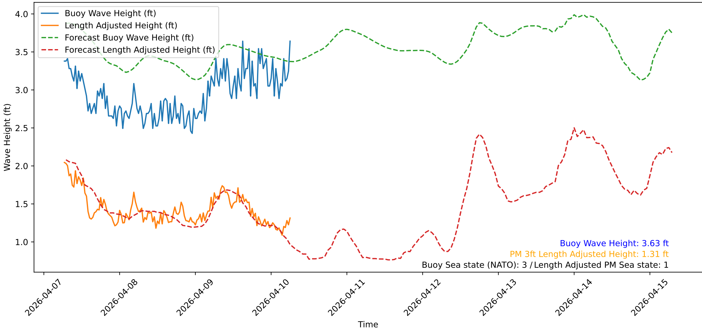
Wave Heights over Time for Oceanside Harbor at 2026-04-10 06:40:32
