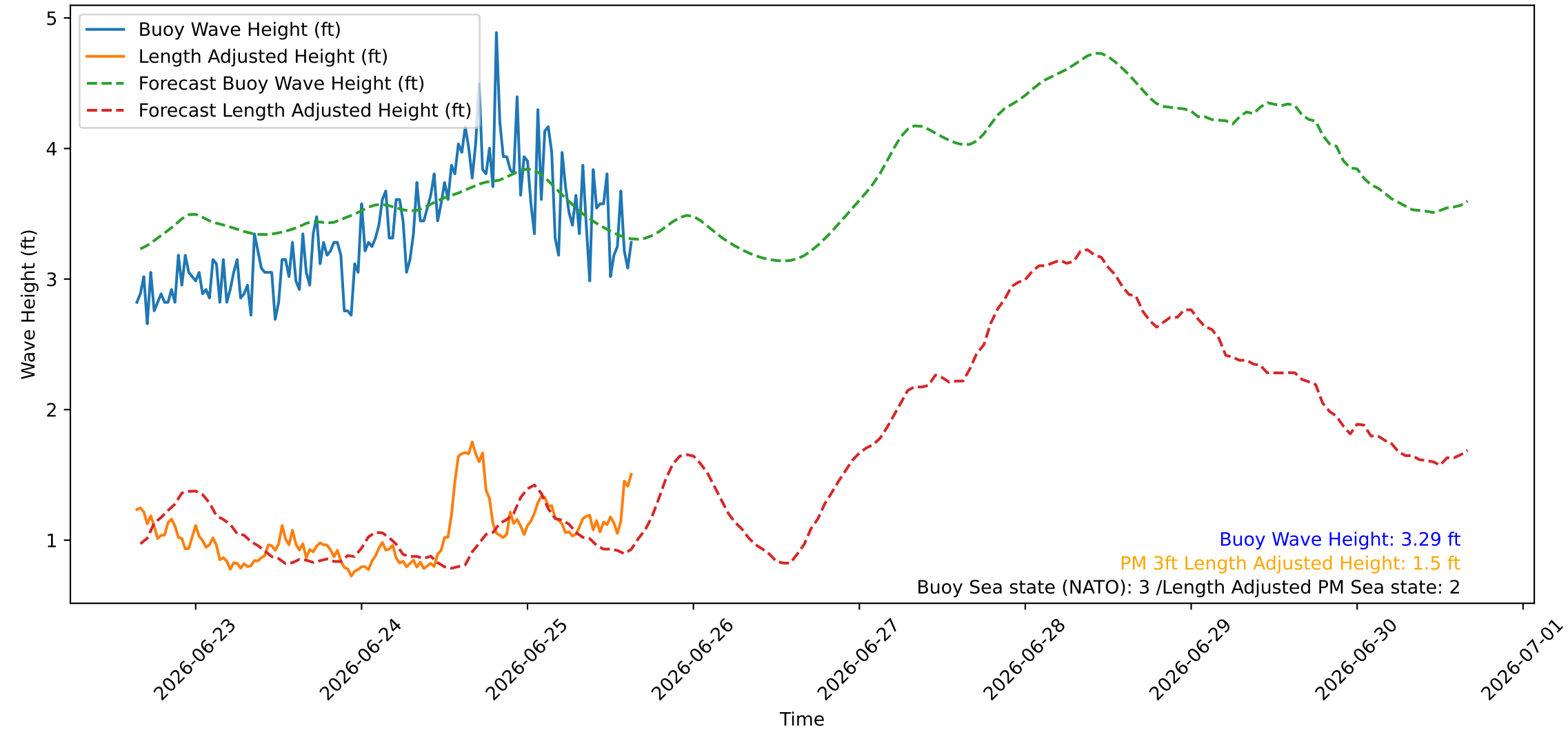
Wave Heights over Time for Oceanside Harbor at 2026-06-25 15:40:26
