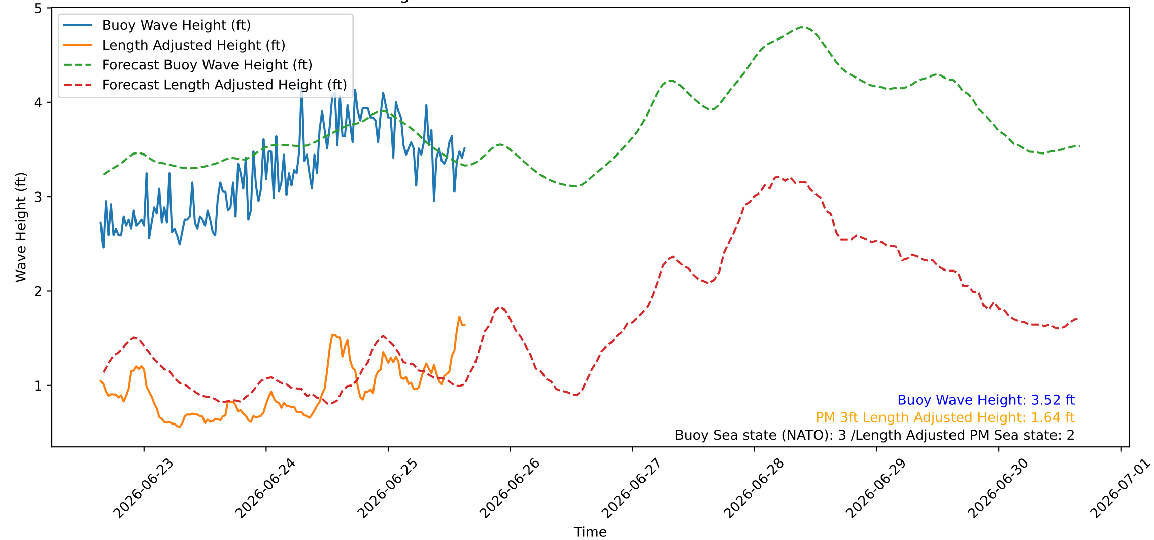
Wave Heights over Time for Green Beach at 2026-06-25 15:41:08
