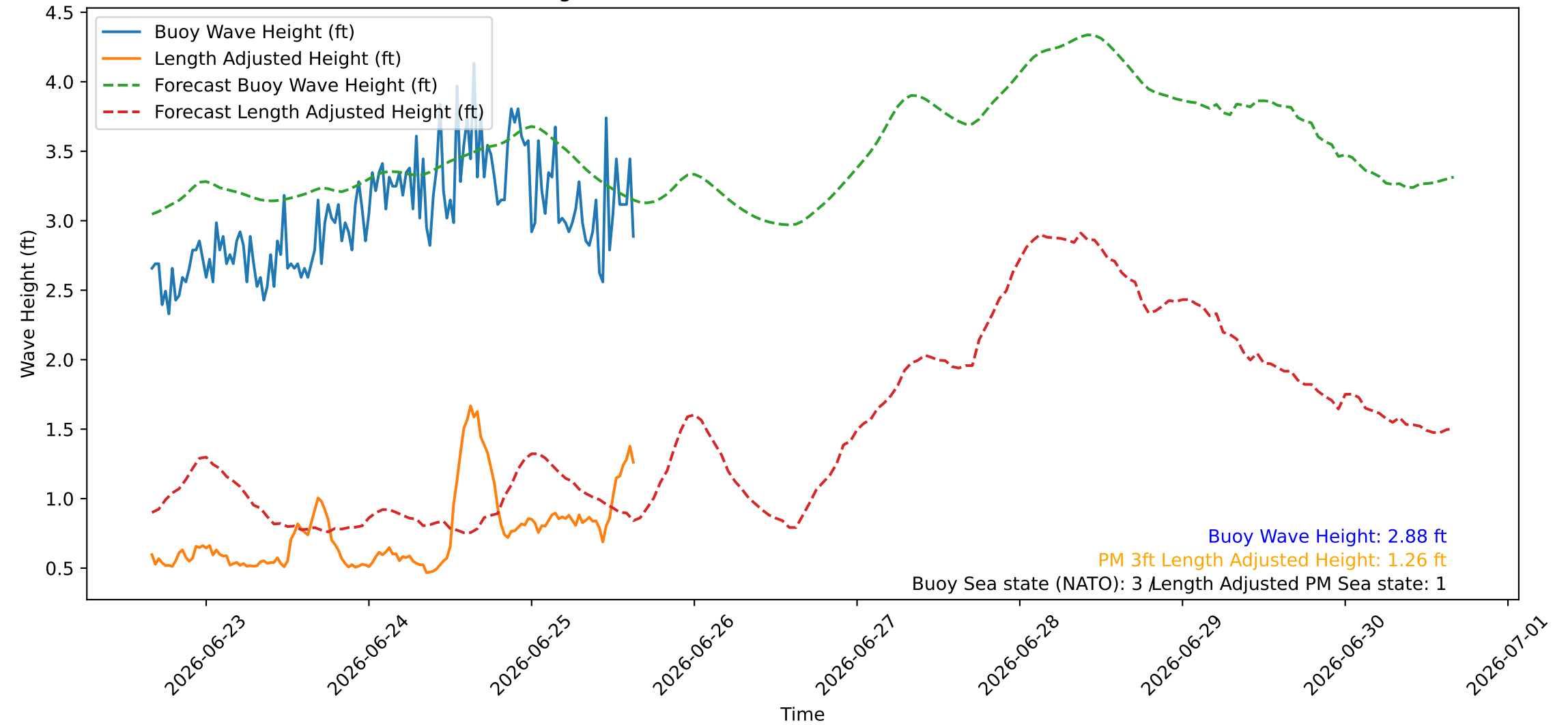
Wave Heights over Time for Red Beach at 2026-06-25 15:40:45
