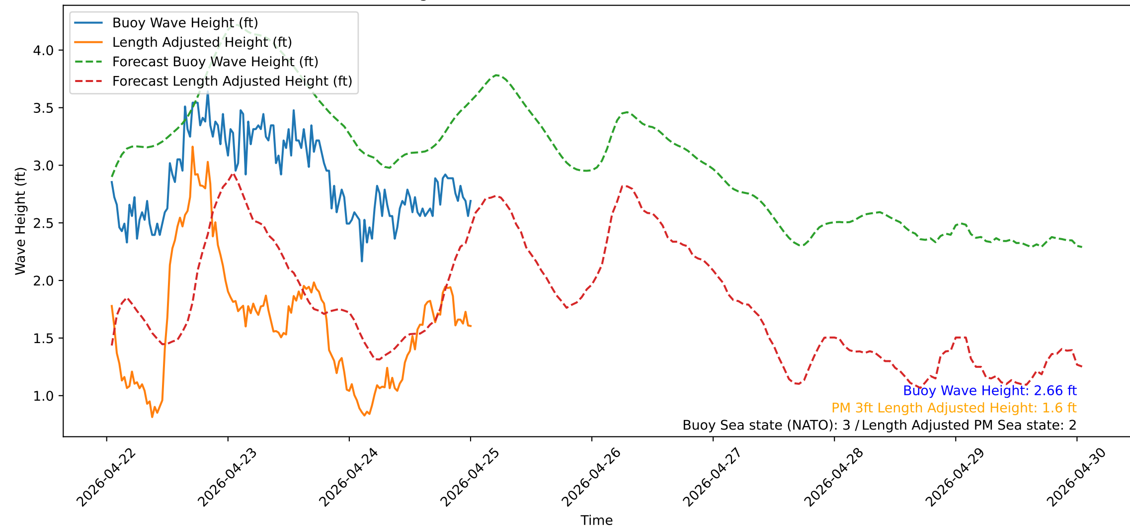
Wave Heights over Time for Red Beach at 2026-04-25 00:40:51
