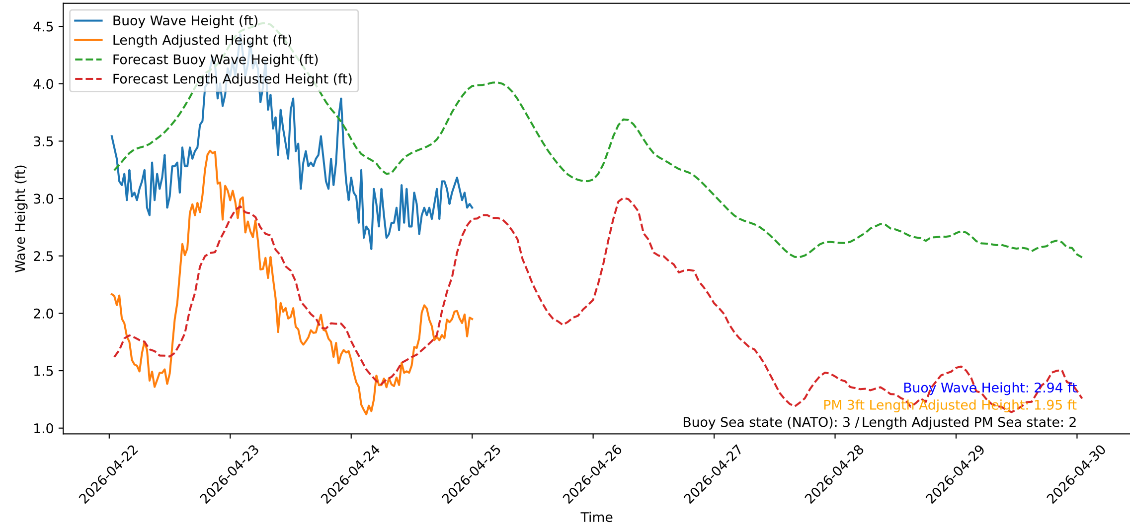
Wave Heights over Time for Oceanside Harbor at 2026-04-25 00:40:31
