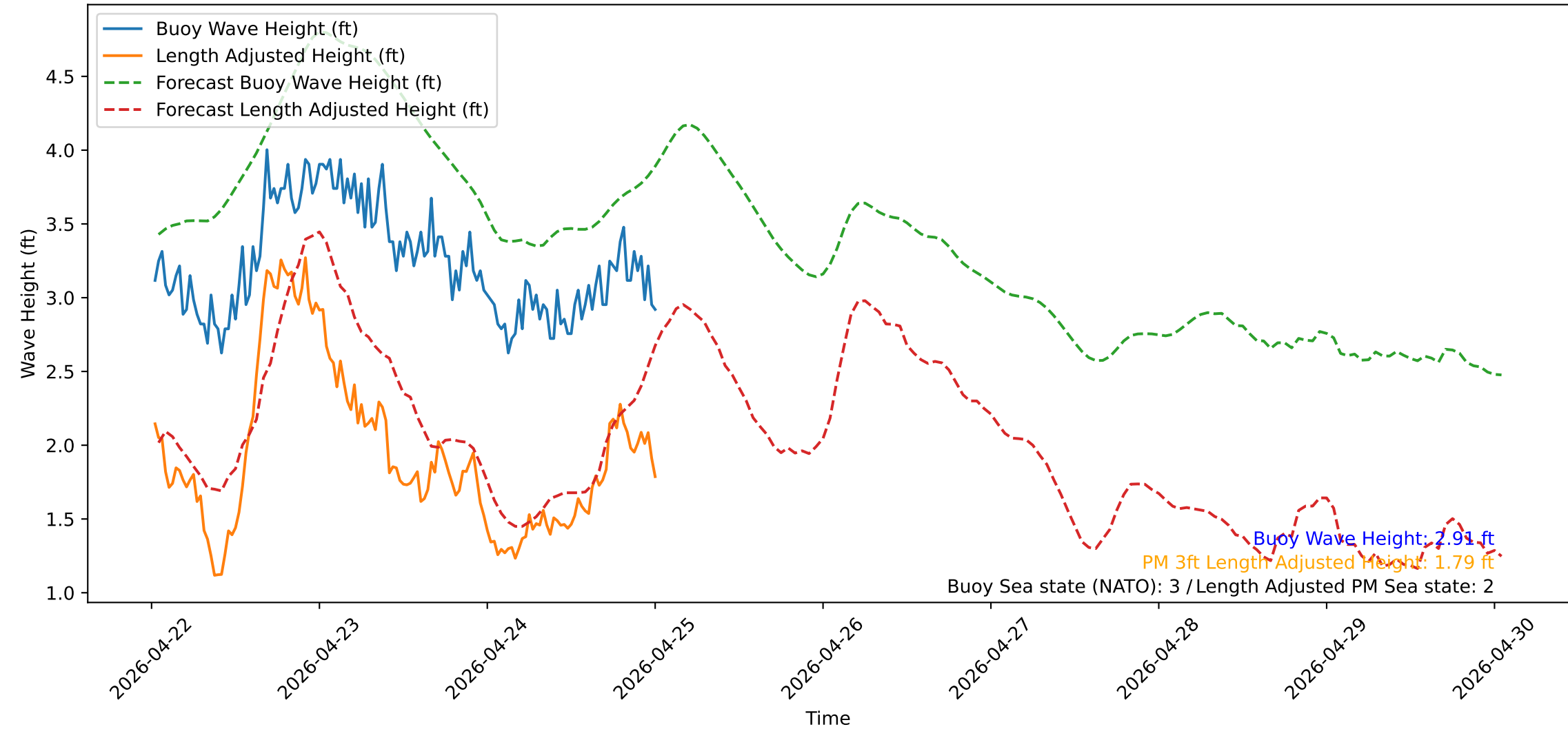
Wave Heights over Time for Green Beach at 2026-04-25 00:41:13
