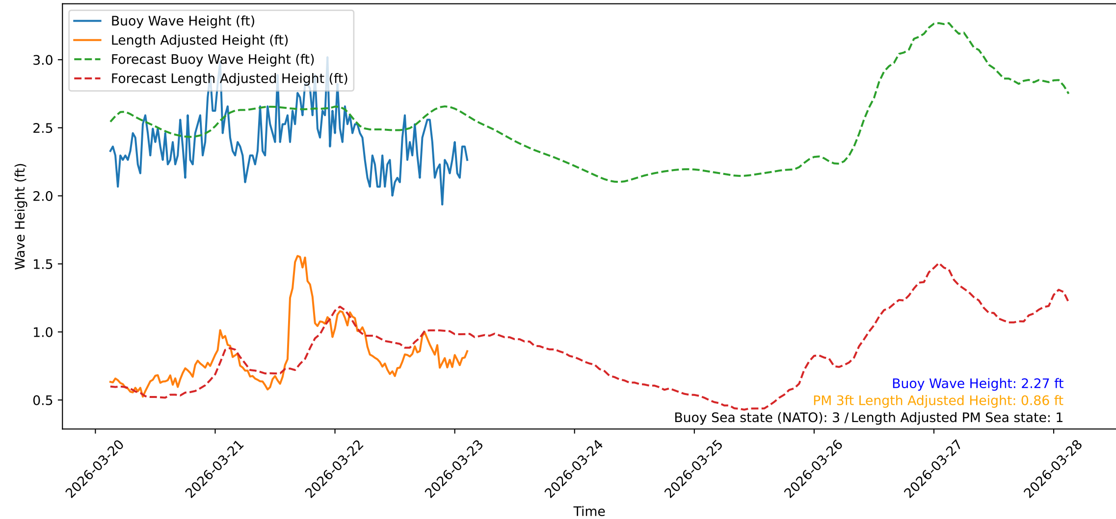
Wave Heights over Time for Oceanside Harbor at 2026-03-23 03:10:31
