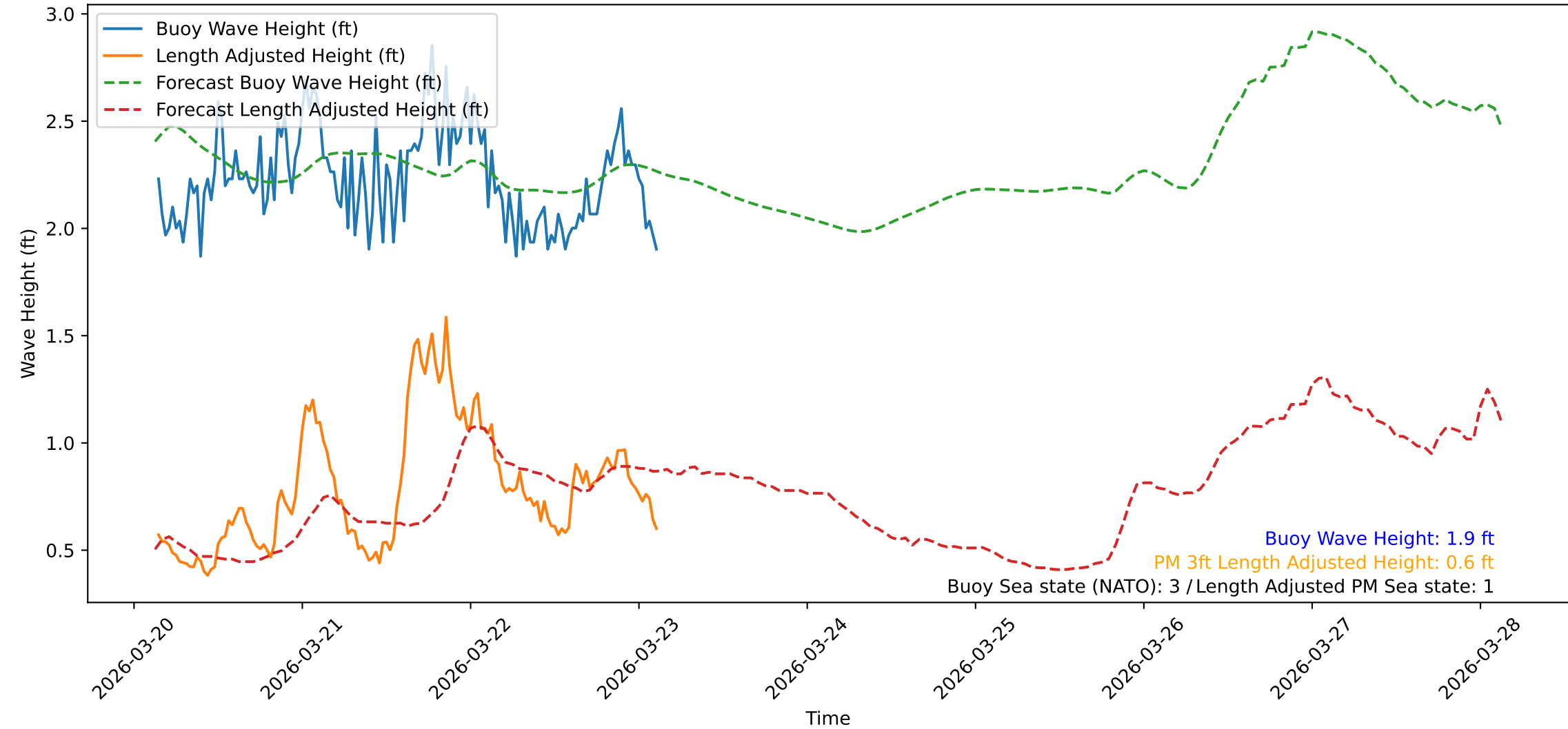
Wave Heights over Time for Red Beach at 2026-03-23 03:10:47
