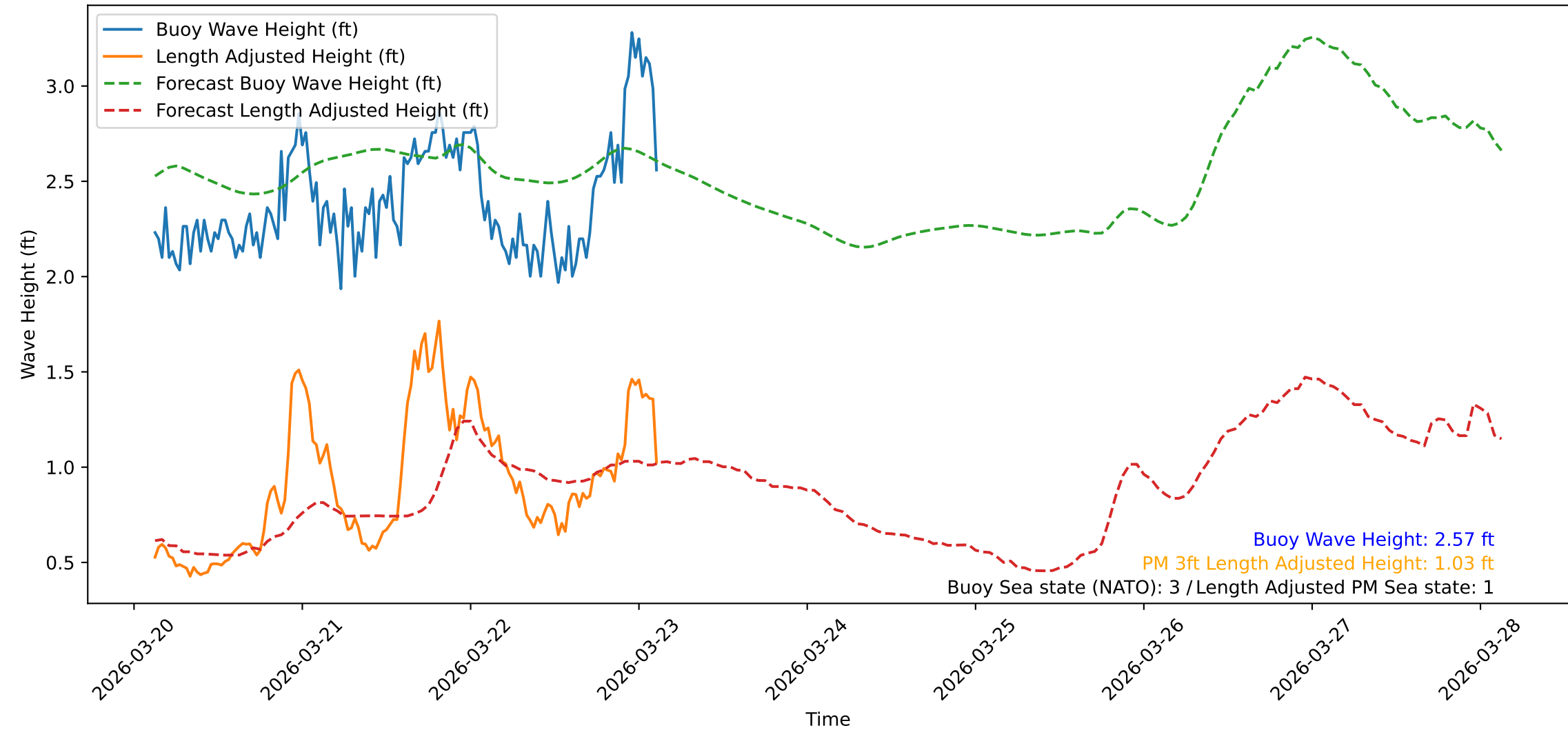
Wave Heights over Time for Green Beach at 2026-03-23 03:11:09
