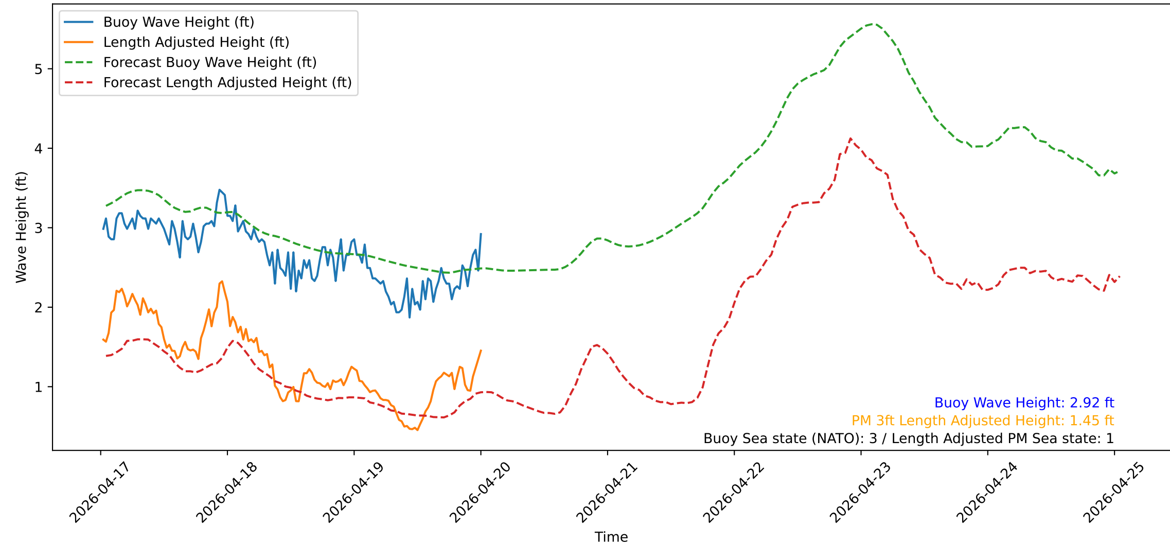
Wave Heights over Time for Green Beach at 2026-04-20 00:41:12
