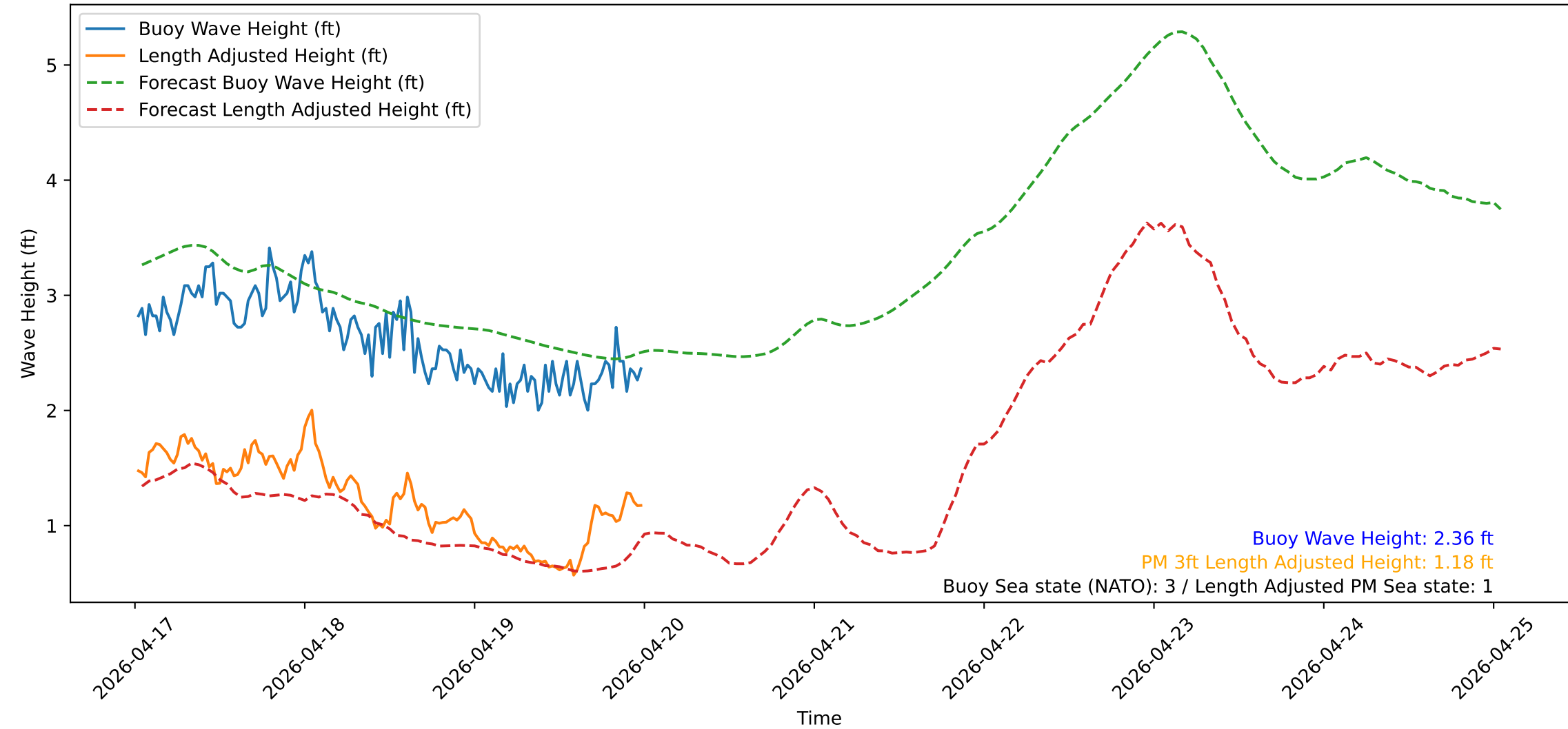
Wave Heights over Time for Oceanside Harbor at 2026-04-20 00:40:31
