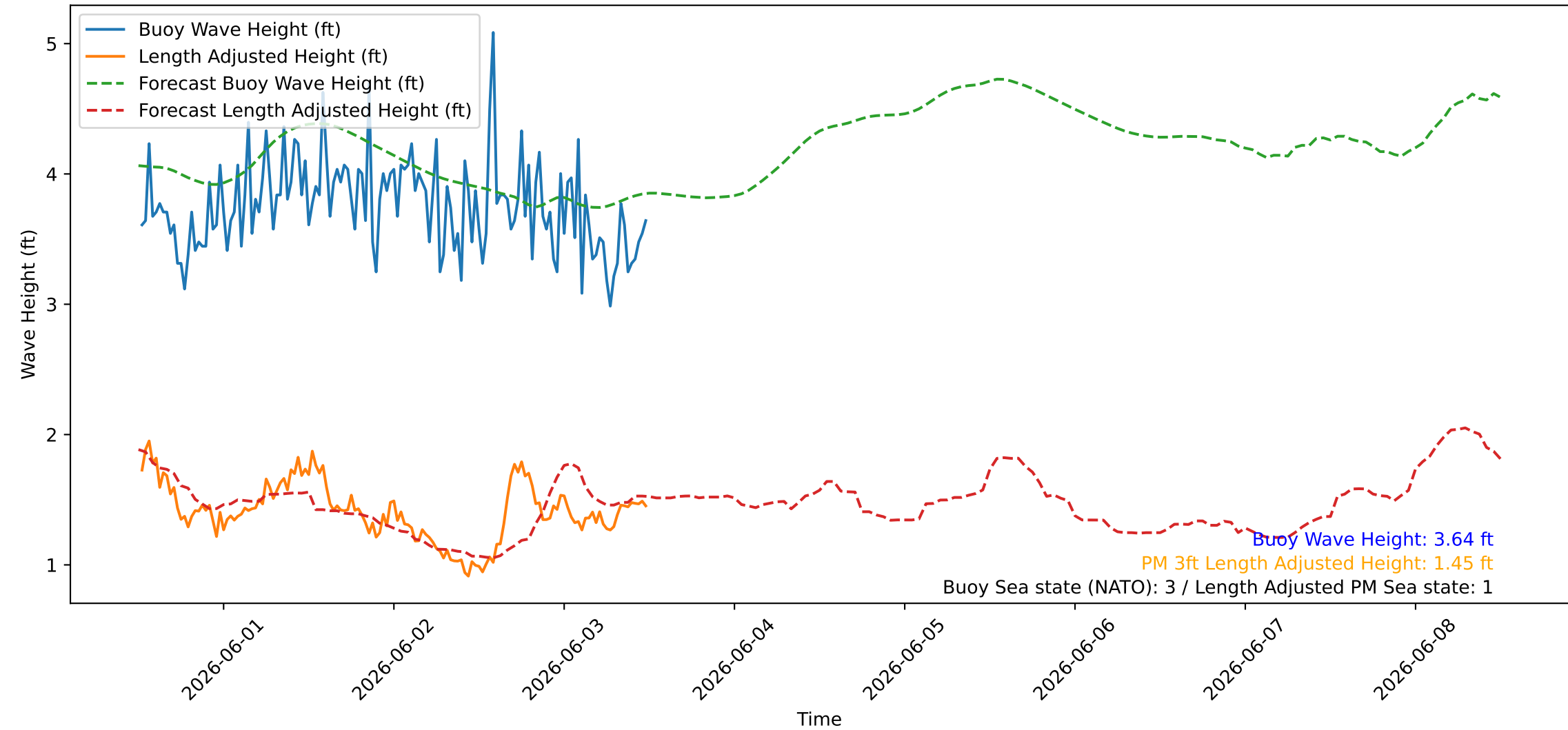
Wave Heights over Time for Oceanside Harbor at 2026-06-03 12:20:26
