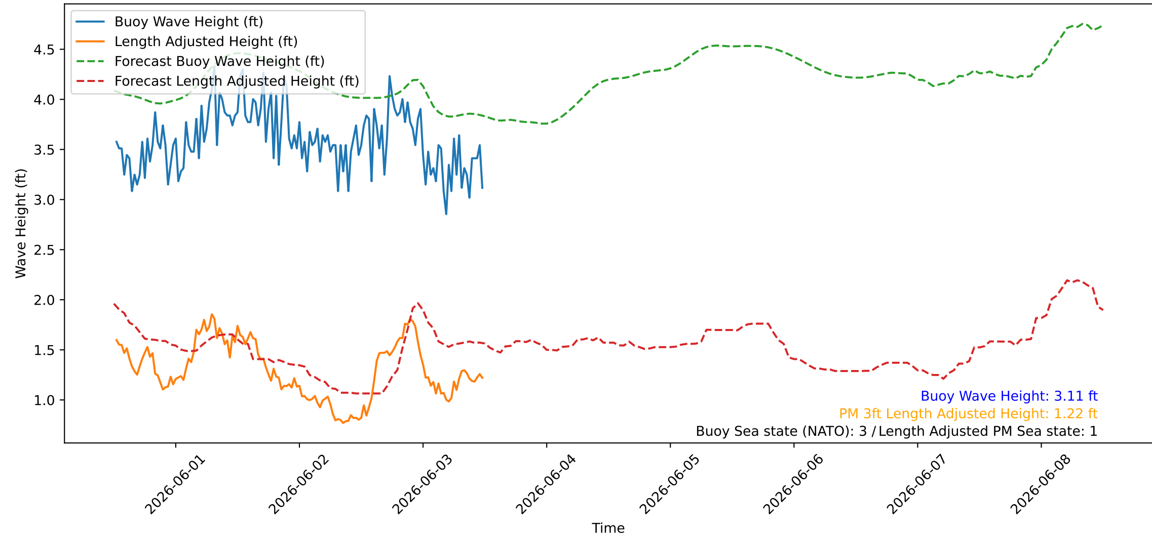
Wave Heights over Time for Green Beach at 2026-06-03 12:21:10
