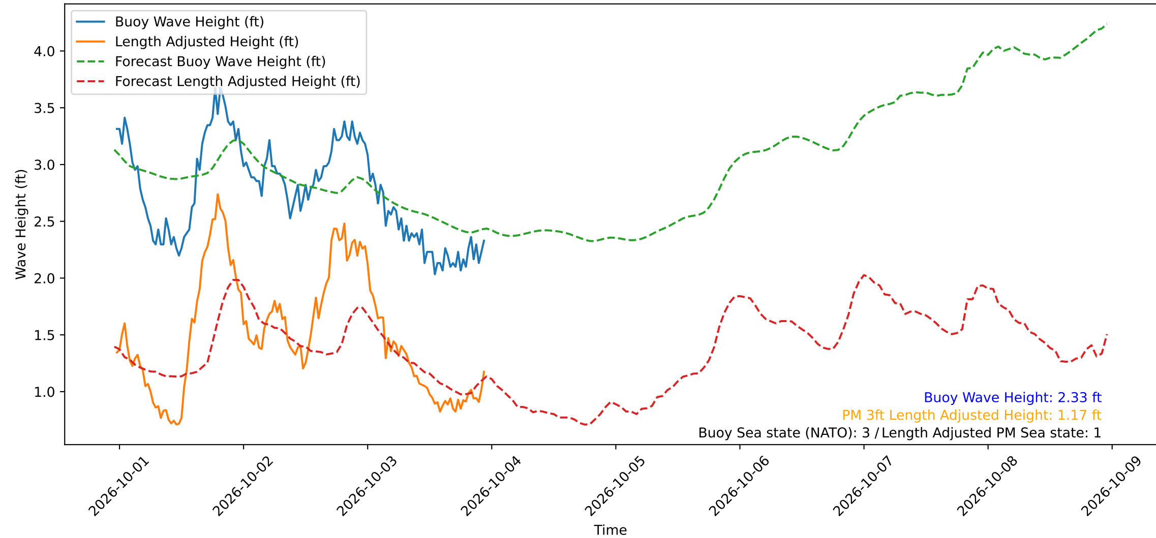
Wave Heights over Time for Green Beach at 2026-10-03 23:21:15
