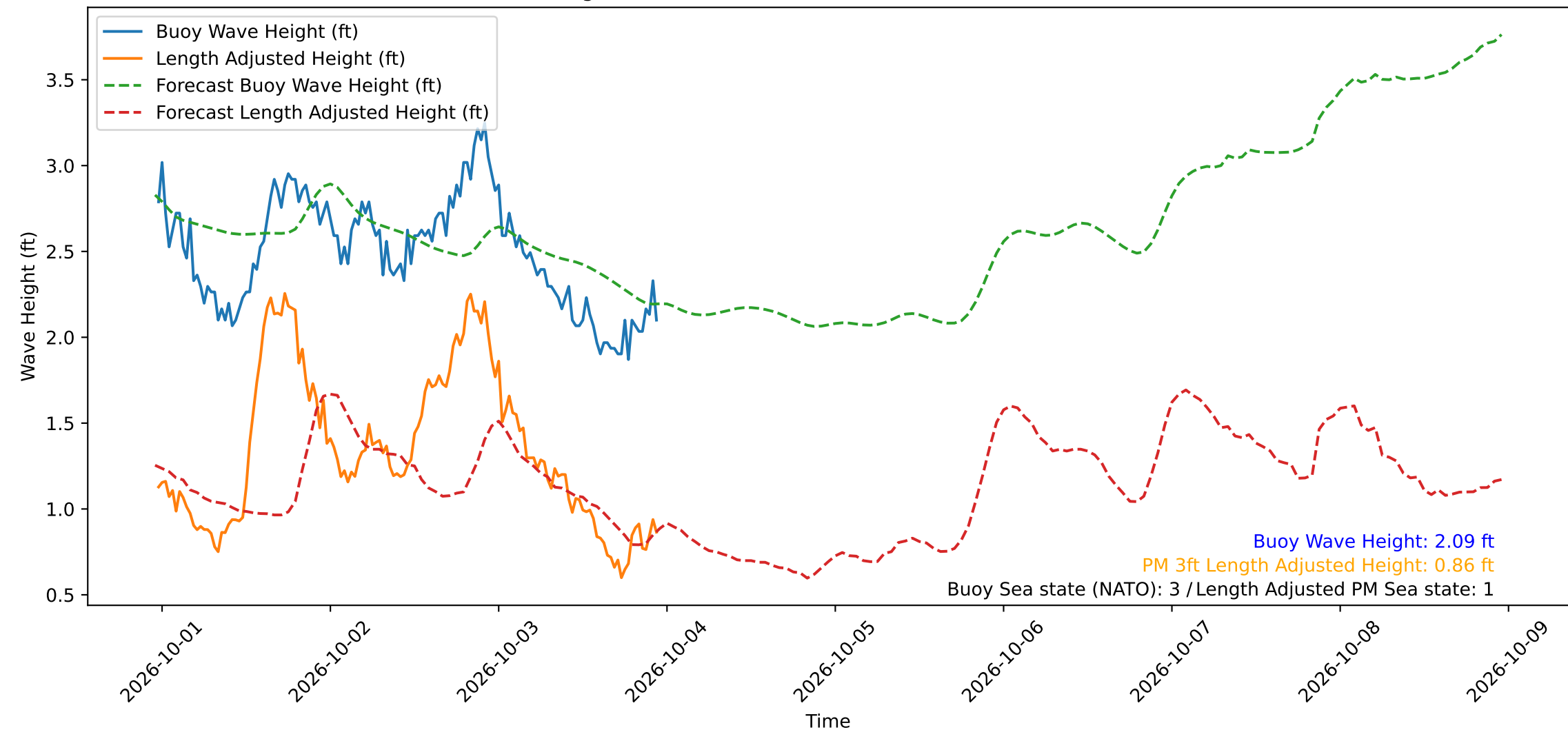
Wave Heights over Time for Red Beach at 2026-10-03 23:20:51
