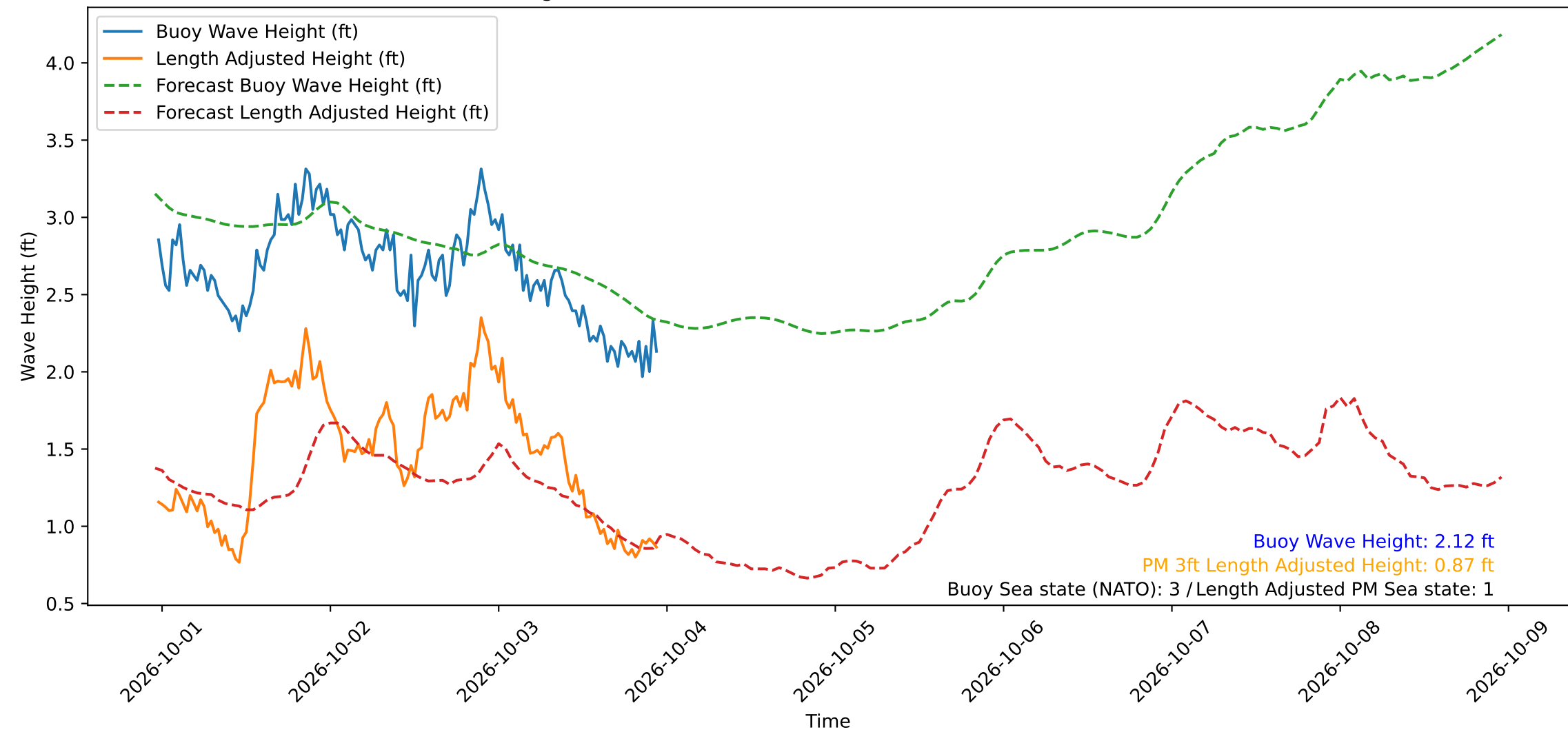
Wave Heights over Time for Oceanside Harbor at 2026-10-03 23:20:30
