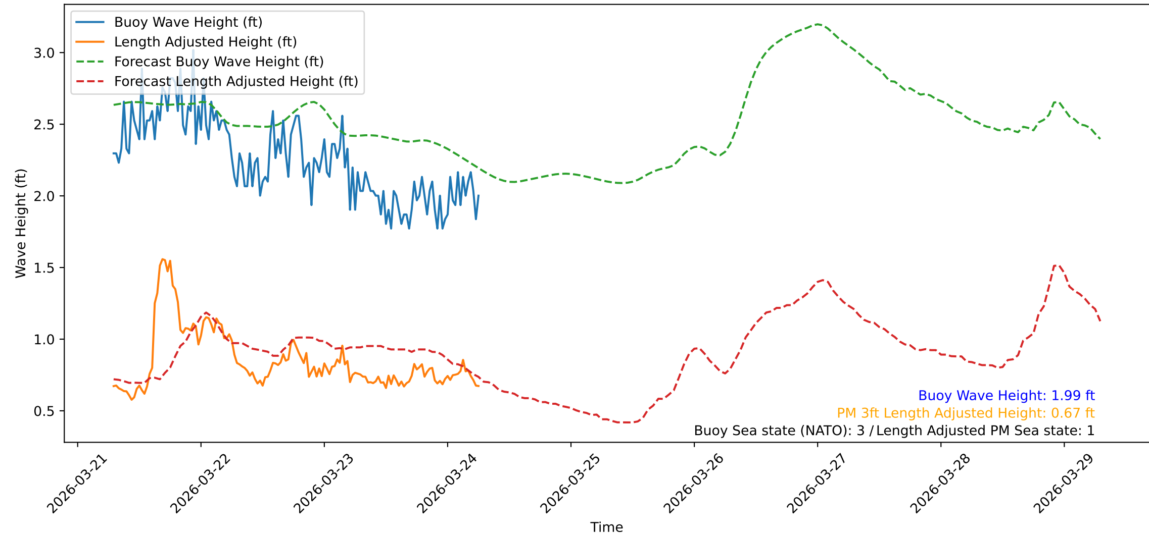
Wave Heights over Time for Oceanside Harbor at 2026-03-24 07:10:31
