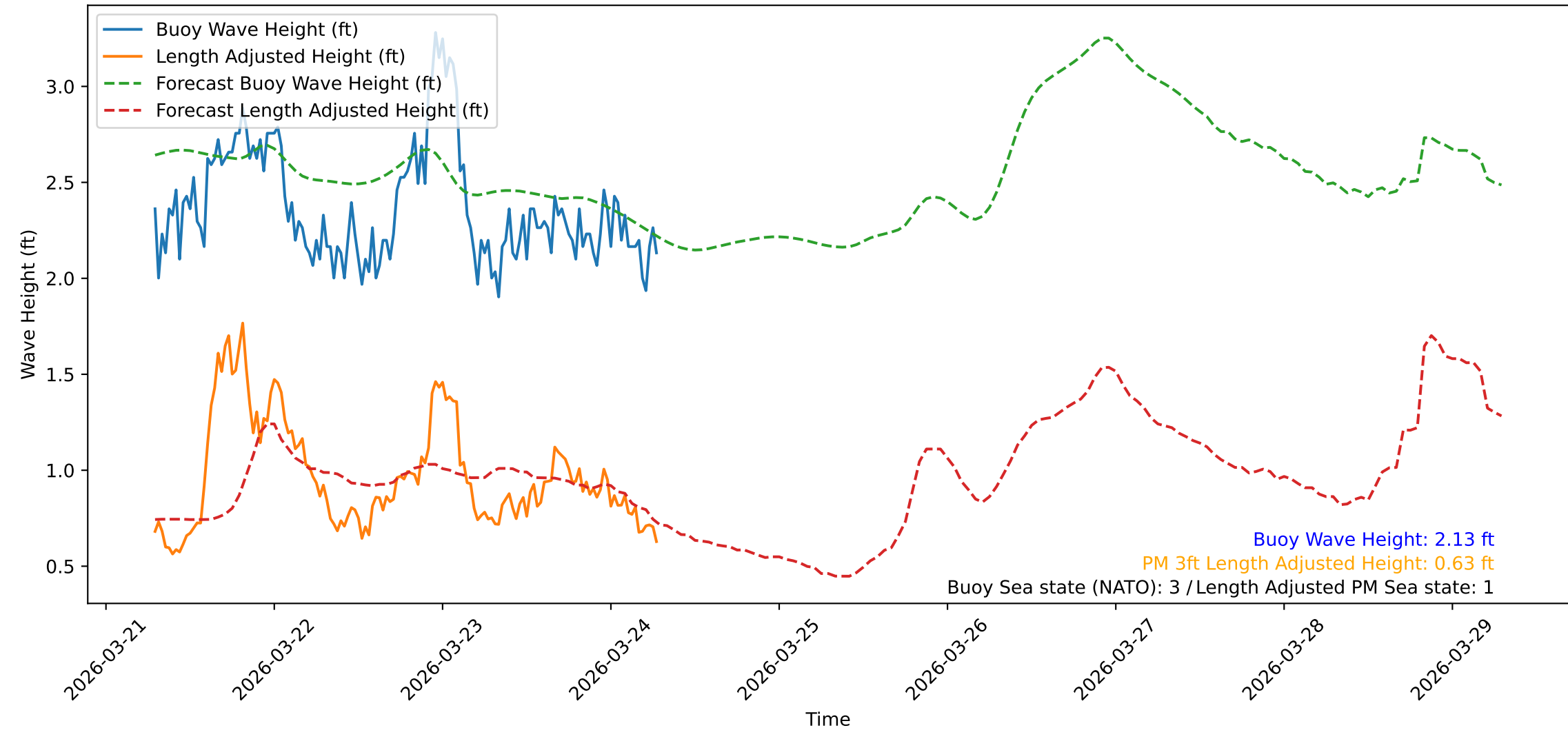
Wave Heights over Time for Green Beach at 2026-03-24 07:11:09
