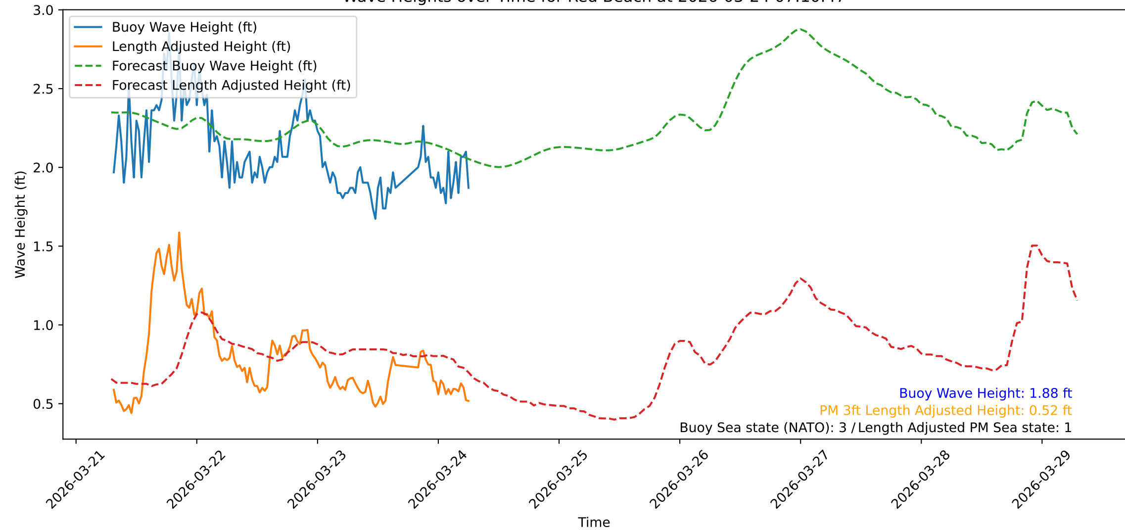
Wave Heights over Time for Red Beach at 2026-03-24 07:10:47
