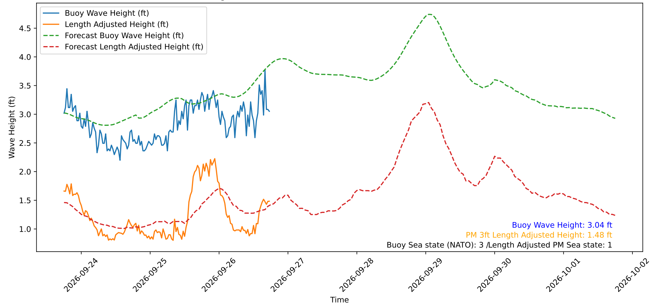
Wave Heights over Time for Oceanside Harbor at 2026-09-26 18:10:29
