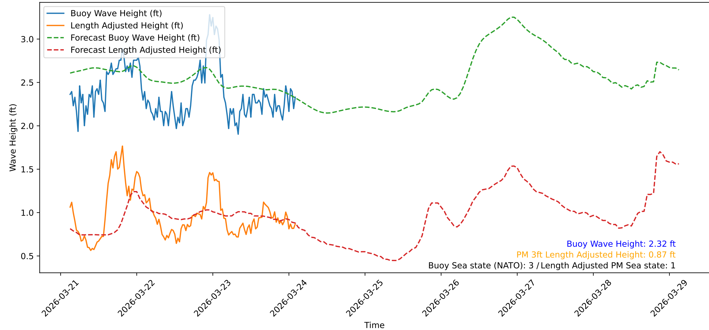
Wave Heights over Time for Green Beach at 2026-03-24 02:51:09
