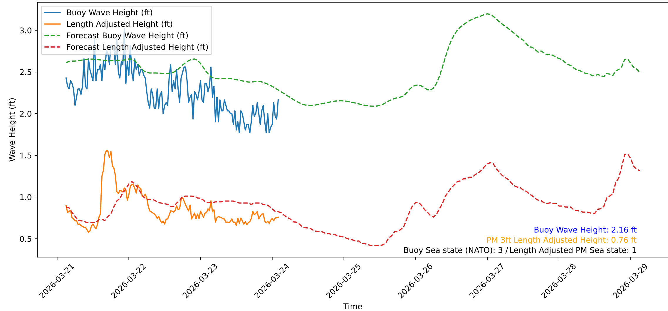
Wave Heights over Time for Oceanside Harbor at 2026-03-24 02:50:31
