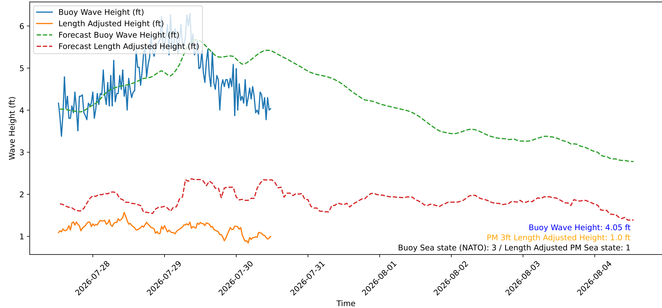
Wave Heights over Time for Green Beach at 2026-07-30 12:31:09
