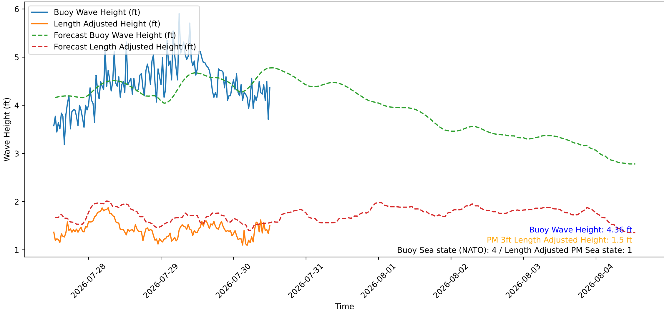
Wave Heights over Time for Oceanside Harbor at 2026-07-30 12:30:26
