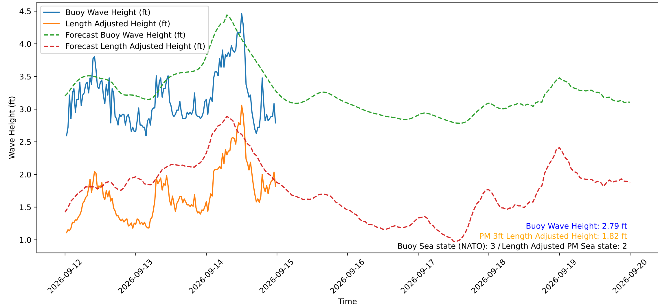
Wave Heights over Time for Oceanside Harbor at 2026-09-15 00:20:30
