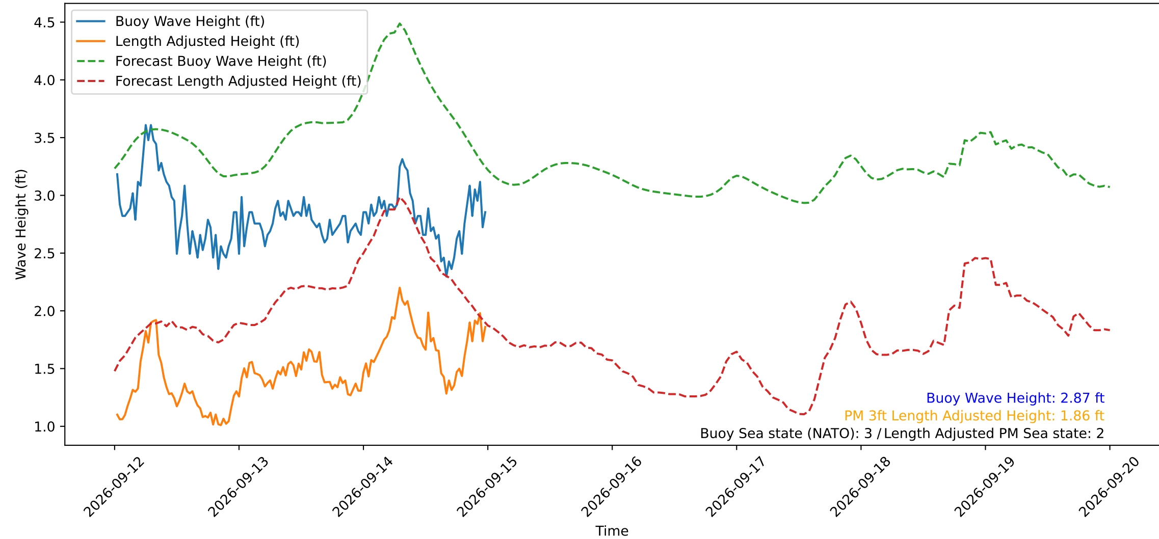
Wave Heights over Time for Green Beach at 2026-09-15 00:21:15
