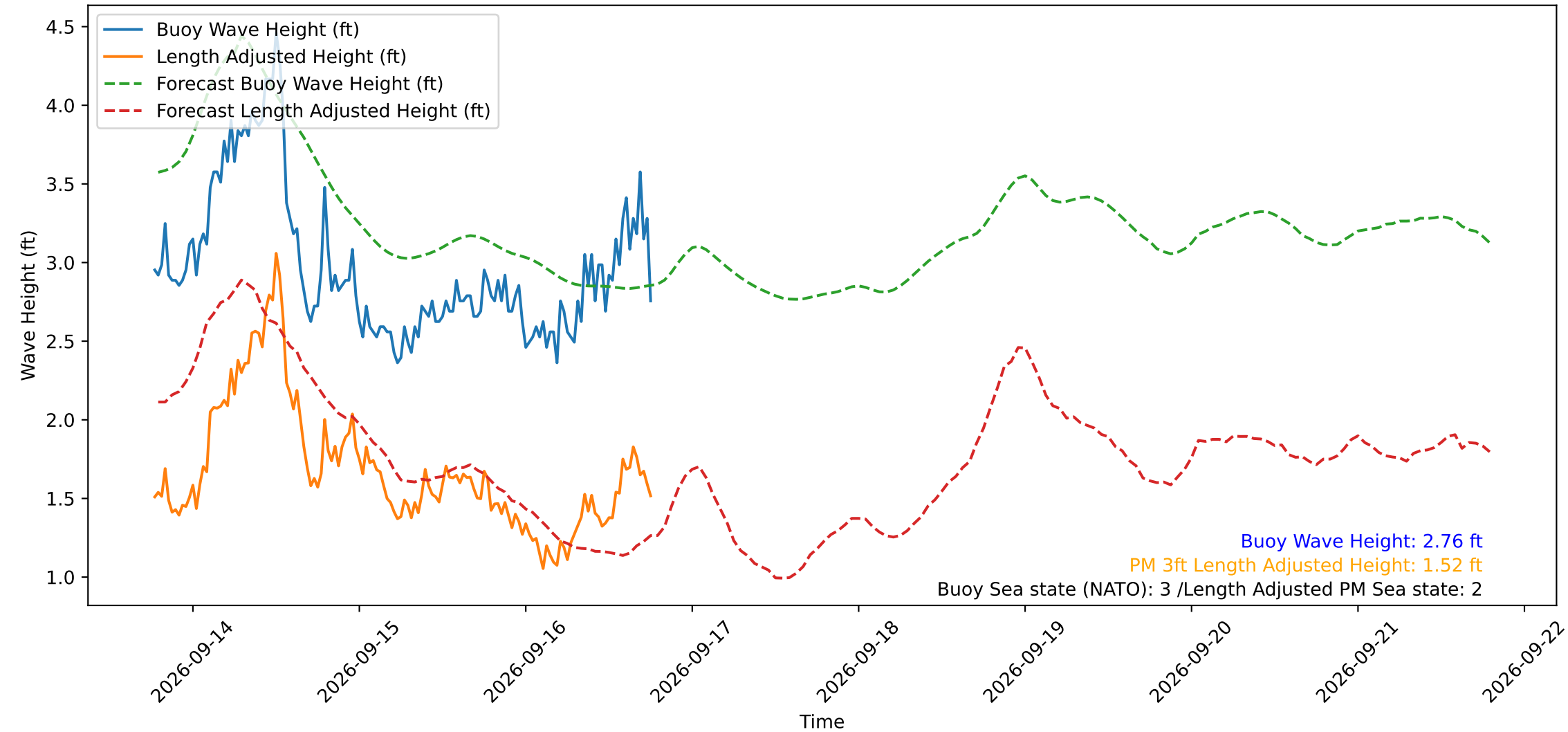
Wave Heights over Time for Oceanside Harbor at 2026-09-16 18:40:29
