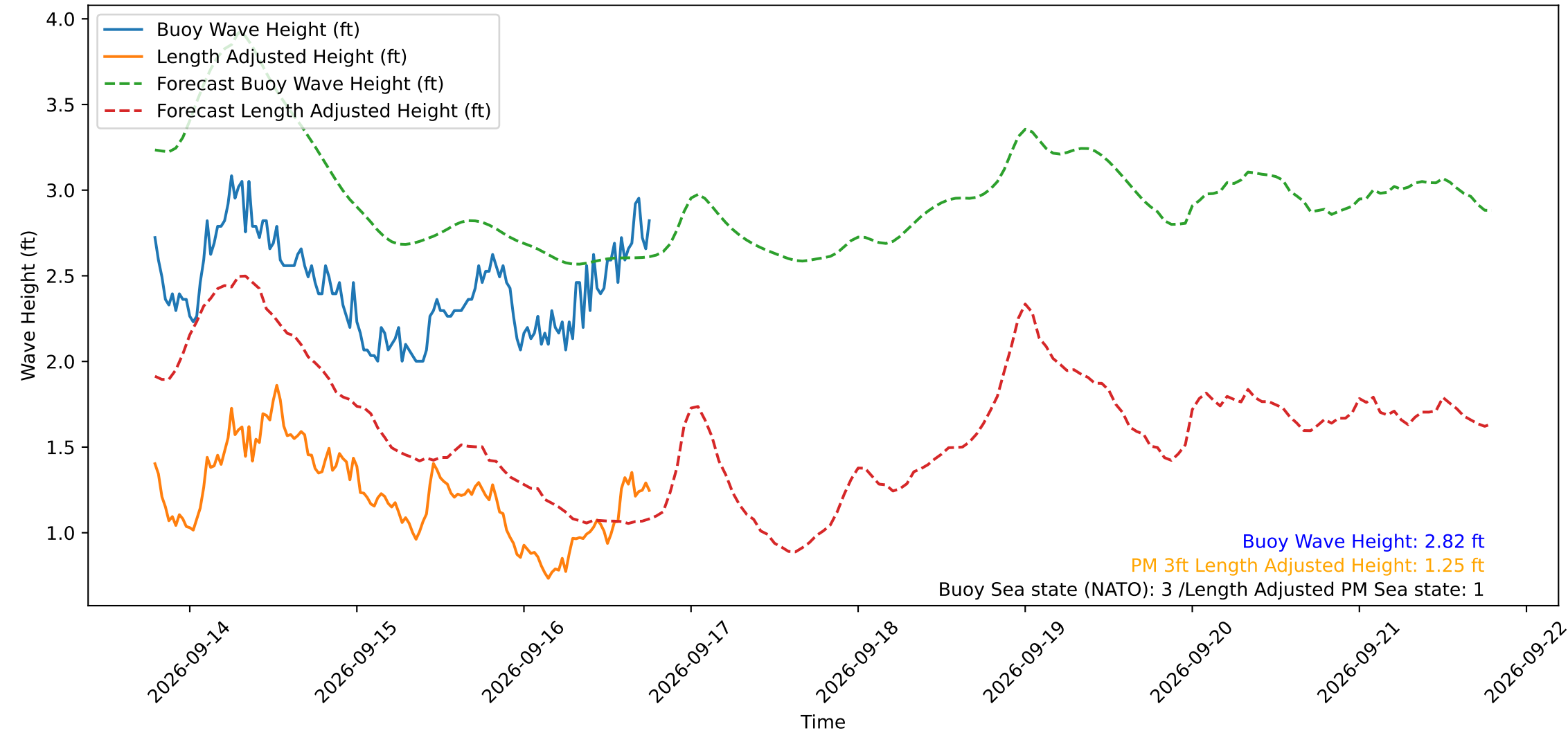
Wave Heights over Time for Red Beach at 2026-09-16 18:40:49
