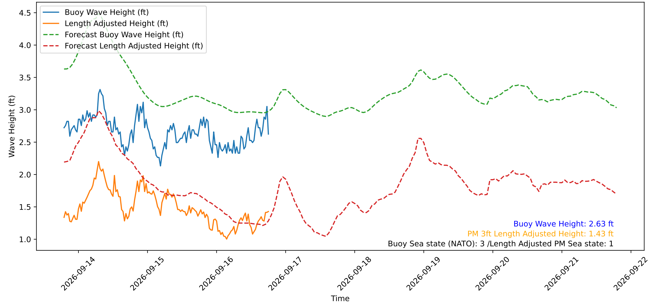
Wave Heights over Time for Green Beach at 2026-09-16 18:41:12
