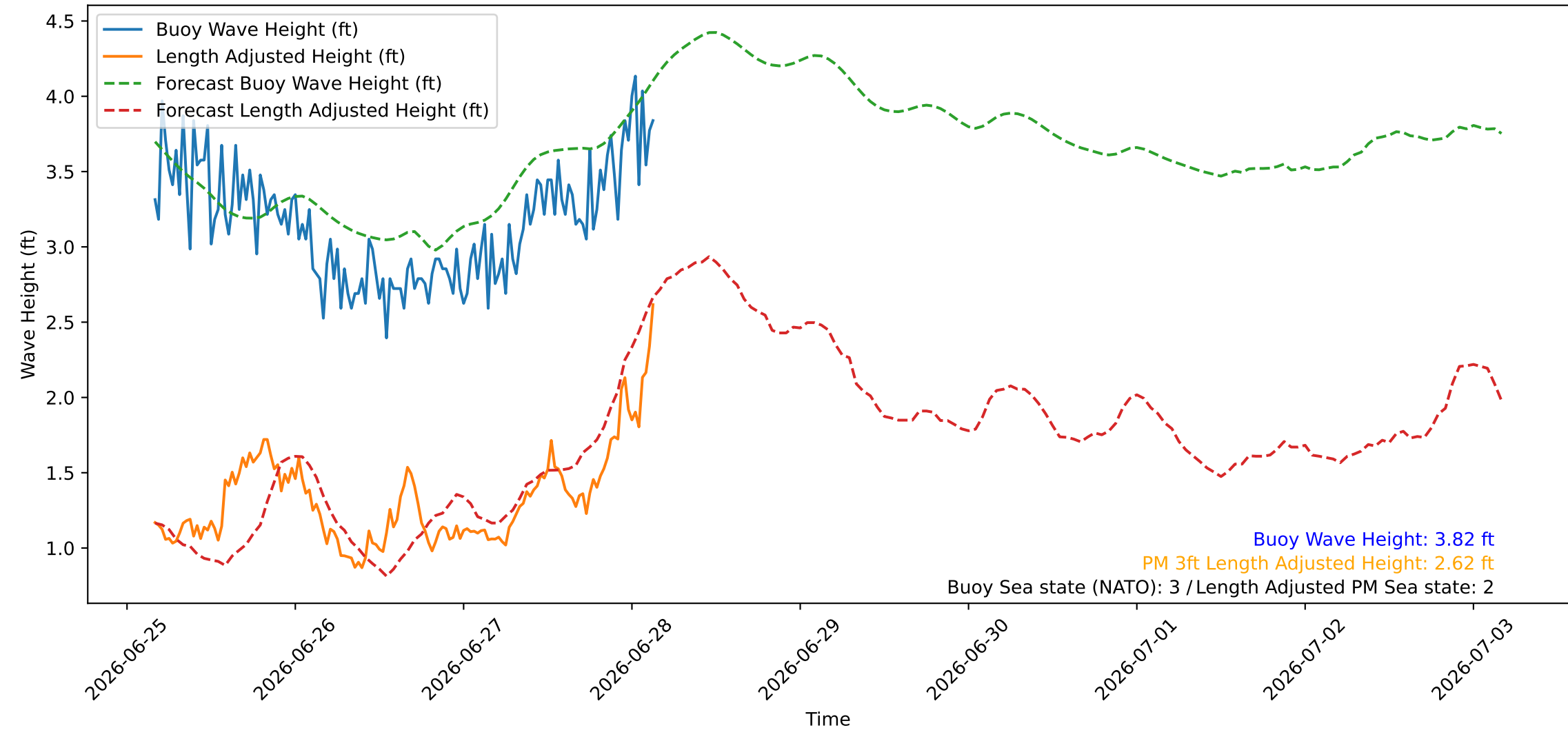
Wave Heights over Time for Oceanside Harbor at 2026-06-28 04:00:25
