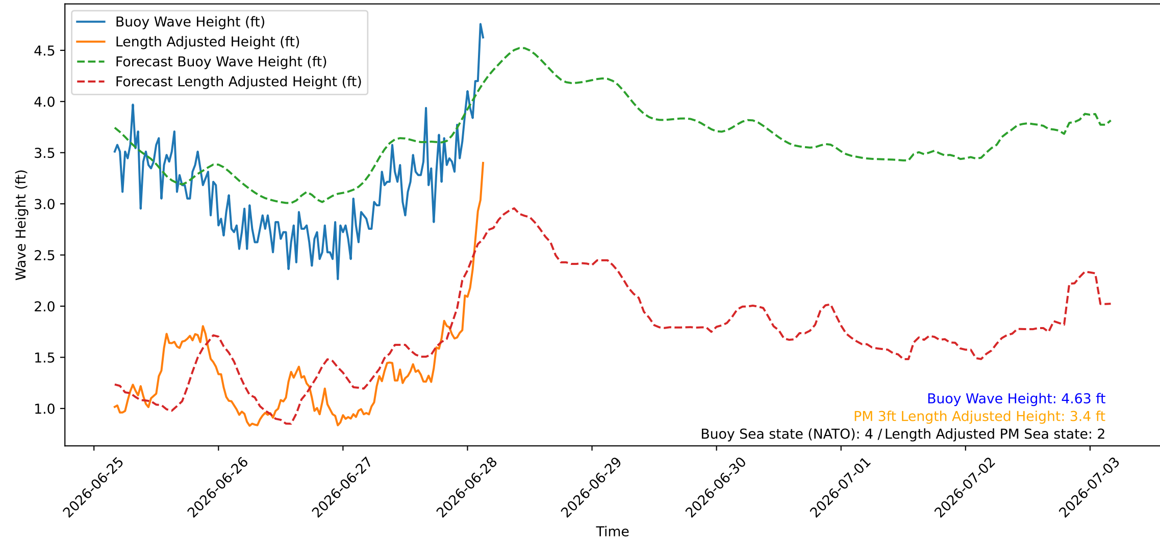
Wave Heights over Time for Green Beach at 2026-06-28 04:01:07
