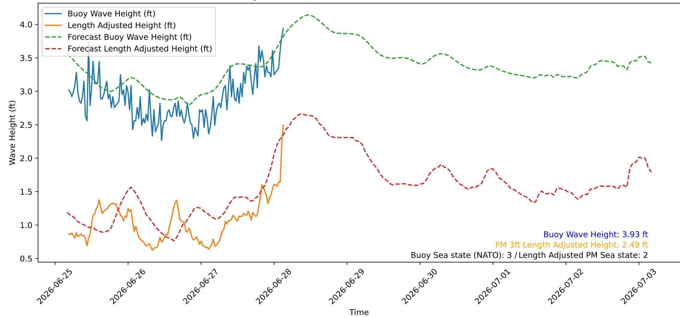
Wave Heights over Time for Red Beach at 2026-06-28 04:00:44
