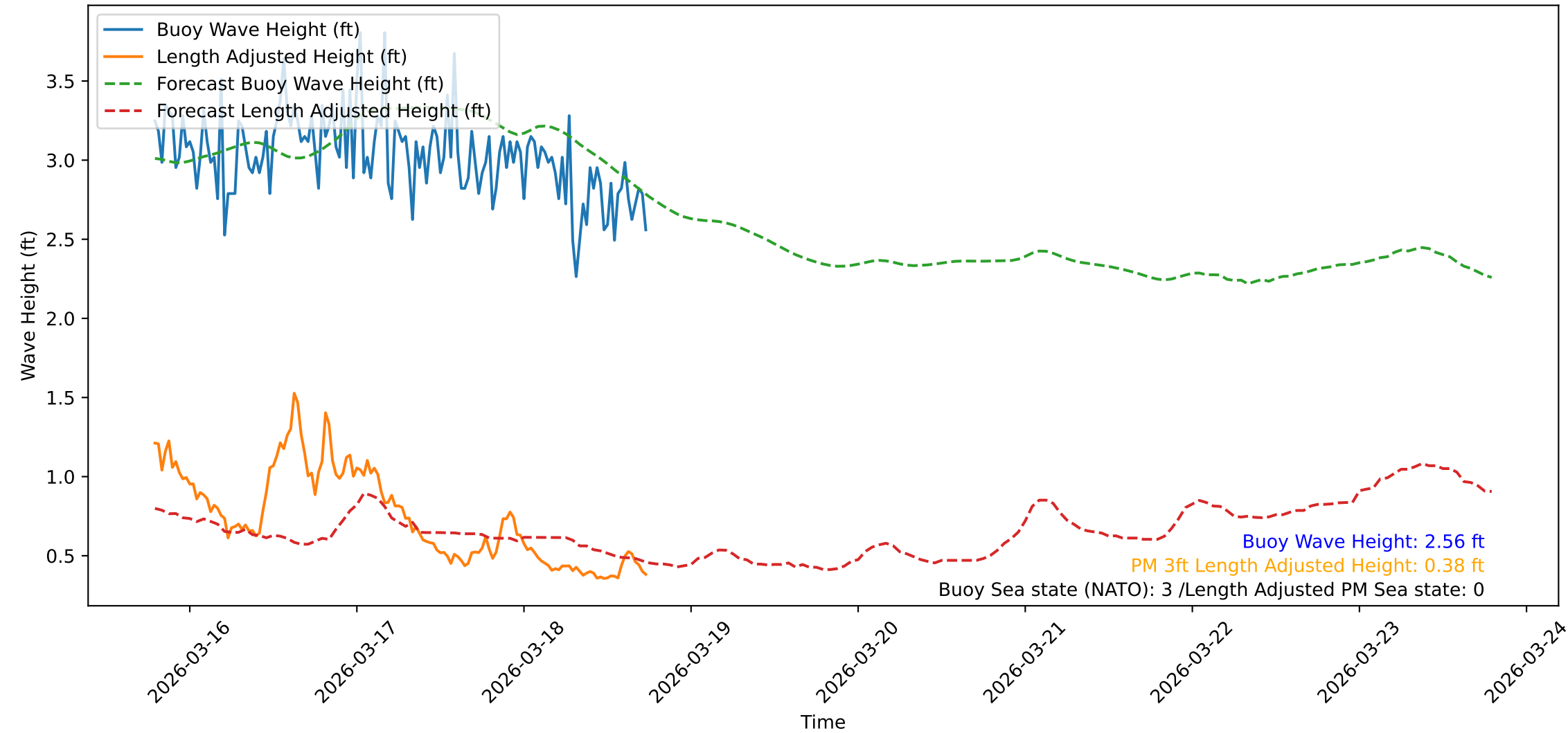
Wave Heights over Time for Red Beach at 2026-03-18 18:30:47
