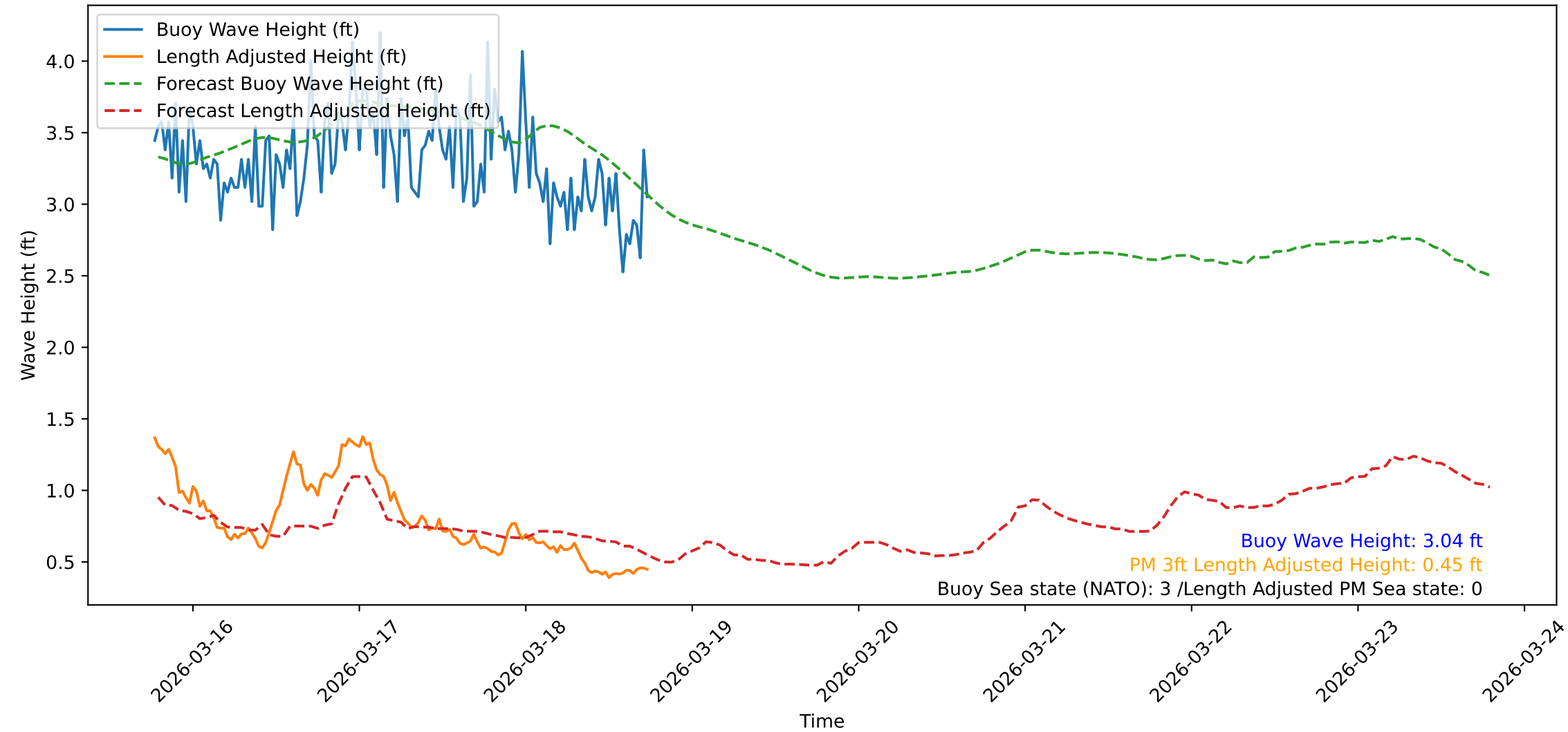
Wave Heights over Time for Green Beach at 2026-03-18 18:31:10
