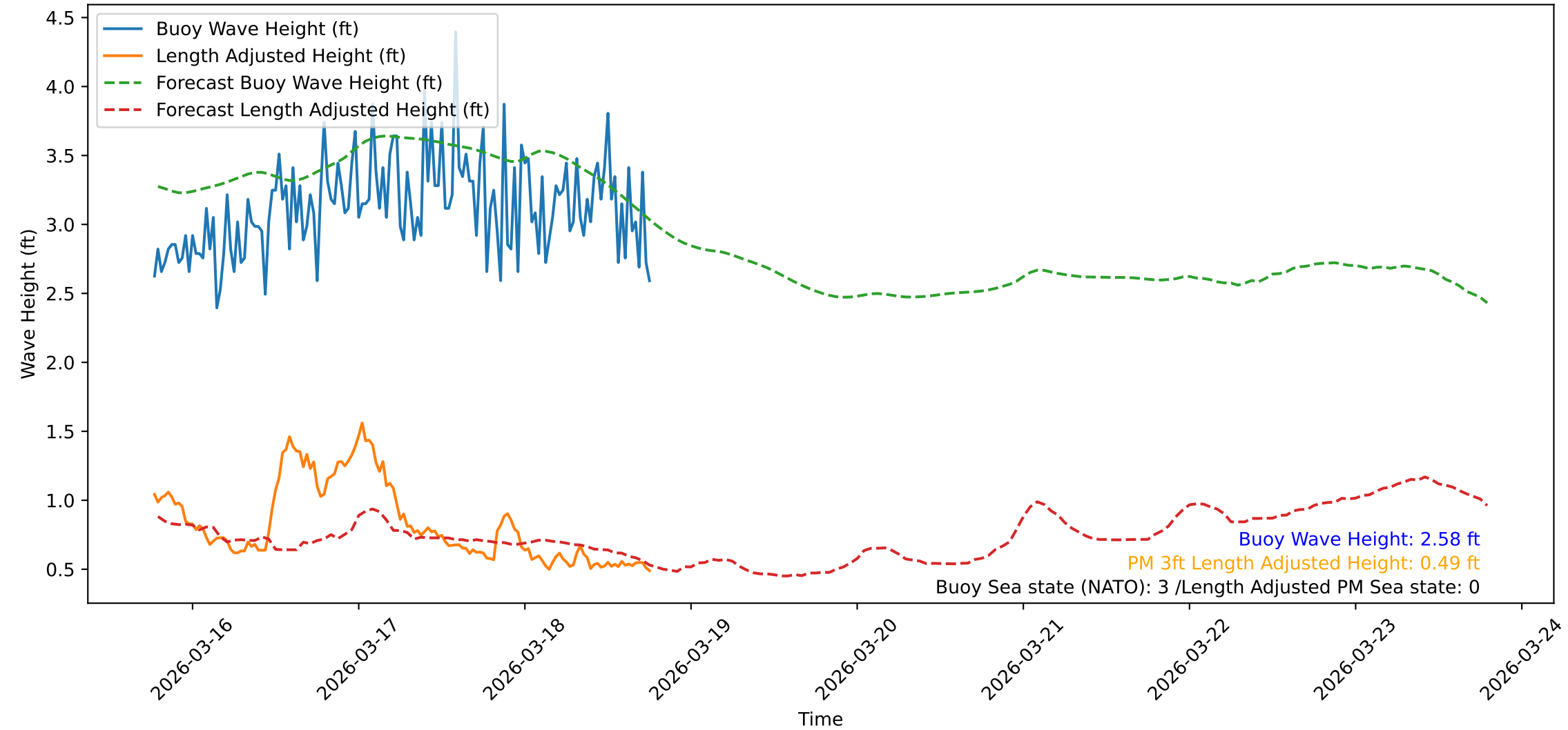
Wave Heights over Time for Oceanside Harbor at 2026-03-18 18:30:31
