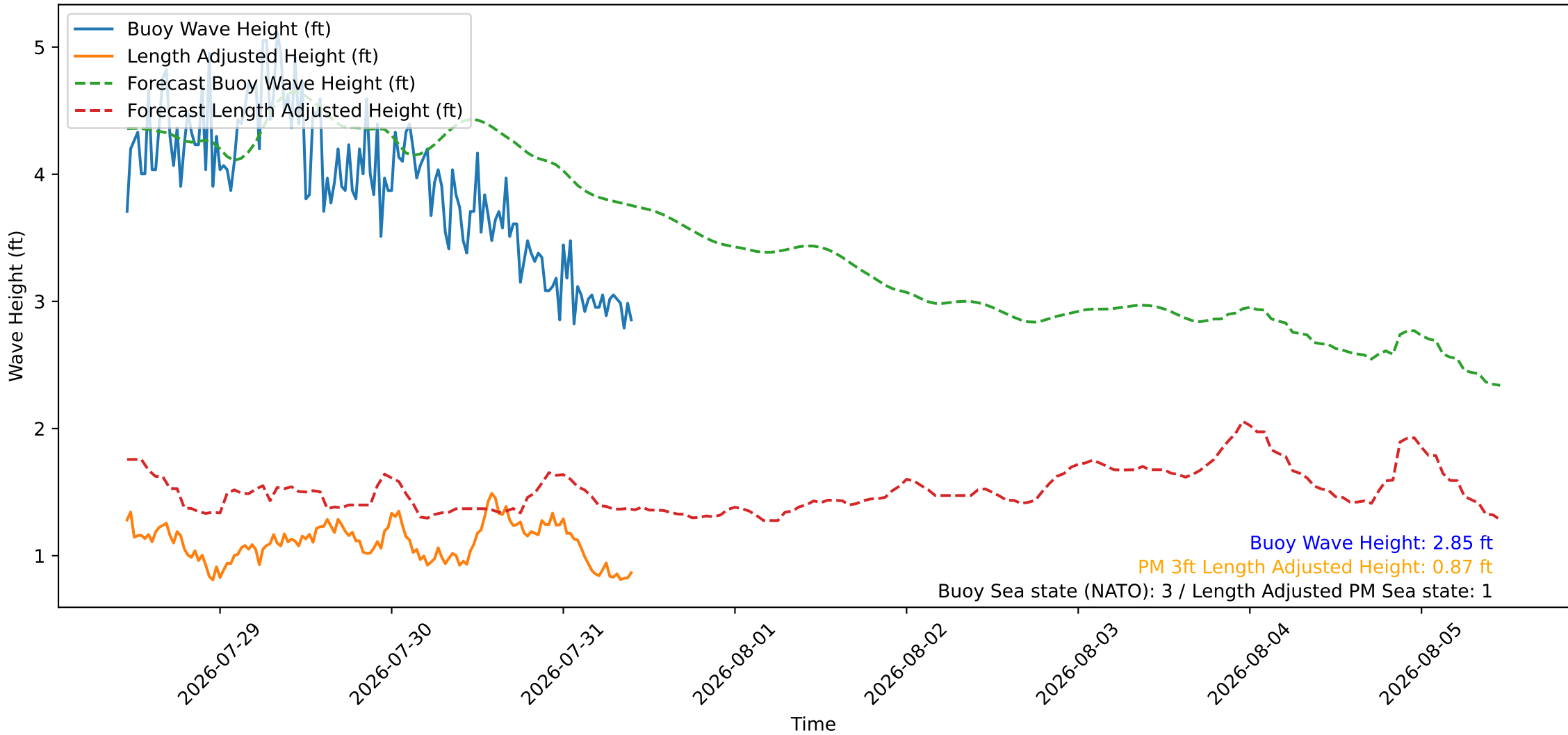
Wave Heights over Time for Red Beach at 2026-07-31 10:50:47
