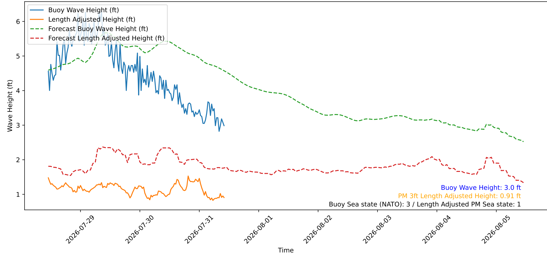
Wave Heights over Time for Green Beach at 2026-07-31 10:51:10
