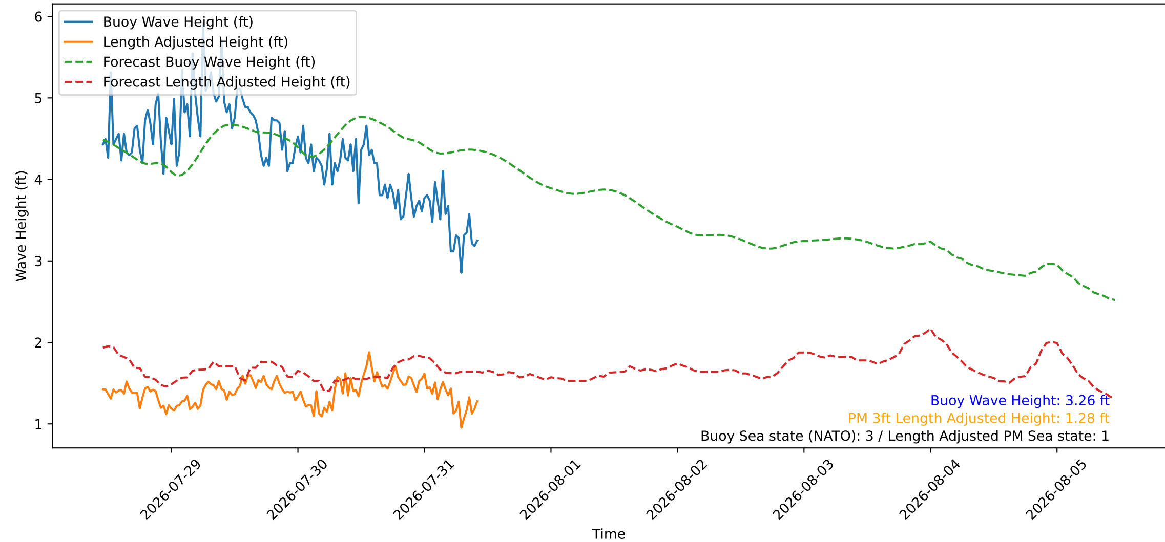
Wave Heights over Time for Oceanside Harbor at 2026-07-31 10:50:26
