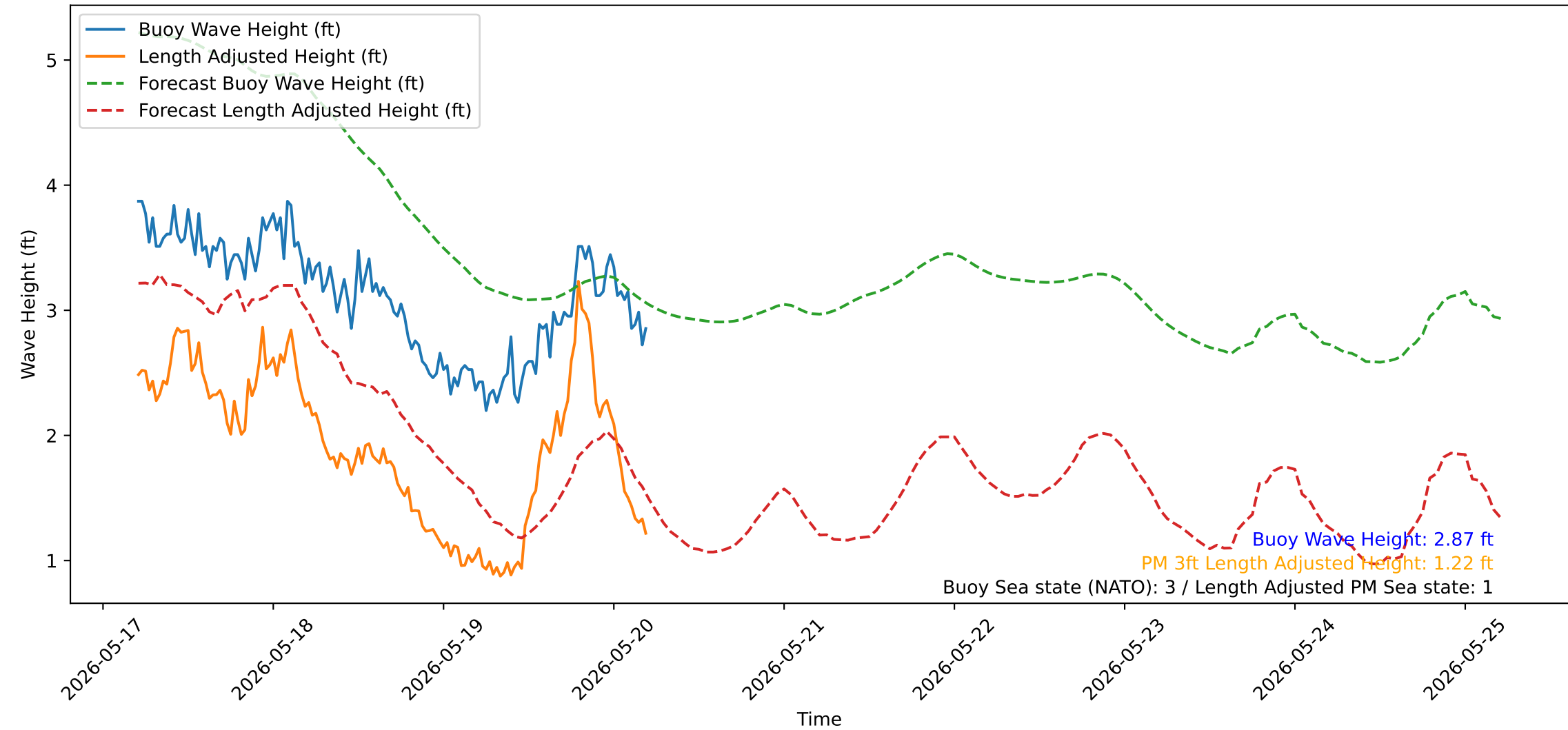
Wave Heights over Time for Oceanside Harbor at 2026-05-20 05:10:31
