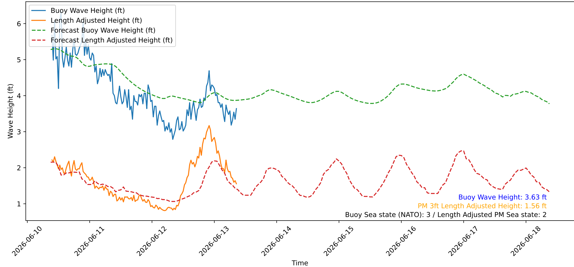
Wave Heights over Time for Oceanside Harbor at 2026-06-13 09:20:26
