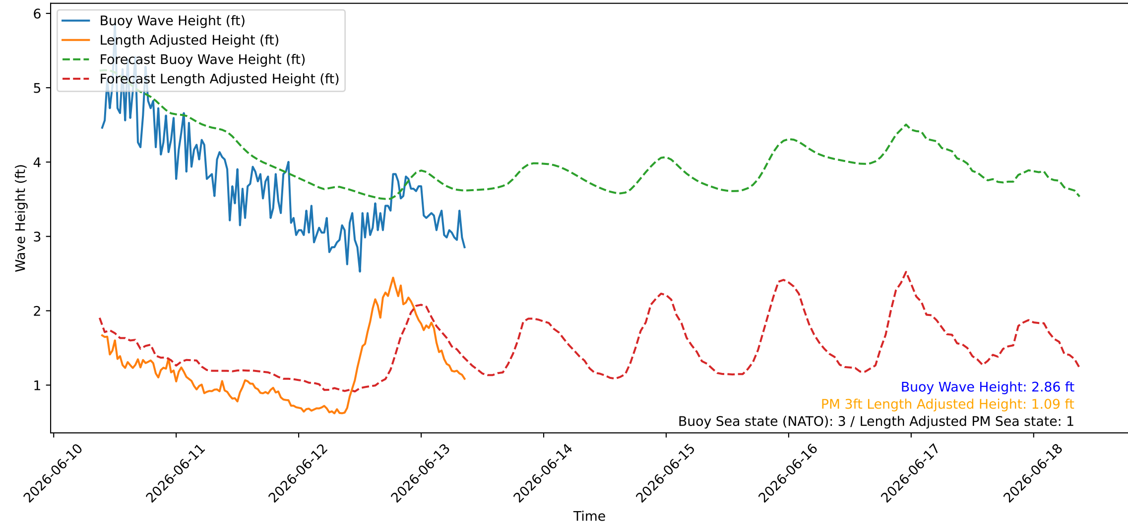
Wave Heights over Time for Red Beach at 2026-06-13 09:20:47
