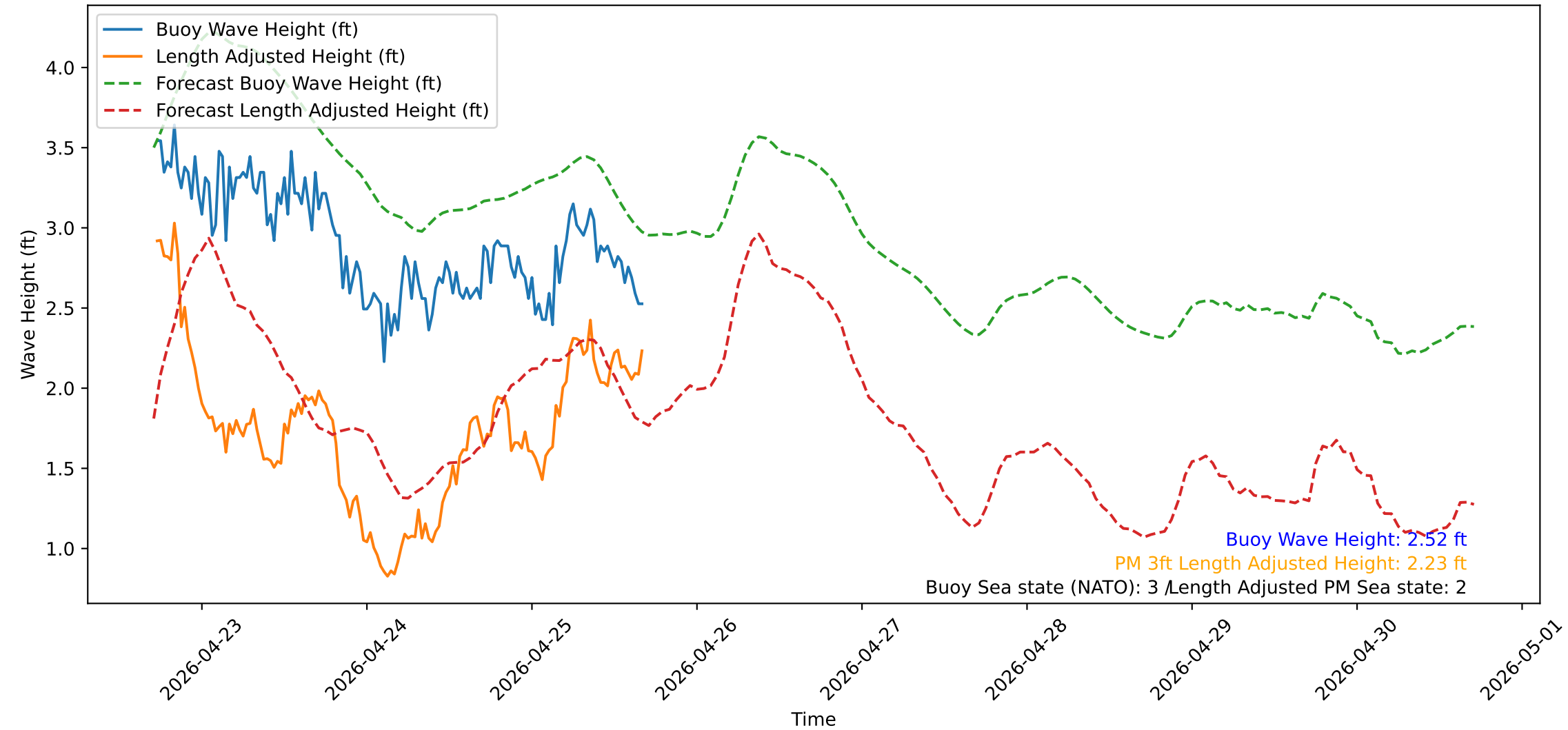
Wave Heights over Time for Red Beach at 2026-04-25 17:00:51
