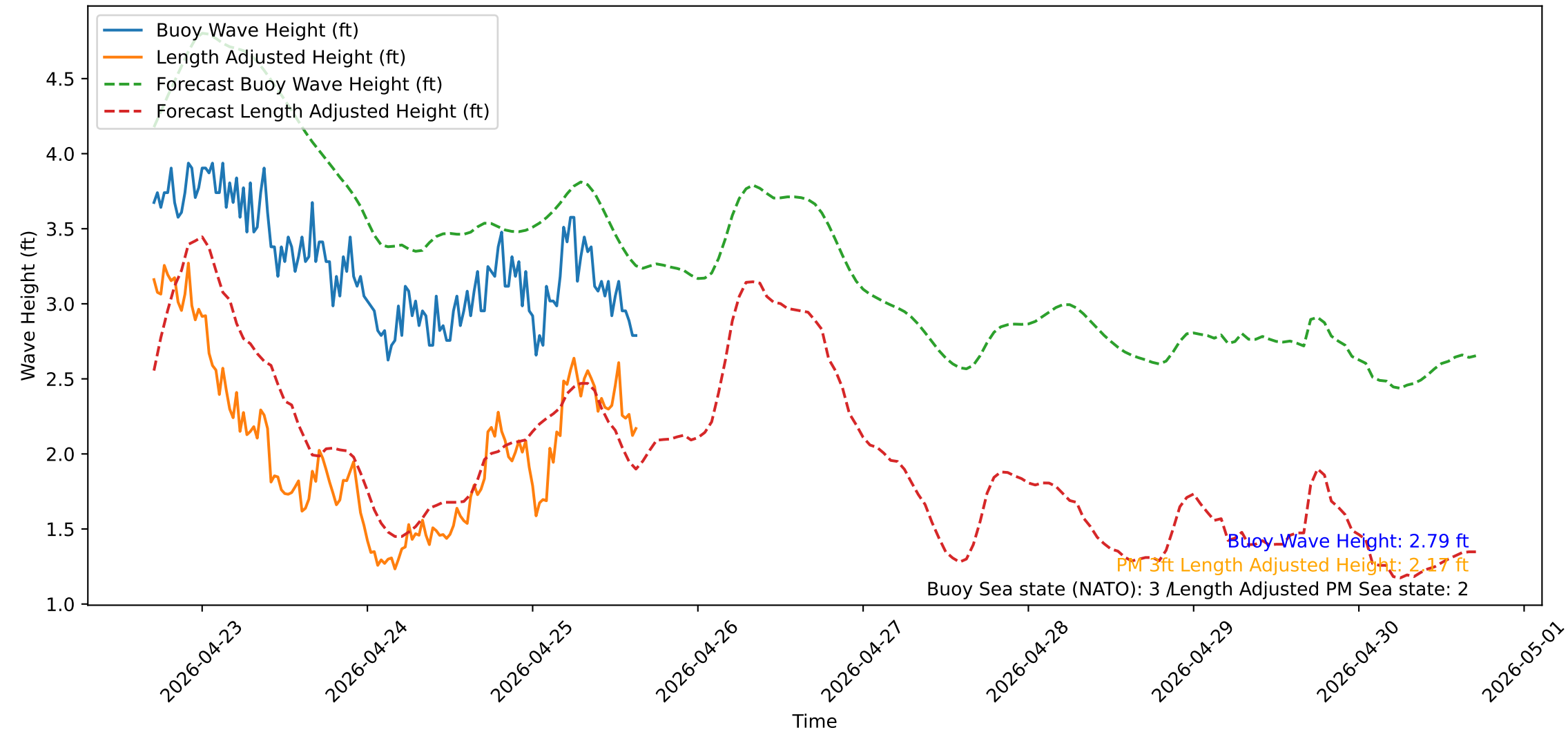
Wave Heights over Time for Green Beach at 2026-04-25 17:01:13
