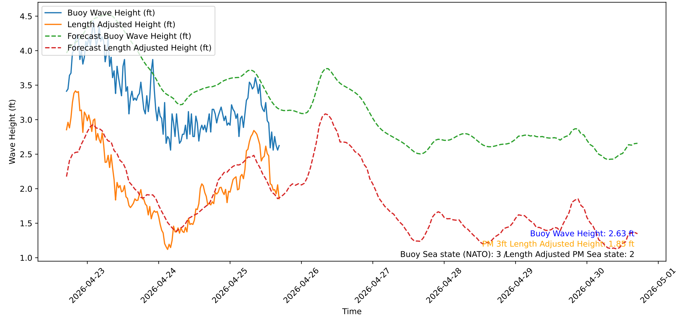
Wave Heights over Time for Oceanside Harbor at 2026-04-25 17:00:31
