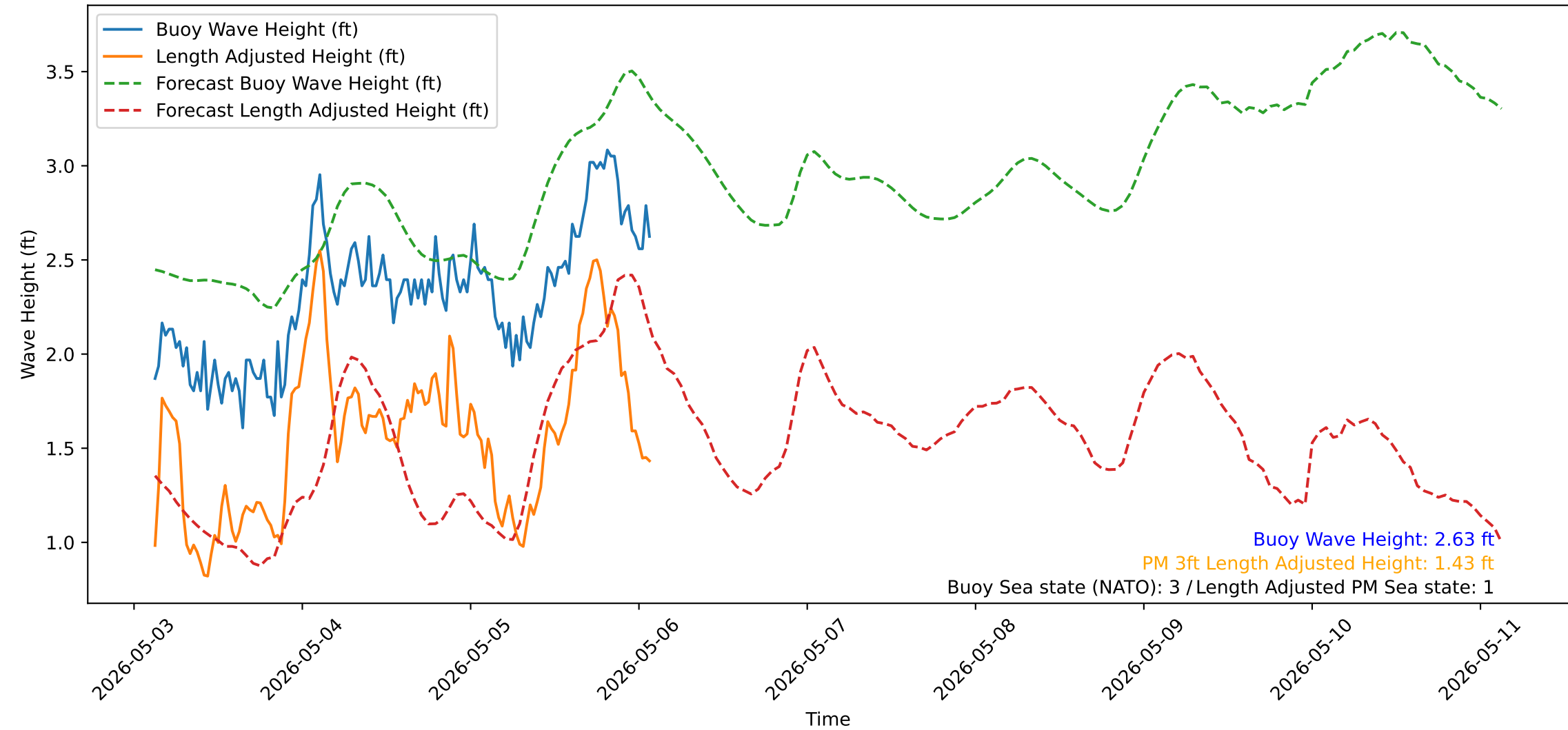
Wave Heights over Time for Red Beach at 2026-05-06 02:30:51
