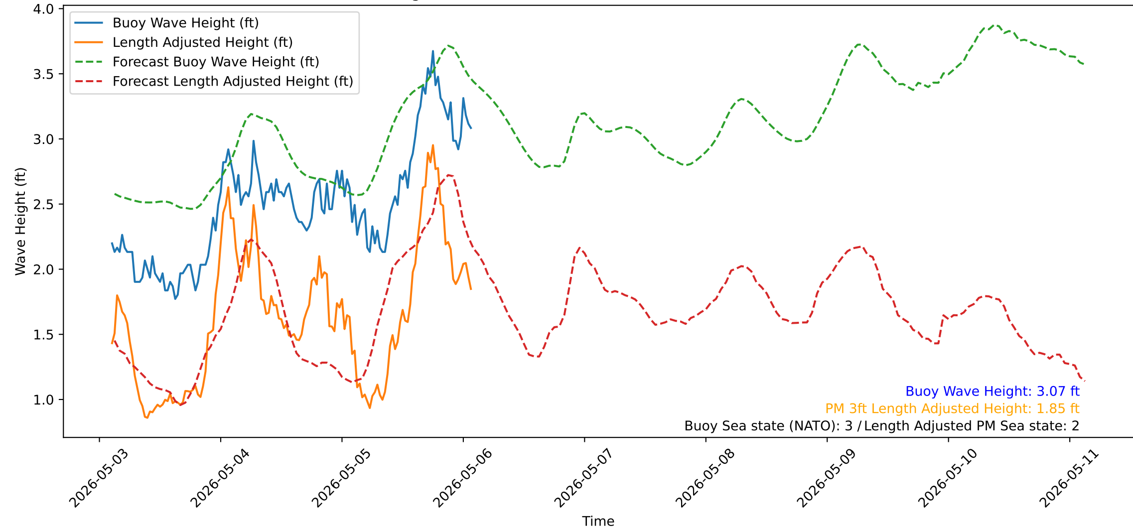
Wave Heights over Time for Green Beach at 2026-05-06 02:31:13
