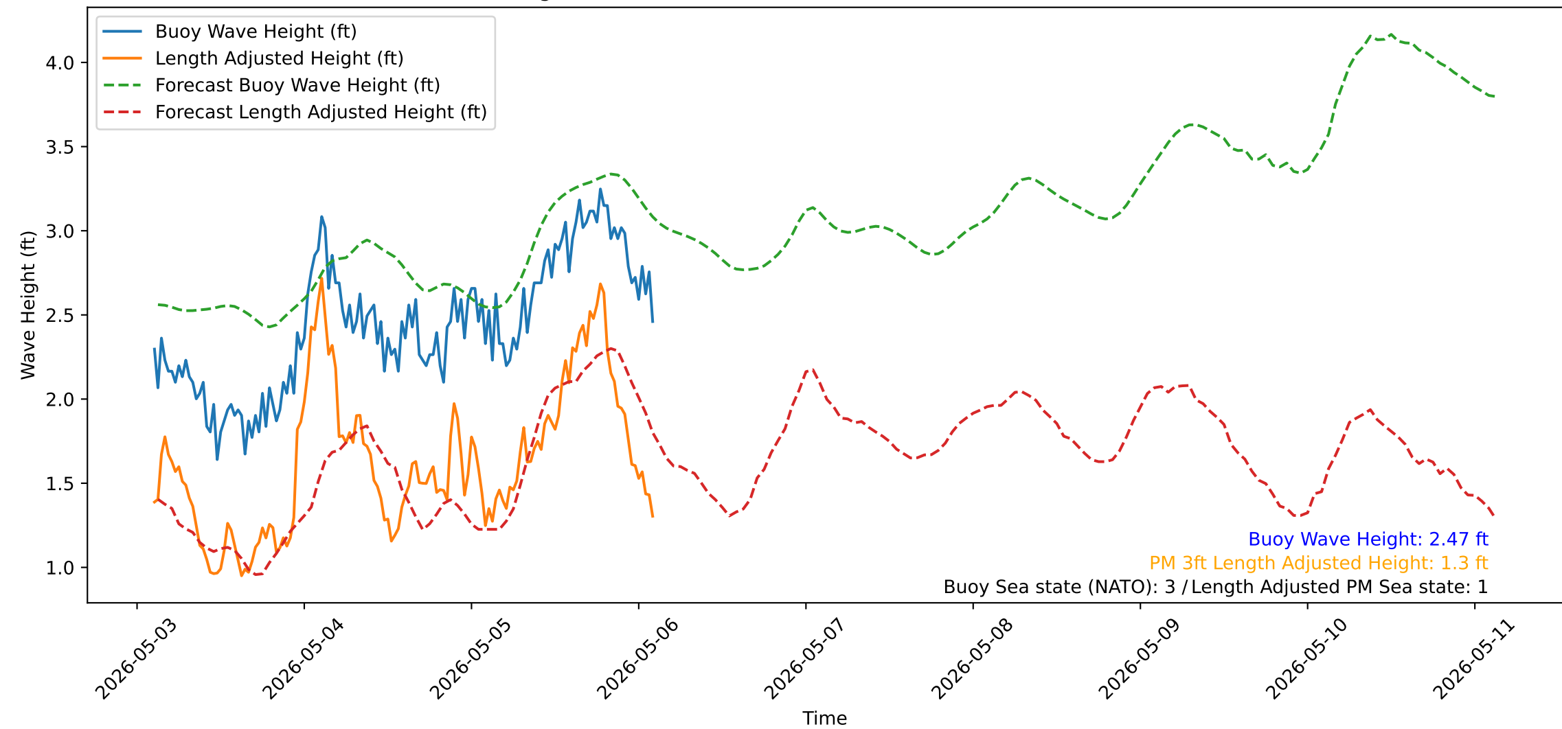
Wave Heights over Time for Oceanside Harbor at 2026-05-06 02:30:32
